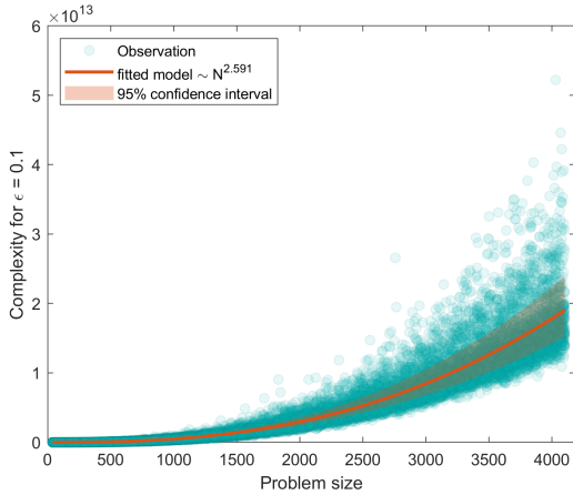
Figure 2.1: Observed complexity of Algorithm 1, its power law fit, and 95% confidence interval.
