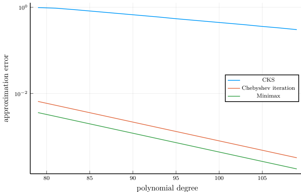
Figure 3.1: Approximation error for a fixed condition number \kappa = 10 and varying degrees.
