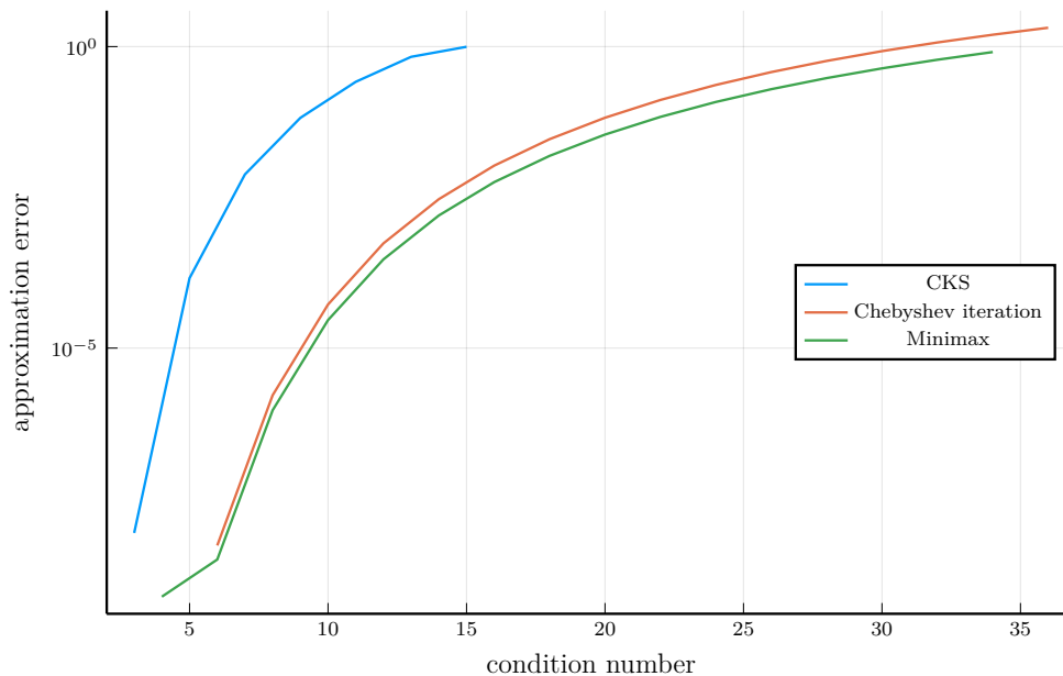
Figure 3.2: Approximation error for a fixed degree 2t - 1 = 127 and varying condition numbers.
