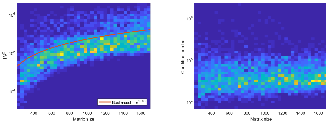
(a) Squared inverse tomography precision 1/\delta^2 for instances of (2.16) of different sizes. (b) Condition number \kappa for instances of (2.16) of different sizes.
