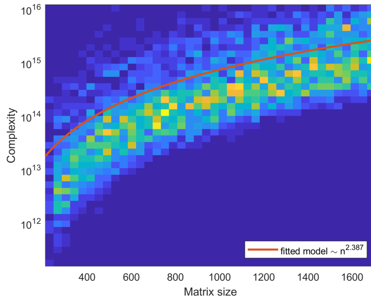
Figure 2.4: Observed complexities for \epsilon = 0.1 and the corresponding power-law fit. The x -axis is n , the size of the Newton system, and the y -axis is the observed complexity, as per Theorem 2.18.
