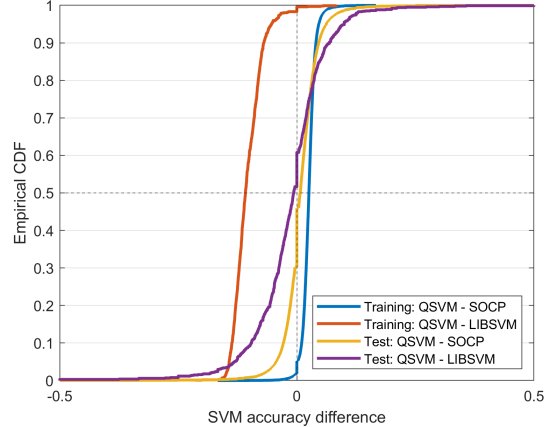
Figure 2.2: Empirical CDF of the difference in accuracy between SVMs trained in different ways.
