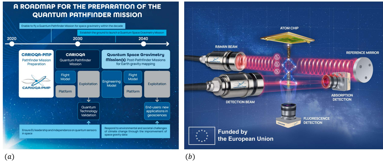
Figure 17: CARIOQA pathfinder mission preparation program - (a) Roadmap for the preparation of quantum gravimetry mission by European Union (extracted from CARIOQA PMP presentation poster ) (b) Artistic view of the atom accelerometer principle ( CARIOQA website )
