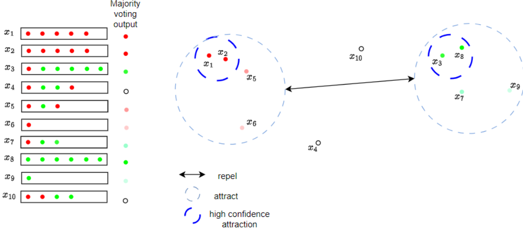
Figure 4.12: Exams such that c(\mathbf{y}_i) = 0 (no decision from majority vote) are considered as unlabeled and uncolored. Exams such that c(\mathbf{y}_{i,j}) = 1 and y_i = y_j , e.g. (x_1, x_2) (resp. (x_3, x_8) ), will be strongly attracted while less attracted to patients with c(\mathbf{y}_i) < 1 , e.g. x_{5,6} (resp. x_{7,9} ). Groups of exams with different y scores are repelled.
