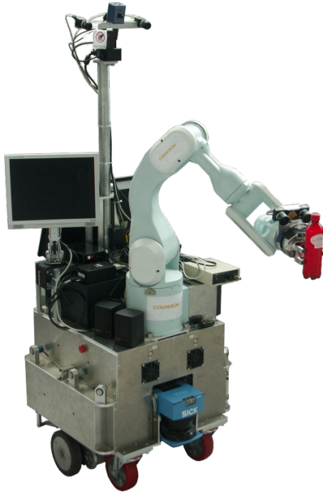
Figure 3.17: The mobile robot Jido which is used in the experiment for taking the required photos.
