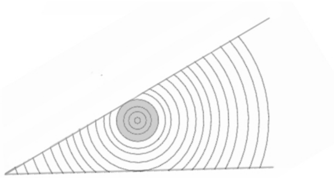
Figure 2.7: The integral is computed over a ball included in the cone defining non-collision.
