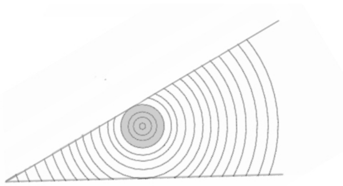
Figure 2.7: The integral is computed over a ball included in the cone defining non-collision.
