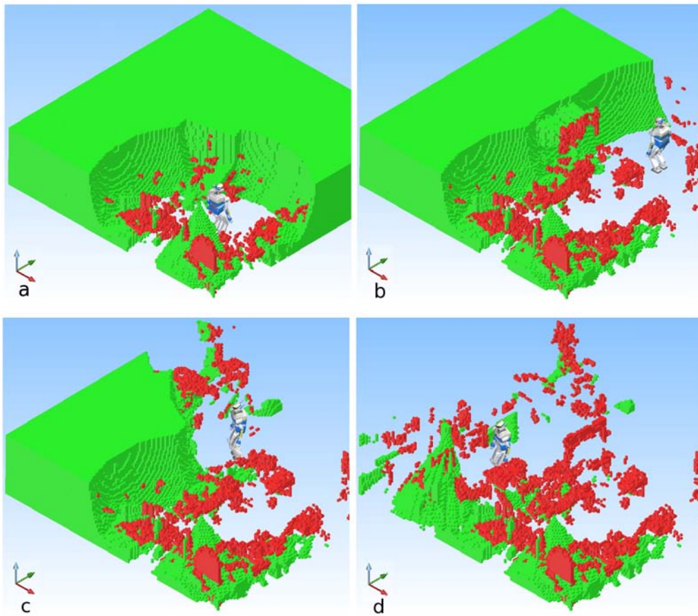
Figure 5.3: Exploring an unknown environment. Red and green voxels represent occupied and unknown zones in the model. The robot plans a path in free zone.
