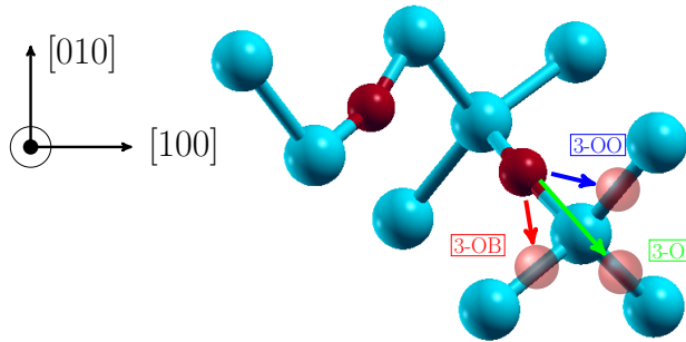
Figure 3.21: Dissociation scheme of O_{2i} from 2-O to 3-OO, 3-OF and 3-OB configurations.
