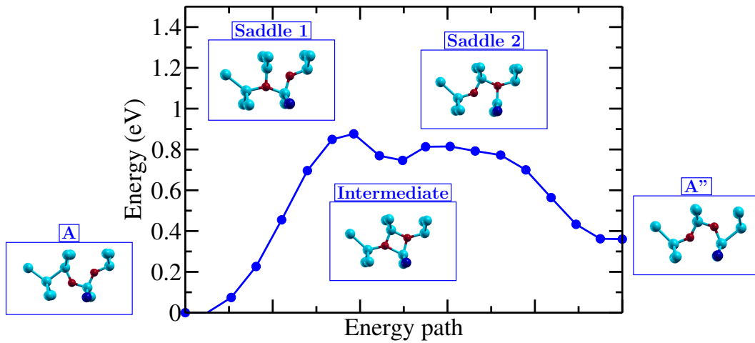
Figure 3.35: NEB calculations of B_s O_{2i} dissociation with O_{2i} going away from B atom.
