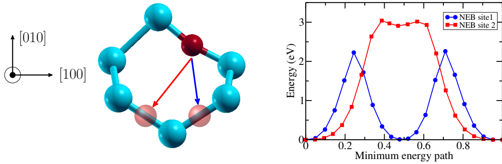
Figure 3.12: Other O_i migration paths.
