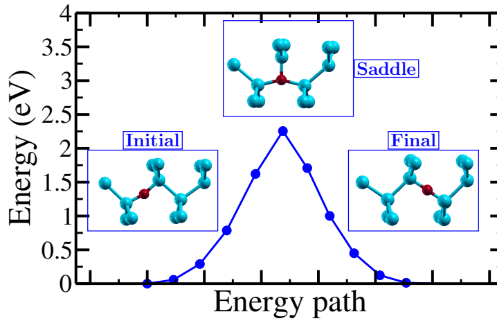
Figure 3.10: O_i migration path calculated with NEB method. Initial, final and saddle configurations are represented on the Figure.
