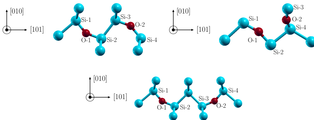
Figure 3.28: Atomic configurations for 2-O and 2-P structures in a (101) plane and in the orthogonal plane.
