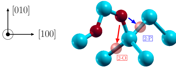
Figure 3.20: Dissociation from O_{2i} to 2-O and 2-P configurations.
