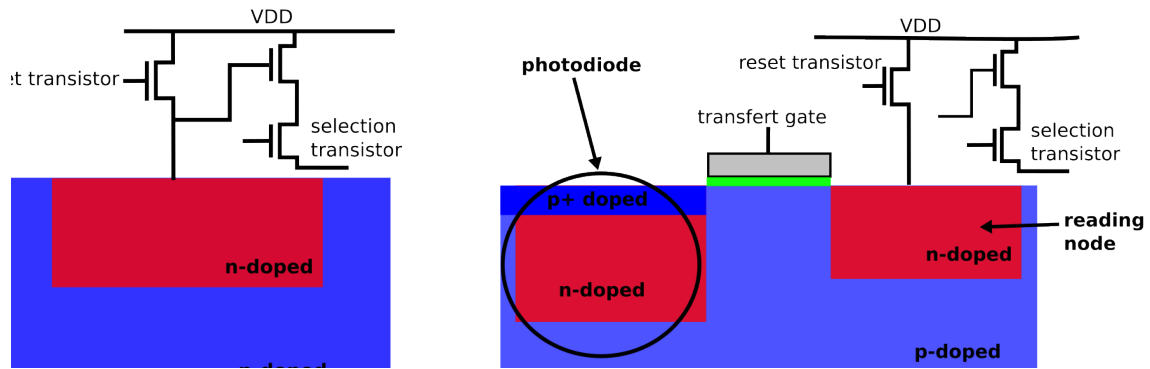
Figure 1.6: (Left) Architecture of a pixel with a photodiode of type 3T - (Right) architecture of a pixel with a photodiode of type 4T.
