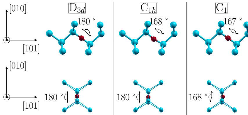
Figure 3.1: Different O_i configurations relaxed with ab initio calculations, from left to right: D_{3d} , C_{1h} and C_1 . The configurations are represented in a (101) plane (top) and in its orthogonal plane (10\bar{1}) (bottom).
