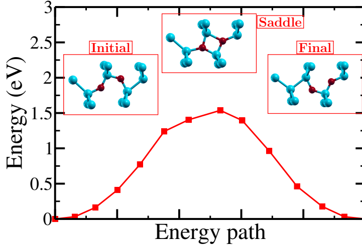
Figure 3.14: O_{2i} migration path determined with NEB method for PBE calculations.
