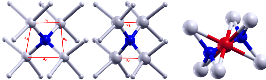
Figure 1.10: Different vacancies configurations. Blue balls indicate a missing atom and red balls an additional atom. From left to right : V_{Td}^{2+} , V_{D2d}^0 and V_{Cs}^{-2} vacancy configurations (pictures from M3 Team in LAAS-CNRS, not published)
