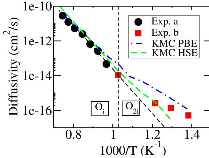
Figure 3.18: Diffusivity of oxygen obtained with KMC using the activation energies calculated with ab initio calculations using PBE and HSE functionals.
