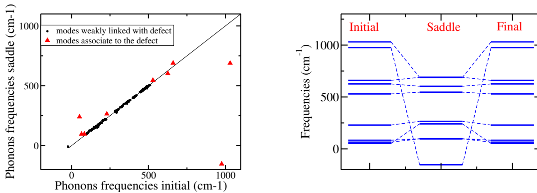
Figure 3.31: Phonons frequencies in the O 2i staggered and in the O 2i migration saddle points.
