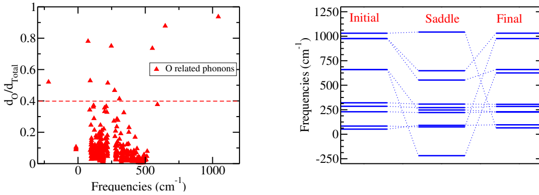
Figure 3.33: (Left) Part of oxygen displacement in the phonons of \text{O}_{2i} to 2-O saddle point. (Right) Projection of the phonons related to oxygen (upon the dotted red line in the left figure) on the phonons of \text{O}_{2i} and 2-O.
