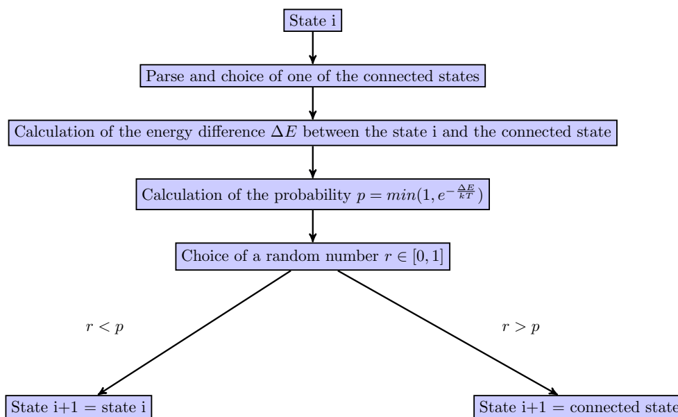
Figure 2.3: Metropolis scheme from [5].
