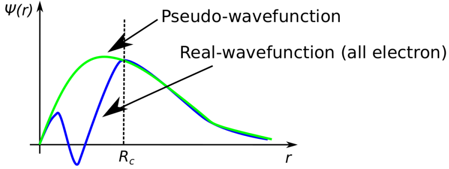
Figure 2.6: Illustration of the pseudopotential concept from [14].
