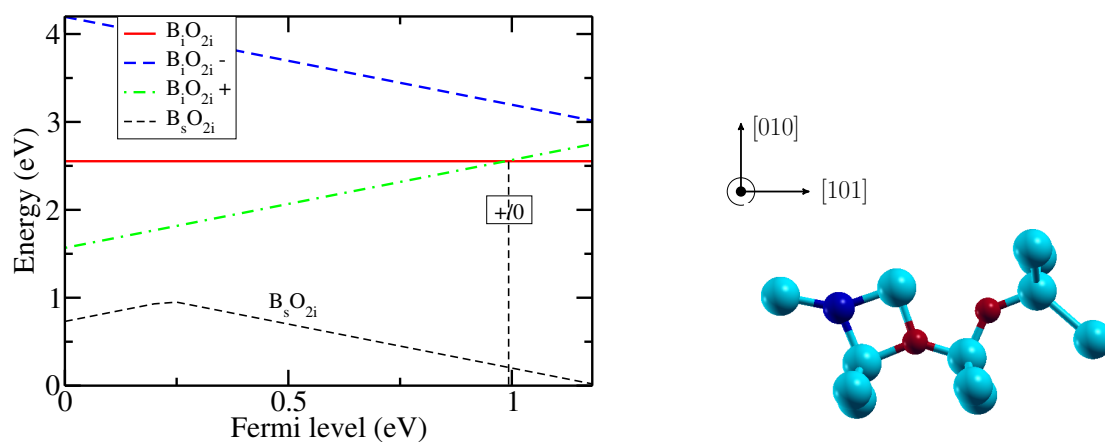
Figure 3.8: B_iO_{2i} formation energy compared to B_sO_{2i} formation energy calculated with HSE.
