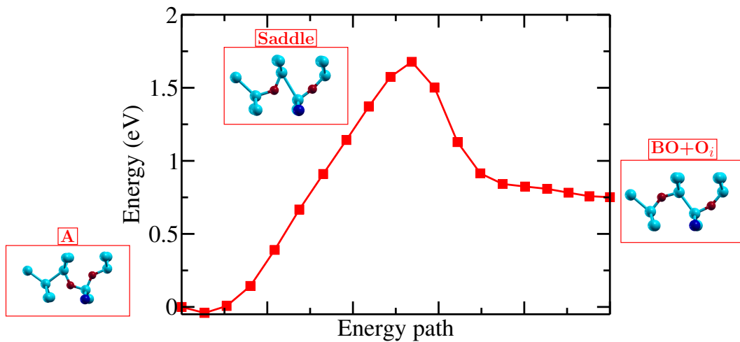
Figure 3.36: NEB calculations of B_s O_{2i} dissociation with O_i going away from BO_i complex.
