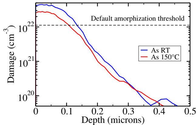
Figure 4.19: Damage predicted in continuum simulations after As implantations at RT and 150 °C.
