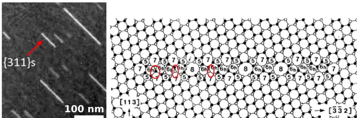
Figure 1.13: (Left) TEM images of 311 defects from [17] (Right) Atomic structure of defects 311 from [18].
