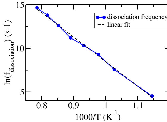
Figure 3.38: Logarithm of the dissociation frequency in the off-lattice KMC depending on the temperature using an intermediate points in the \text{O}_{2i} dissociation path (averaged on 20 simulations).
