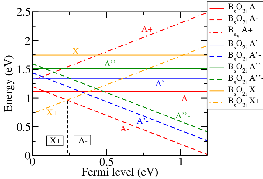
Figure 3.6: B_s O_i formation energies for the different configurations ( A, A', A'' and X ) calculated using HSE formalism.
