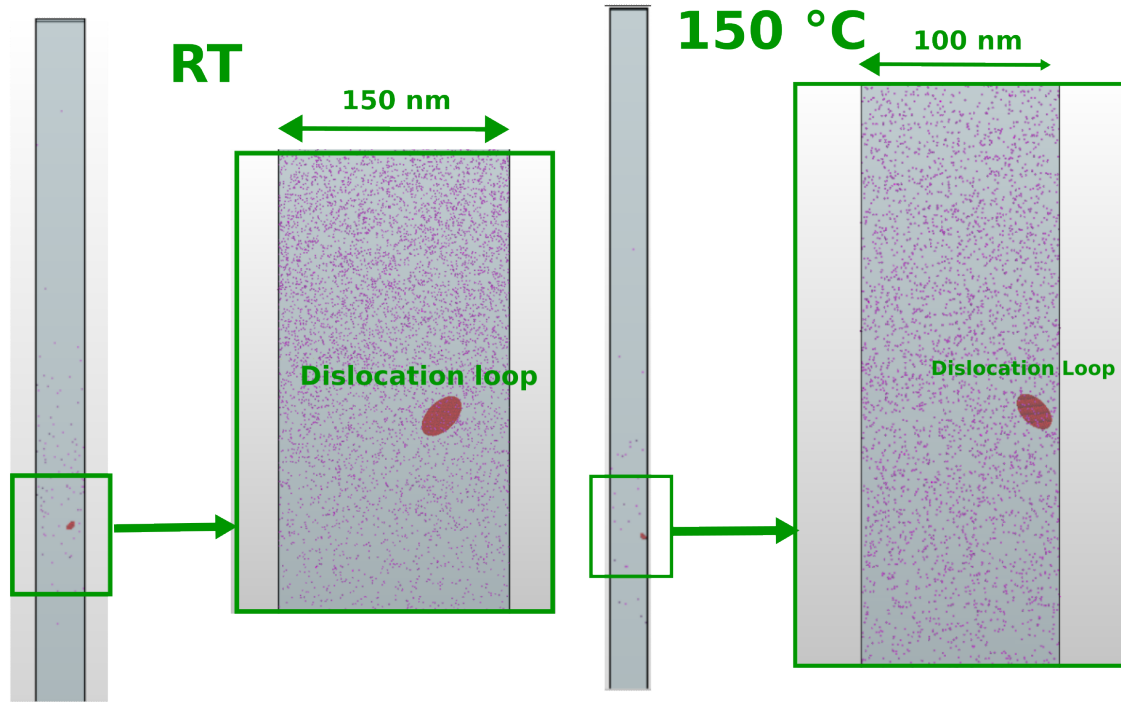
Figure 4.9: KMC simulations of phosphorus implantation at RT and 150°C with a dose of 6 \times 10^{13} \text{ cm}^{-2} and followed by annealing described Table 4.2. The red circles represent the DLs.
