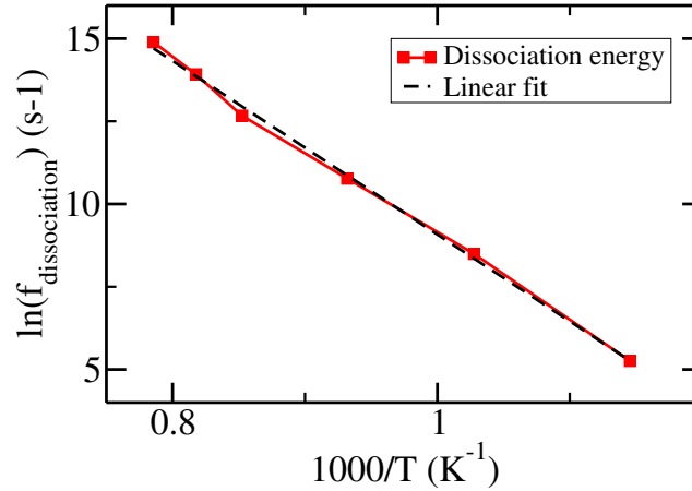
Figure 3.37: Logarithm of the dissociation frequency in the Off-Lattice KMC depending on the temperature with the barriers implemented until the 4th neighbors (averaged on 20 simulations).
