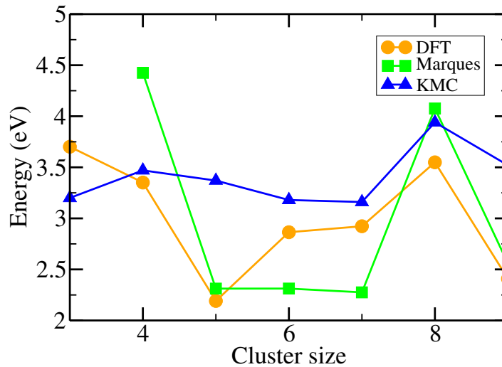
Figure 4.32: Comparison of the activation energies for the emission of an interstitial from a SMICs between the values implemented in the KMC, the values extracted using the formula 4.4 with the formation energies of [22] and those calculated in DFT.
