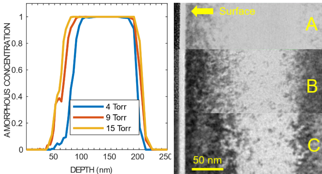
Figure 4.3: (Left) Simulation of amorphous concentration as function of the depth for a 60 keV carbon implantation with a dose of 1.5 \times 10^{15} \text{ cm}^{-2} and for cooling pressures of 15, 9 and 4 Torr. (Right) A, B and C are the TEM images of 60 keV carbon implanted wafers with a dose of 1.5 \times 10^{15} \text{ cm}^{-2} and a cooling pressure of 15, 9 and 4 Torr respectively.
