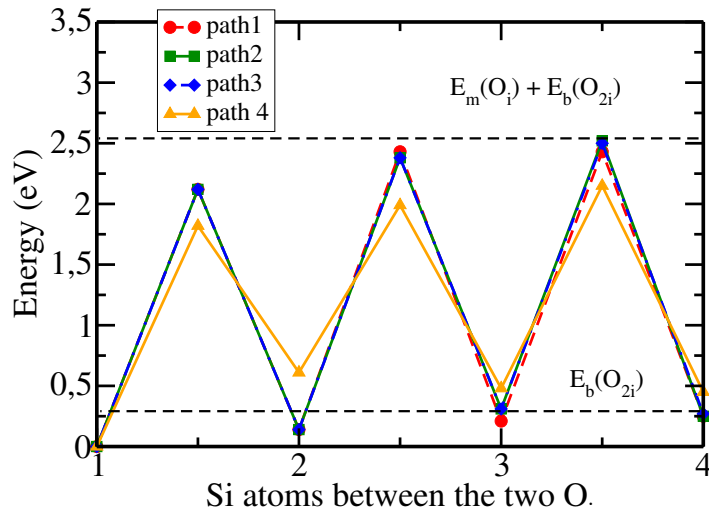
Figure 3.23: \text{O}_{2i} dissociation energies for saddle structures and intermediate stable structures calculated with ARTn. Path 1, 2, 3 start with the \text{O}_{2i} \rightarrow 2\text{O} . Path 4 is 2P \rightarrow 3PP \rightarrow 4PPP .
