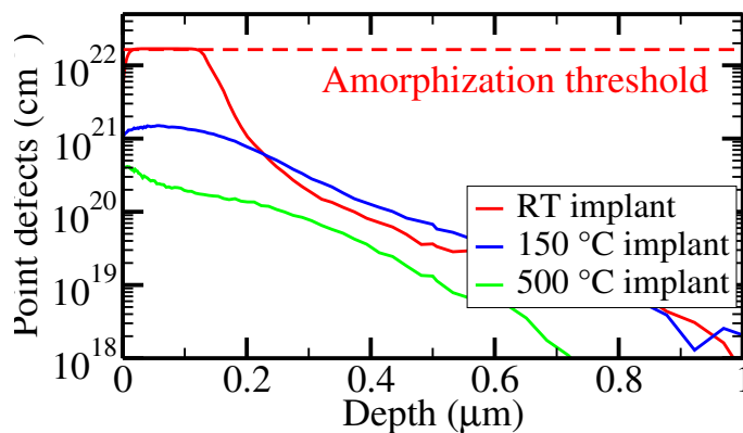
Figure 4.21: KMC prediction for the concentration of points defects as-implanted in the RT, 150 °C and 500 °C cases.
