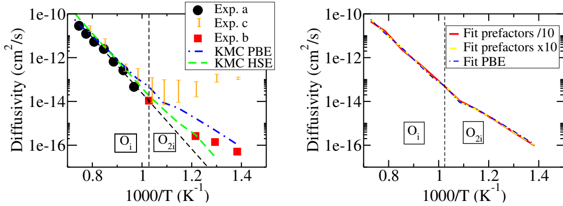
Figure 3.19: (Left) O_{2i} diffusion calibrated and compared to other experimental data [42] and [34] (Right) Predict oxygen diffusion in KMC using a same ratio with different values for \nu_{dis}(O_{2i}) and \nu_m(O_{2i}) .
