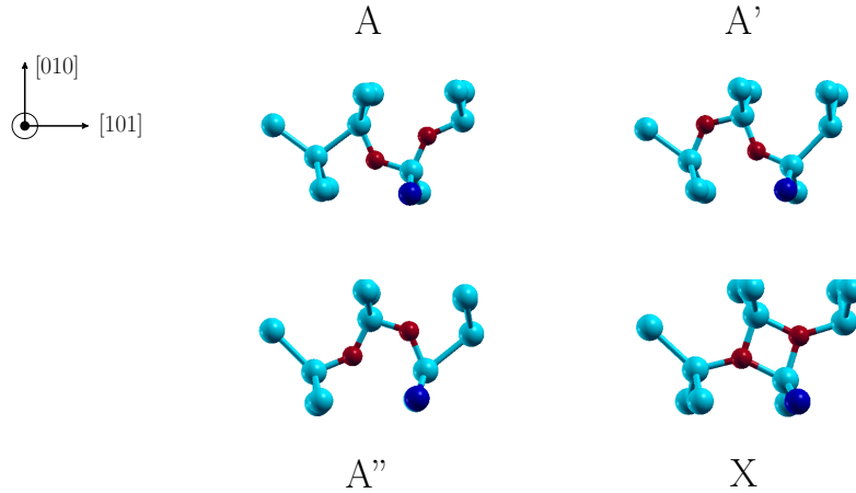
Figure 3.5: \text{BO}_{2i} configurations A, A', A'' and X represented in the same (101) plane.
