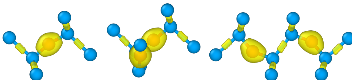
Figure 3.29: Iso-surface of the O i charge density (Left), 2-O charge density (Middle) and 2-P charge density (Right). All views are in the (101) plane.
