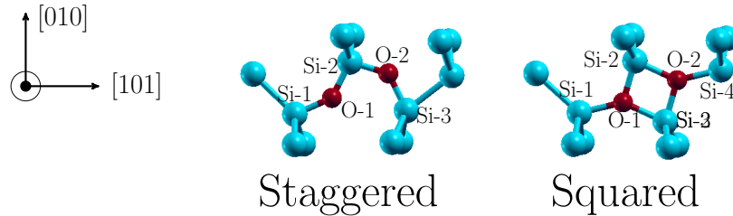
Figure 3.3: O_{2i} configurations: staggered (left) and squared (right) in a (101) plane from ab initio simulations.
