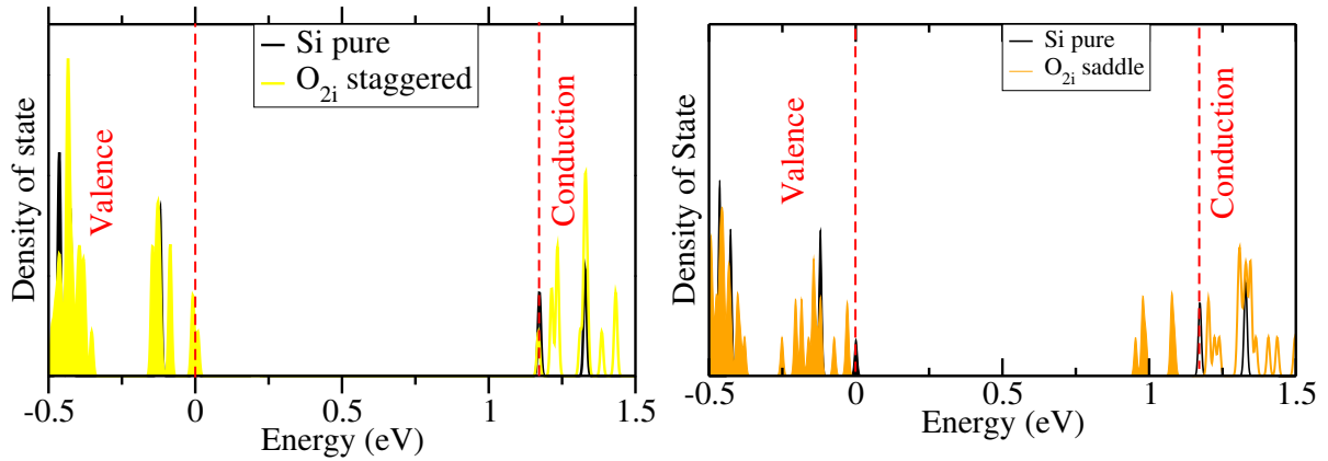
Figure 3.15: DOS for O_{2i} stable structure and migration saddle point structure.
