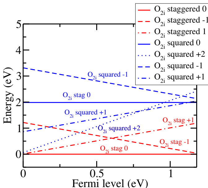
Figure 3.4: \text{O}_{2i} formation energies calculated using HSE formalism in neutral, +1 and +2 charge states for squared configuration and in neutral, -1 and +1 charge states in staggered configurations.
