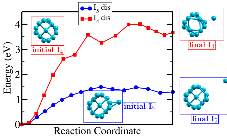
Figure 4.33: Emission paths to emit one I from I_4 (red curve) and I_5 (blue curve) of compact type into respectively I_3 and I_4 .
