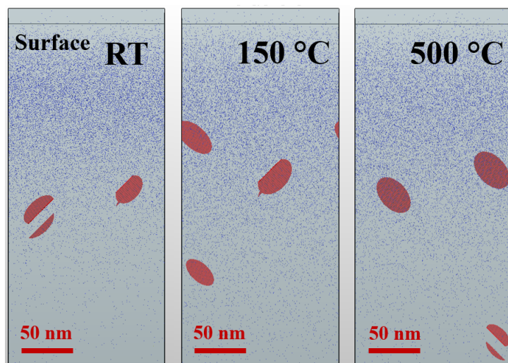
Figure 4.22: Simulation of the 3 implantations followed by annealing (left RT, middle 150°C and right 500°C) using the default KMC model. The red loops correspond to the dislocation loops.
