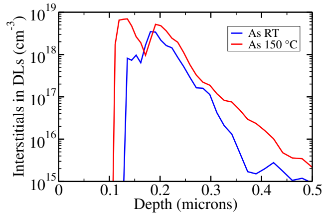
Figure 4.20: Continuum prediction for interstitials concentration in DLs after the annealing sequence following the RT and 150 °C implantations.
