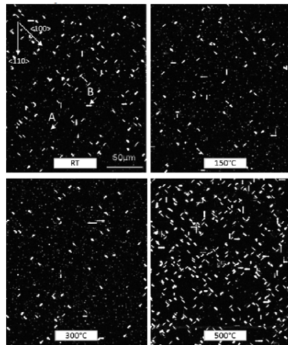
Figure 1.20: Photoluminescence imaging of wafers implanted at different temperatures (RT, 150^{\circ}\text{C} , 300^{\circ}\text{C} and 500^{\circ}\text{C} ) then annealed at 950^{\circ}\text{C} for 3 minutes from . Extended defects are visible in white on the images.
