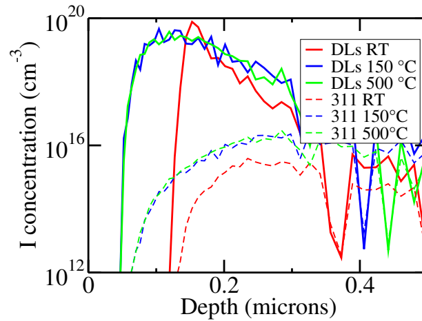
Figure 4.23: Interstitial concentration in DLs and in \{311\} in KMC-continuum.
