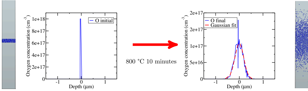
Figure 3.17: Methodology to extract the diffusivity from KMC simulations.
