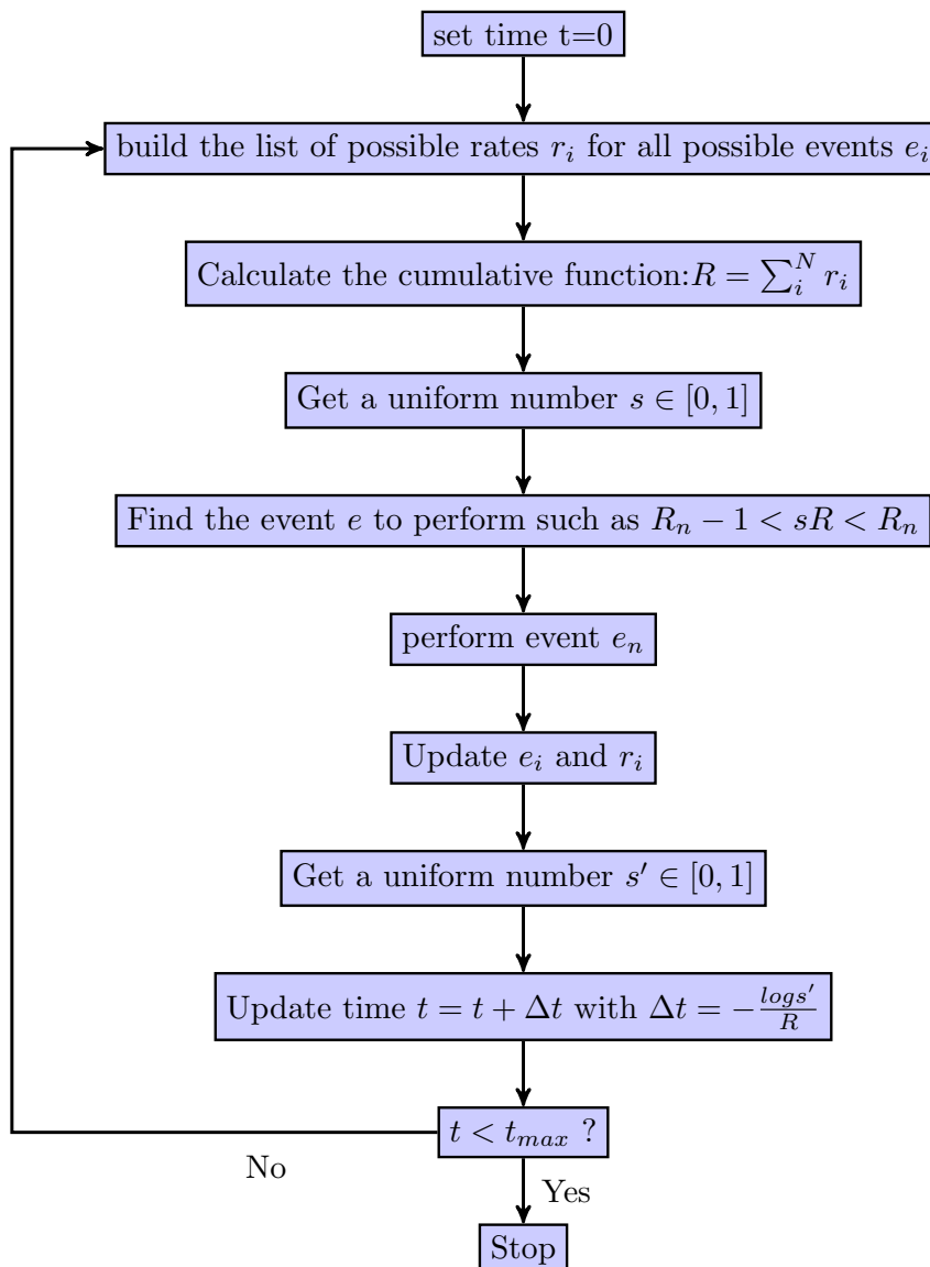
Figure 2.4: KMC scheme from [5].
