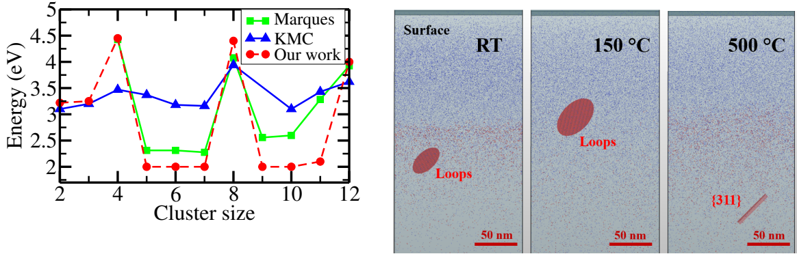
Figure 4.28: (Left) Activation energies for interstitial emission depending on the SMICs size (Right) Resulting defects formed after the annealing in the 3 cases (implantations at RT, 150°C and 500°C).
