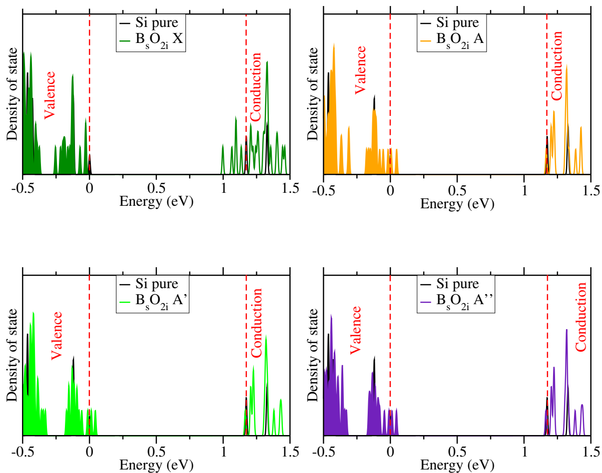
Figure 3.7: DOS of the different configurations A , A' , A'' and X for neutral charge state calculated with HSE.
