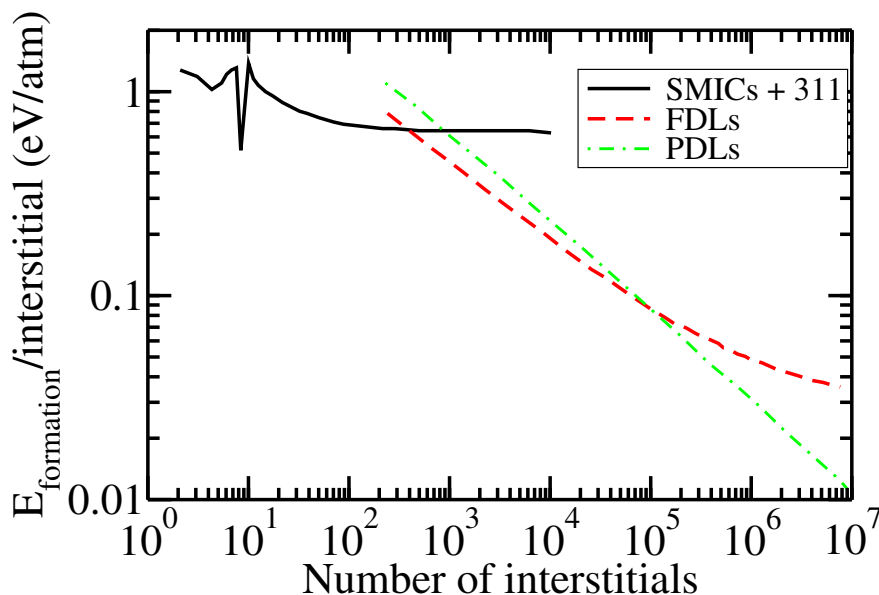
Figure 1.16: Interstitial formation energies for different types of defects as a function of the number of interstitials in the defect [35][36][24]
