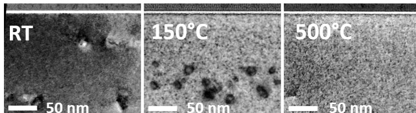
Figure 4.11: Cross section TEM micrographs taken from samples implanted with As (cf. Table 4.4 for implant details) and annealed according to Table 4.5. The As implants were carried out at different temperatures: room temperature (left), 150°C (center) and 500°C (right).
