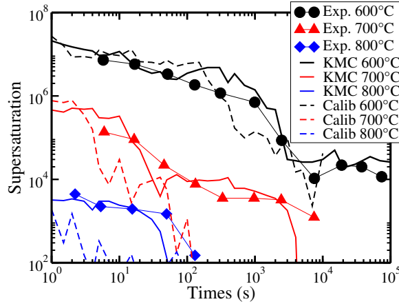
Figure 4.29: Comparison of supersaturation extracted from [25] experiments (exp in the legend) and predicted by the KMC using the default implementation (KMC in the legend) and the calibrated energies on the As implementations (calib in the legend).
