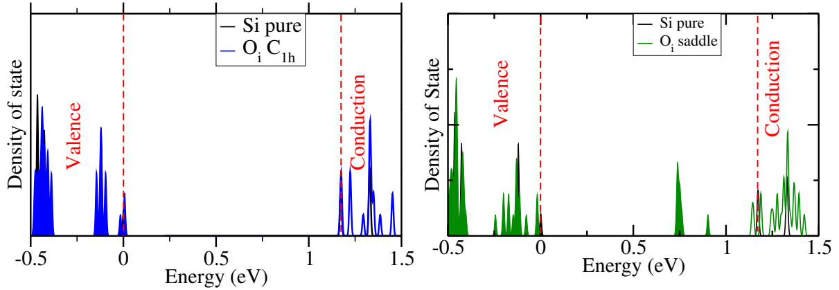
Figure 3.11: DOS of O_i migration stable and saddle structure calculated using HSE formalism.
