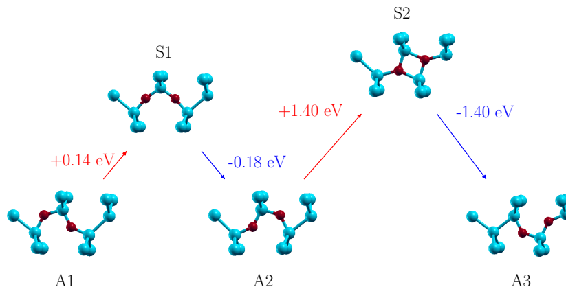
Figure 3.13: O_{2i} migration path between two staggered configurations. Activation barriers are given in eV obtained for PBE calculations.
