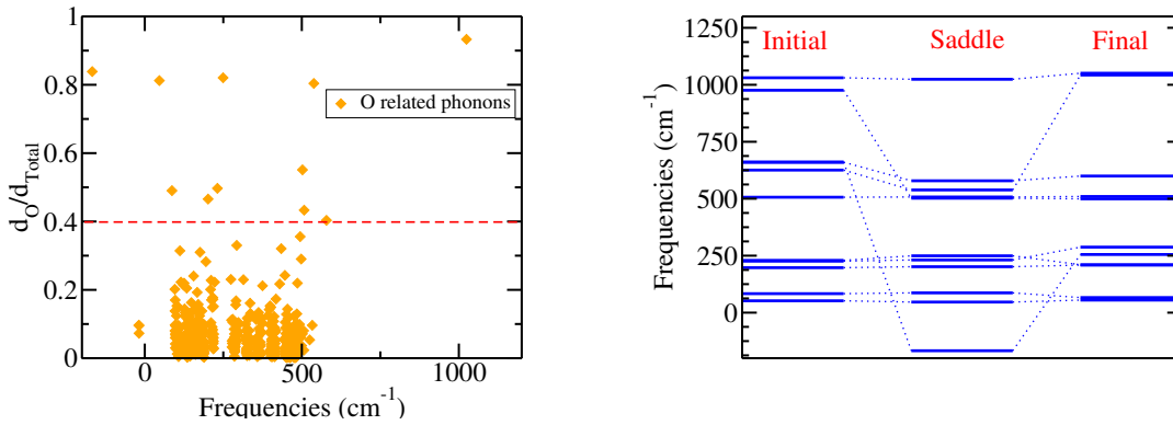
Figure 3.32: (Left) Part of oxygen displacement in the phonons of O 2i to 2-P saddle point. (Right) Projection of the phonons related to oxygen (upon the dotted red line in the left figure) on the phonons of O 2i and 2-P.
