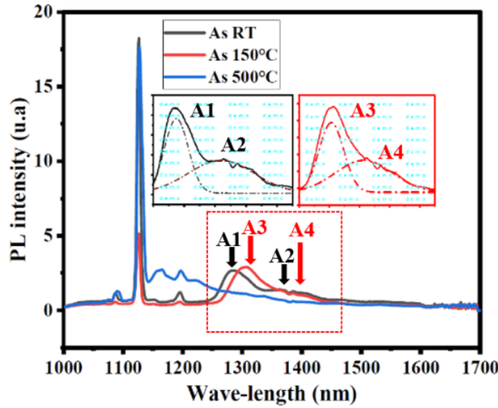
Figure 4.14: PL spectra taken at a temperature of 8K from samples implanted with As (cf. Table 4.4 for implant details) and annealed according to Table 4.5. The As implants were carried out at different temperatures: room temperature, 150°C and 500°C.
