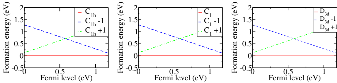
Figure 3.2: O_i formation energies in C_1 , C_{1h} and D_{3d} configurations in charge state -1, 0 and +1 calculated with HSE.
