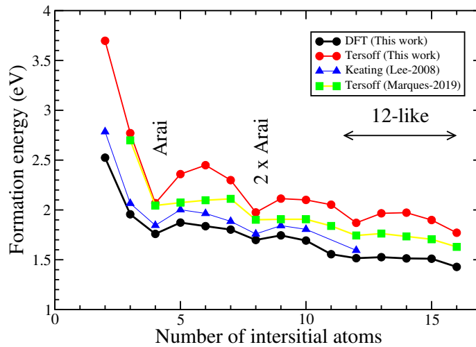
Figure 4.31: Comparison of the interstitial formation energies of SMICs from [22] and [23] works and the energies calculated in this thesis using the coupled MD - DFT strategy.
