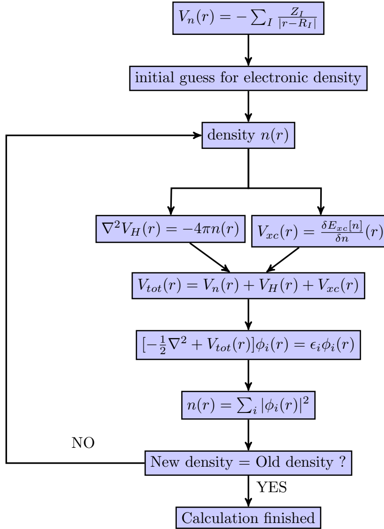
Figure 2.5: Kohn-Sham scheme from [18].
