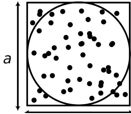
Figure 2.1: Scheme of a Monte Carlo method to find the value of \pi .
