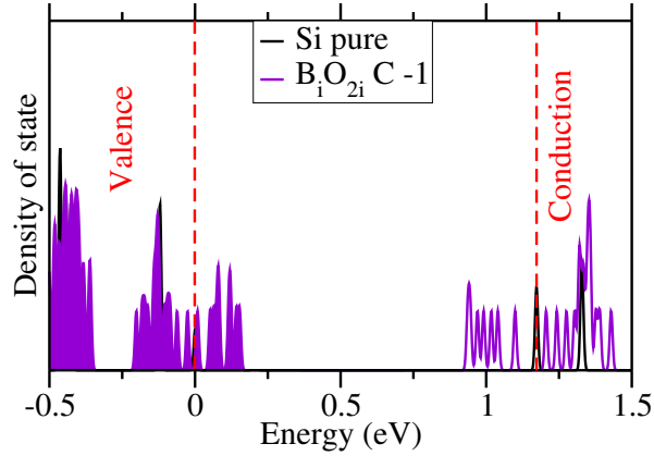
Figure 3.9: DOS of B_iO_{2i} C configuration calculated with HSE.
