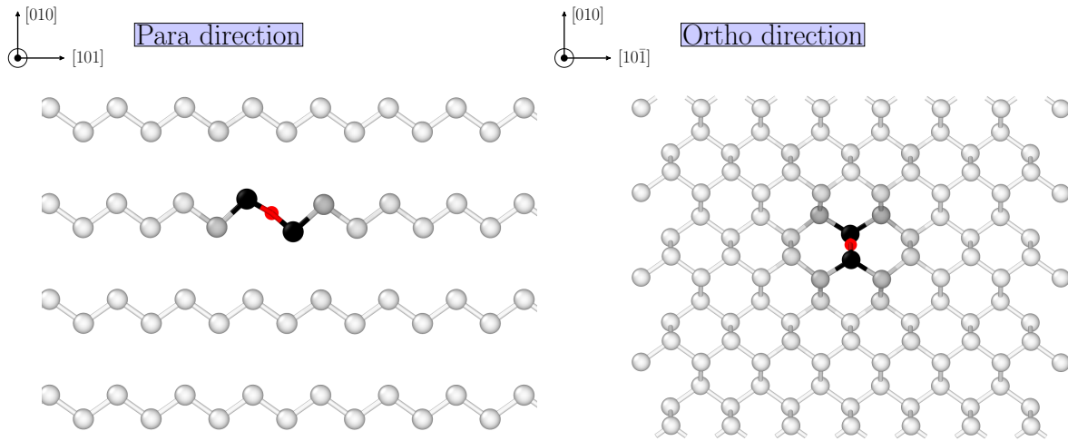
Figure 3.27: Displacements of Si atoms in a O_i supercell compared to their positions in a pure Si cell calculated using IRA [43].
