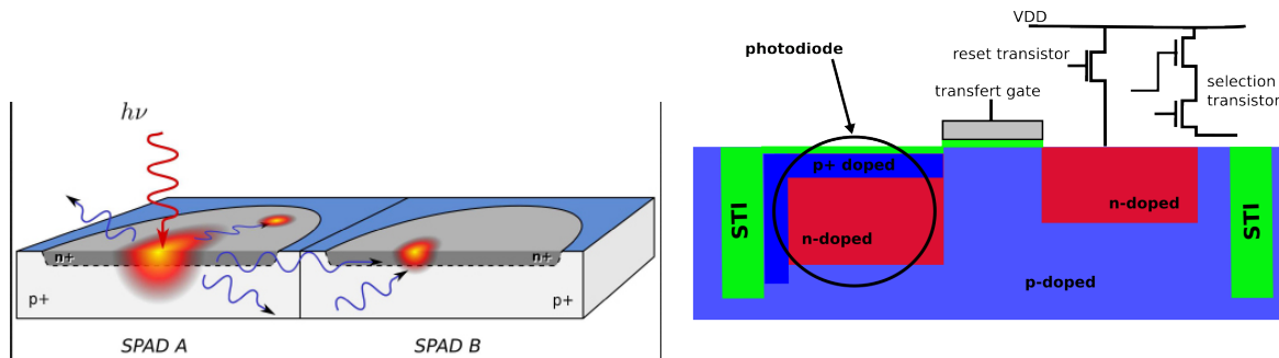
Figure 1.8: (Left) Cross-talk between 2 pixels from [3] - (Right) Scheme of a 4T photodiode with STI to avoid cross-talk phenomena.
