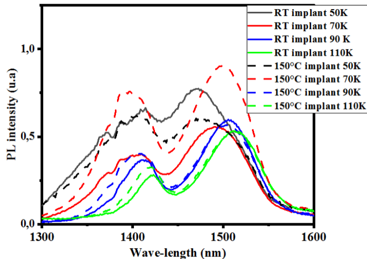
Figure 4.8: PL spectra acquired at different temperatures from samples Ph2 and Ph3 (cf. Table 4.2) implanted with P at different temperatures (RT and 150°C respectively).
