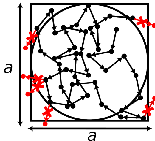
Figure 2.2: Scheme of a Monte Carlo method to find the value of \pi .
