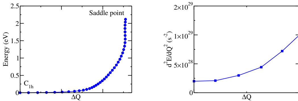
Figure 3.34: (Left) Energy along the dissociation path as function of the displacement vector Q . (Right) Second derivative of the energy along the dissociation path against the displacement vector Q .
