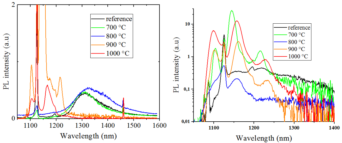
Figure 4.17: Photoluminescence spectra after additional annealing for the wafer initially implanted at 150 °C (Left) and 500 °C (Right).
