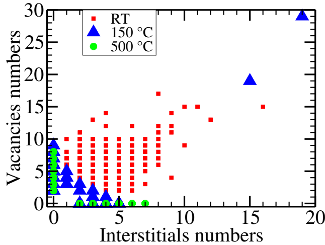
Figure 4.26: Histogram of I and V clusters for implantation at RT and heated implantation at 150 °C and 500 °C.
