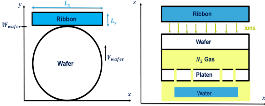
Figure 4.1: Schematics of the implanter end-station used in this work (left) and of its cooling system (right).
