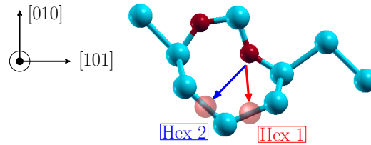
Figure 3.30: O 2i reorientation alternative paths.
