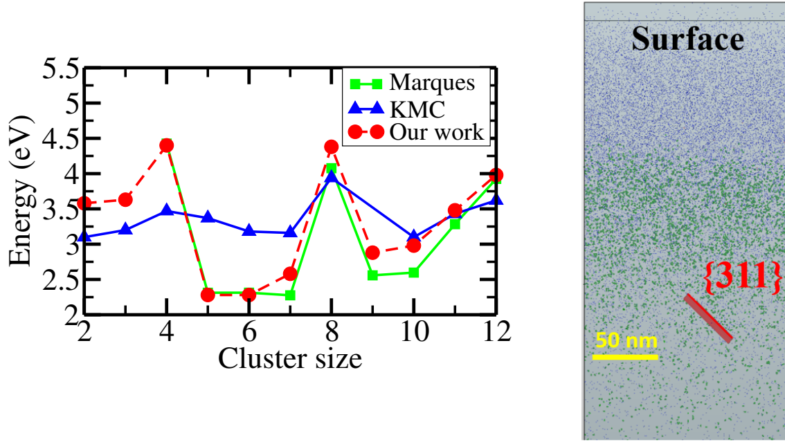
Figure 4.27: (Left) Activation energies for interstitial emission depending on the SMICs size (Right) Predicted \{311\} in KMC using the calibration presented on the left.
