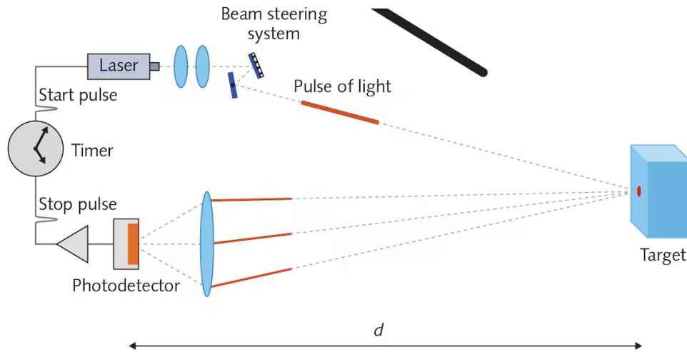
Figure 1.3: Operating scheme of a SPAD for a TOF application.
