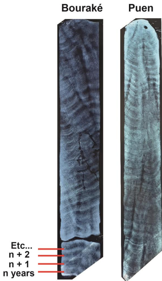
Figure VIII-18 | Positive X-radiographs of the two coral cores (Bouraké B2 and Puen R1) in New Caledonia. The model-age follows the density bands of the skeleton (red lines).
