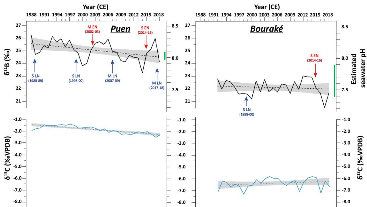
Figure VI-1 | Temporal evolution of \delta^{11}\text{B} (black) and \delta^{13}\text{C} (blue) signatures in Porites sp. cores collected at Puen (left) and Bouraké (right), over 31 and 27 years, respectively. The estimated seawater pH corresponding to the \delta^{11}\text{B} signatures is plotted on the second y-axis (right side of the graphs). The range
