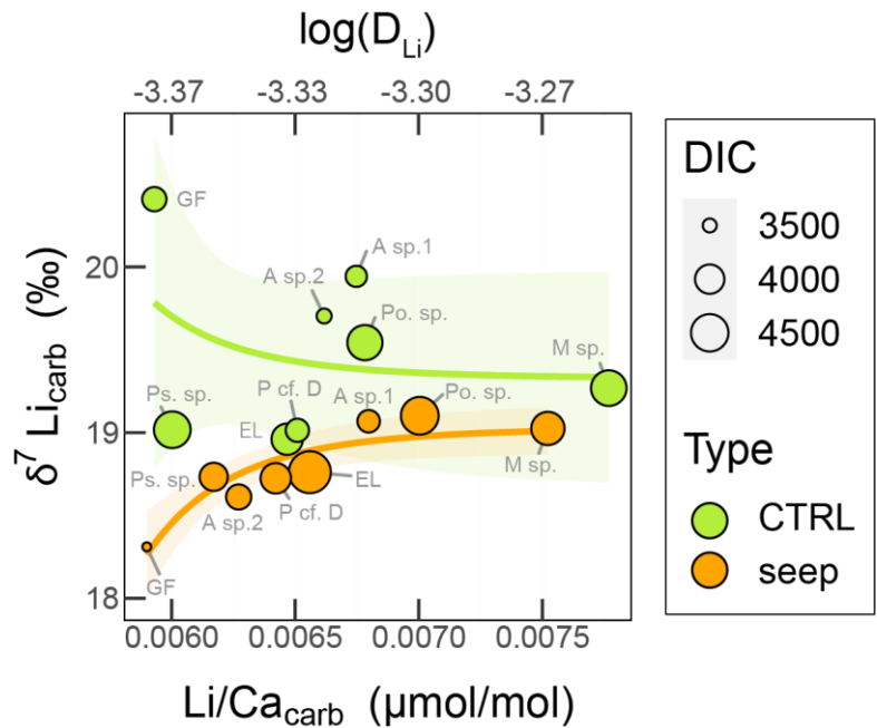
Figure 5: Coral Li isotope composition \delta^7\text{Li}_{\text{carb}} (‰) versus coral \text{Li}/\text{Ca}_{\text{carb}} concentration ratio (bottom x-axis) and partition coefficient D_{\text{Li}} (top x-axis). Orange circles are for corals living at the seep site, while green circles are for corals living at the CTRL site. Circle sizes are proportional to \text{DIC}_{\text{cf}} ( \mu\text{mol}/\text{kg} ). Solid lines are the exponential fits, and the shadow zones, the confidence intervals. Grey text refers to the initials of the corals species (see Table S1).
