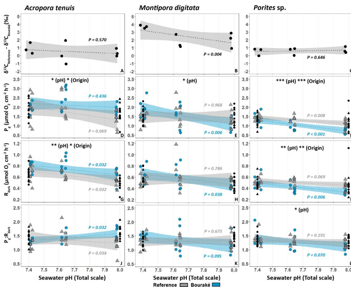
Figure VIII-13 | \delta^{13}\text{C}_{\text{Reference}} - \delta^{13}\text{C}_{\text{Bouraké}} (A-C), Gross photosynthesis ( P_g ) (D-F), dark respiration ( R_{\text{dark}} ) (G-I), and P_g:R_{\text{dark}} ratios (J-L) of Acropora tenuis , Montipora digitata and Porites sp. measured at the experimental \text{pH}_{\text{sw}} conditions. Black dots represent the difference between \delta^{13}\text{C}_{\text{Reference}} and \delta^{13}\text{C}_{\text{Bouraké}} . Blue circles and grey triangles correspond to Bouraké and Reference colonies, respectively. Largest symbols represent averaged values, while the smallest symbols represent data for each individual colony. Dashed lines represent linear model regressions fitted using linear model function in RStudio with 95% confidence intervals represented by the envelopes. ( n=7 per pH conditions, parameters, site of origin and species). The black symbols (dots for Bouraké and triangle for Reference) represent data for the Variable pH condition (incubated for photosynthesis and respiration rates measurements at both Extreme (7.53) and Control (8.11) pH) and are not included in the regressions. Stars represent statistical significance (Appendix Table VIII-14). Please, note that data in panels D-L comes from the study of chapter 4.
