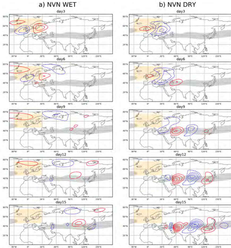
Figure 3.11: Geopotential height anomaly at 250 mb for nudging experiments on the summer climatology basic state by nudging the domain towards the lag-15day composite of (a) NVN-Wet and (b) NVN-Dry. The grey shading indicates the jet stream where the zonal wind is greater than 20m/s. The orange shading indicates the nudging domain.
