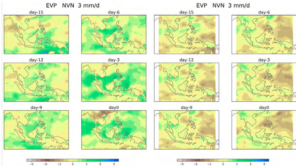
Figure 4.22: Composite of Evaporation anomaly reproduced by ERAI and RegCM4 associated with Large-scale Wet Events exceeding +3\text{mm/day} in NVN. The contour interval is 0.1\text{mm/day} .
