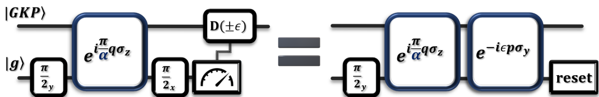
Figure 2.4: Equivalence of Ramsey-type measurement sequence of the stabilizer \mathbf{S}_q with TLS measurement-based feedback and the autonomous sequence in eq. 2.7, in which the feedback is applied via e^{-i\epsilon p\sigma_y} .
