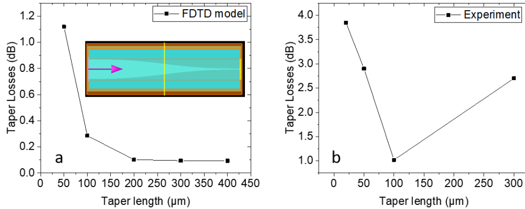
Figure 4.12: (a) Taper losses as function of the taper length. In the simulation model, all the material used were set to be lossless. Here losses are only from the non-adiabaticity of the taper. (b) Measured losses of in tapers as function of their respective length.
