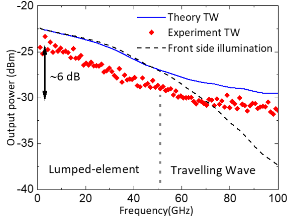
Figure 3.43: Theoretical (line) and experimental (symbols) frequency response of a 1-mm-long TW photomixer at 10 V bias and an optical power P_0=0.4 W resulting in a dc photocurrent I_{dc}=0.5 mA. In dash line is also plotted the theoretical output power assuming a front side illumination (obtained by using our model with n_{THz} = 0 ).
