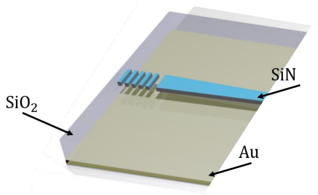
Figure 2.8: Schematic representation of the grating coupler design
