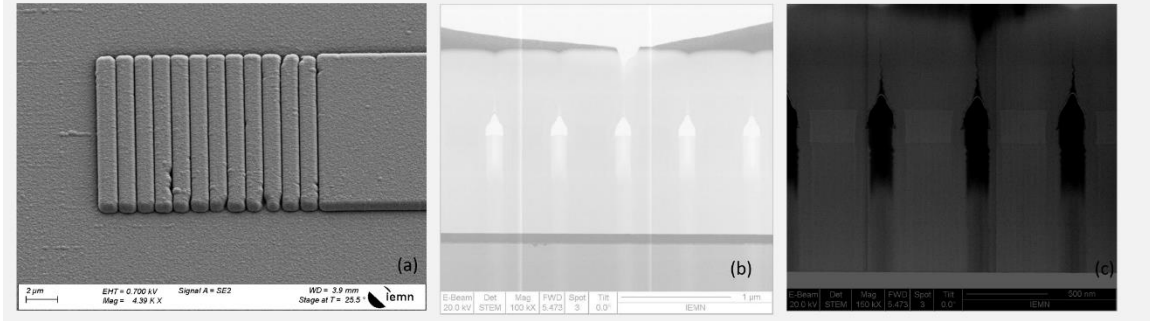
Figure 3.30: (a) SEM images showing a top view of the grating coupler and (b), (c) a side view of a FIB cut of the grating coupler.
