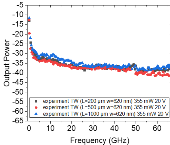
Figure 4.18: experimental frequency response of a 200\text{ }\mu\text{m} (black), 500\text{ }\mu\text{m} (red) and 1000\text{ }\mu\text{m} (blue) long TW photomixer. The bias was at 20 V and the optical power at 0.355 W resulting in a DC photocurrent of 3.65 mA, 3.957 mA and 4.63 mA respectively.
