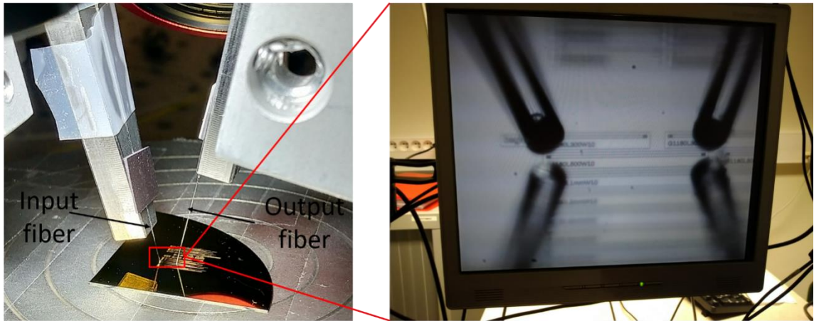
Figure 3.8: Experimental setup for the characterization of the waveguide platform. For a clear photo showing the waveguides and the optical fibers, the index matching gel is not used.
