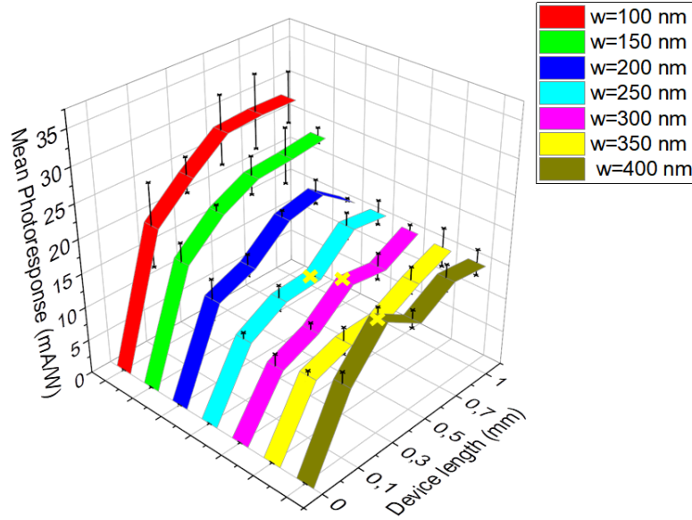
Figure 3.39: The graph shows the average photoreponse of devices with the same core width based on the device length. The photocurrent was divided by the optical power at the active region after it passed through the grating coupler and taper.
