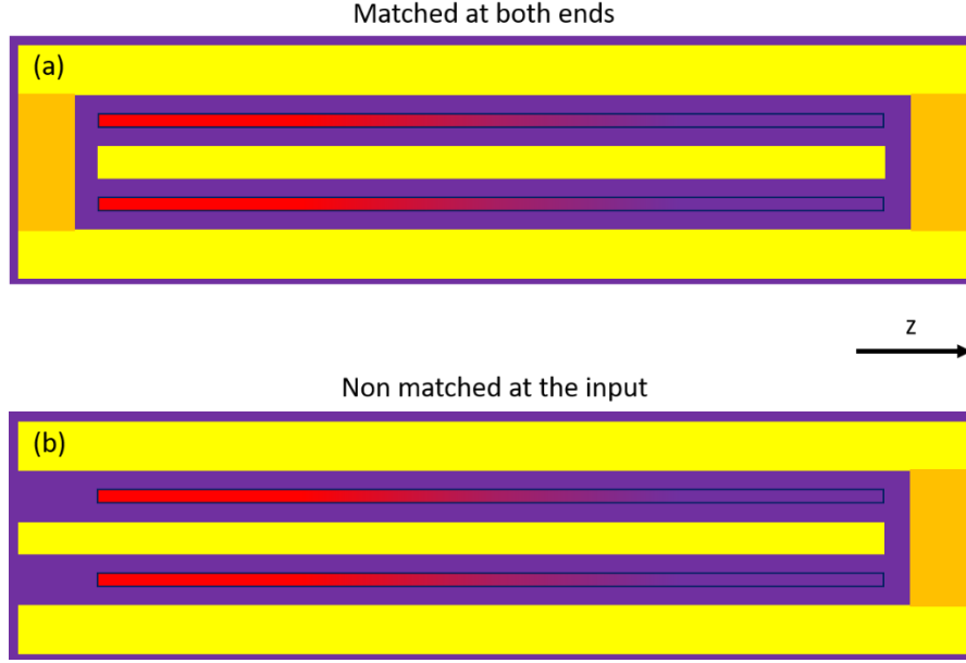
Figure 2.2: (a) Representaion of a CPW matched at both ends and (b) a CPW only matched at the output.
