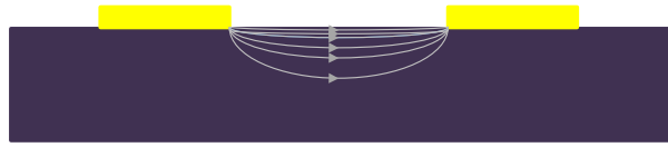
Figure 2.11: Cross-section representation of a electrodes deposited on a semiconductor material showing the semi-elliptical trajectories of the carriers following the electric field lines generated by the dc bias.
