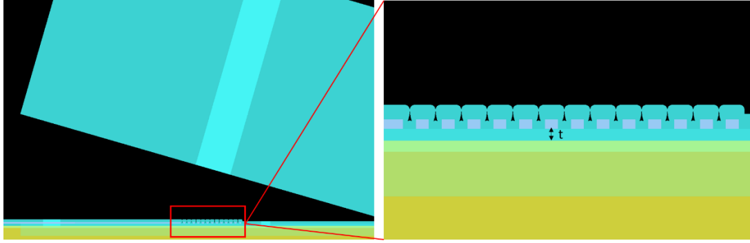
Figure 4.9: Screen capture of the 2D FDTD design showing the optical fiber above the grating coupler and an enlarged image presenting the realistic design.
