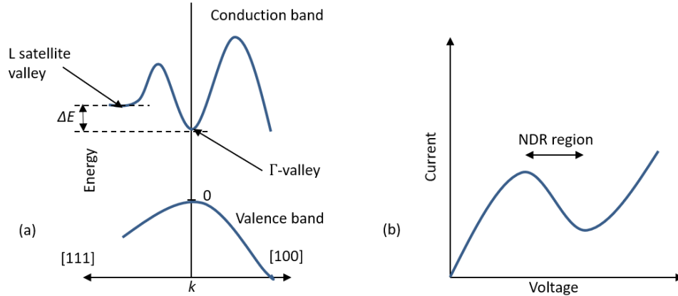
Figure 1.10: (a) Energy diagram variation due change in the orientation of GaAs. It shows the \Gamma -valley and the L-valley. (b) current-voltage characteristic curve showing the NDR region.
