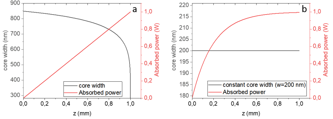
Figure 3.12: (a) Variable core width along the device (black line) allowing a linear absorbed power (in red) in the device. (b) Constant core width (200 nm) along the device (in black) resulting in a fast absorption in a 1 mm long device.
