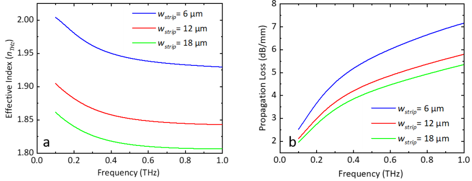
Figure 3.15: THz effective index (a) and THz propagation losses (b) for three strip widths w_{strip} ( 6 \mu\text{m} , 12 \mu\text{m} and 18 \mu\text{m} ) as function of the frequency.
