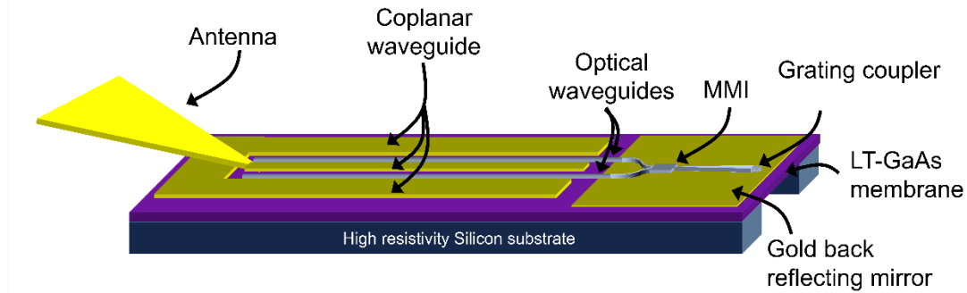
Figure 2.6: Conceptual representation of the proposed TW-photodetector showing the dielectric and the coplanar waveguides. The optical beating is coupled through a grating coupler into a \text{SiO}_2/\text{Si}_3\text{N}_4 waveguide platform. The optical mode is split into two modes by the aid of MMI (multimode interferometer). The two modes enter between the slit of the CPW and are absorbed gradually in the LT-GaAs resulting in the generation of THz waves that can be emitted by an Antenna at the output
