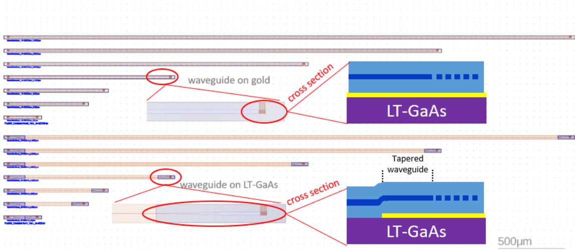
Figure 3.9: Example of the lithographic mask of a test structure presenting straight waveguides on gold and on LT-GaAs used to measure the propagation and coupling losses. Cross section representations in the grating show the main difference between the two designs.
