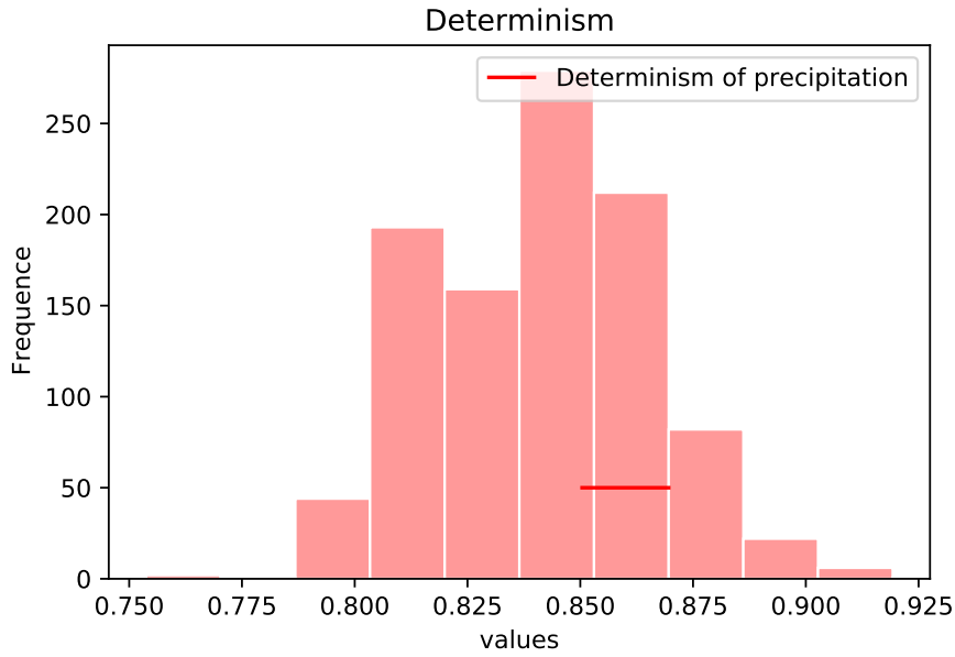
Figure 6.7: Determinism computed from AR1 using random values of a and \sigma .
