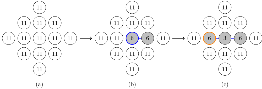
Figure 2.5. An example of transitions is presented which, starting from a fully disordered configuration (a), result in partial ordering of the system. In (b), a blue circled spin changes its value to form a bond with its right neighbor. In (c), an orange circled spin evolves to have the same color as its right neighbor. As a result, two (6) states appear in (b) and a (3) state appears in (c). The spins that have the same color are shown in grey, while the blue bonds indicate non-trivial interactions between spins, as employed in [55]. Plot taken from [5].
