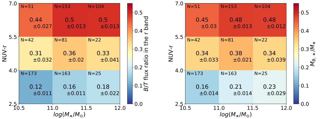
Fig. 17: Mean value of the bulge-to-total ratio for EFIGI \cap GALEX galaxies with Incl-Elong \leq 2 in color-mass cells of 0.5 dex in total stellar mass and 1.5 in NUV - r color, and derived from Fig. 16. Only the bright part of the Blue Cloud, the Green Plain and the Red Sequence are shown. The associated error on the mean, and the number of galaxies in each cell are indicated. Left: Luminosity ratio in the r band, Right: Stellar mass ratio. There is a significant increase in the bulge-to-total ratio in both luminosity and mass with the NUV - r color across the Green Plain, by a factor of \sim 1.5 - 2.6 and \sim 2.1 - 3.6 from the Blue Cloud to the Green Plain and the Red Sequence respectively. There is no effect with the galaxy stellar mass across the Green Plain, but a moderate one across the Red Sequence and sampled Blue Cloud.
