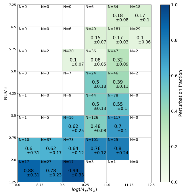
Fig. 24: Fraction of EFIGI \cap GALEX galaxies with Incl-Elong \leq 2 having an attribute value of Perturbation > 0 , all the way from the Blue Cloud to the Red Sequence. This attribute measures the distortion of the galaxy profile from rotational symmetry, with a nonzero value thus indicating an asymmetry. Galaxies are binned in cells of 0.75 dex in stellar mass and 0.75 in NUV - r color, and cells with less than 10 galaxies are discarded. The sample size as well as the error on the mean are indicated in each cell. Red Sequence galaxies are mostly unperturbed, while many of the Blue Cloud galaxies show various levels of Perturbation , with a trend of bluer galaxies being more frequently perturbed.
