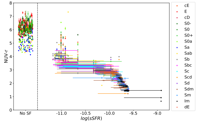
Fig. 11: Relation between the NUV - r color and the sSFR inferred by SED model-fitting for EFIGI \cap GALEX galaxies with \text{Incl-Elong} \leq 2 , showing the correlation between these two parameters, with the bluest galaxies being the most star forming, while red sequence galaxies mostly show no star formation. Intermediate colors are prone to larger uncertainties.
