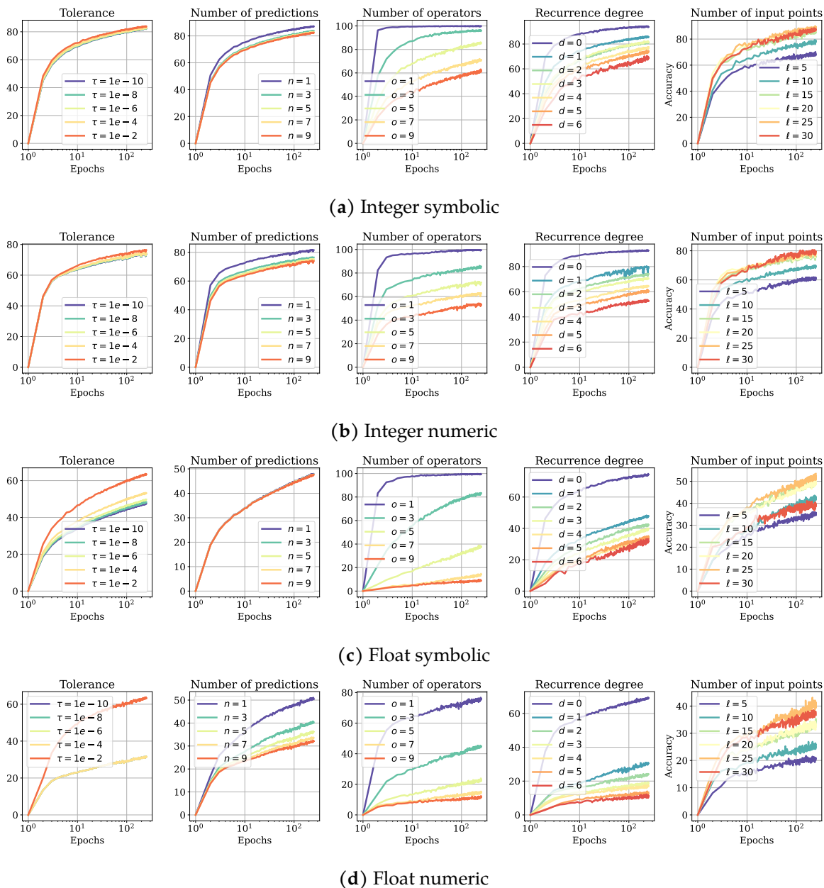
Figure F.8 – Training curves of our models. We plot the accuracy of our models at every epoch, evaluated of 10,000 sequences generated from the same distribution as during trianing. From left to right, we vary the tolerance \tau , the number of predictions n_{pred} , the number of operators o , the recurrence degree d and the number of input terms l . In each plot, we use the following defaults for quantities which are not varied: \tau = 10^{-10} , n_{pred} = 10 , o \in \llbracket 1, 10 \rrbracket , d \in \llbracket 1, 6 \rrbracket , l \in \llbracket 5, 30 \rrbracket .
