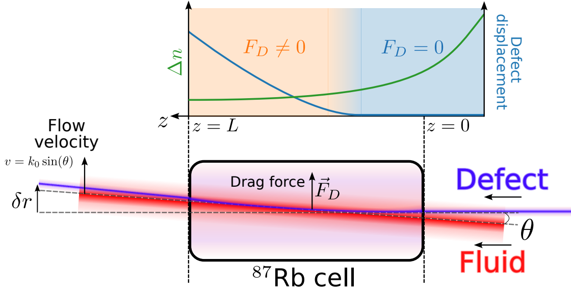
Fig. 4.13 Physical situation of the defect displacement measurement. Using side-access through the cell, we can reconstruct z -evolution of the drag force. At some point through the cell, the interaction strength \Delta n drops enough such that the critical velocity for superfluidity is lower than the initial fluid velocity. The drag force can then be measured at each point of the cell by measuring the slope of the defect displacement.
