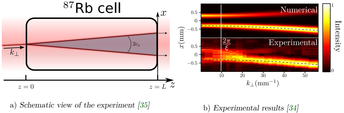
Fig. 1.3 a) The perturbation (dark red beam) is superimposed to a large gaussian background (in light red). Two localized excitations are generated propagating at the speed of sound as long as k_{\perp} < k_{\xi} . The output position of both wavepackets is recorded at the output of the cell. b) Numerical and experimental taken from [34]. The initial angle of the perturbation beam is varied and the position of the phonons is recorded. The profile is first flat until k_{\xi} before converging to a linear slope at high k_{\perp}
