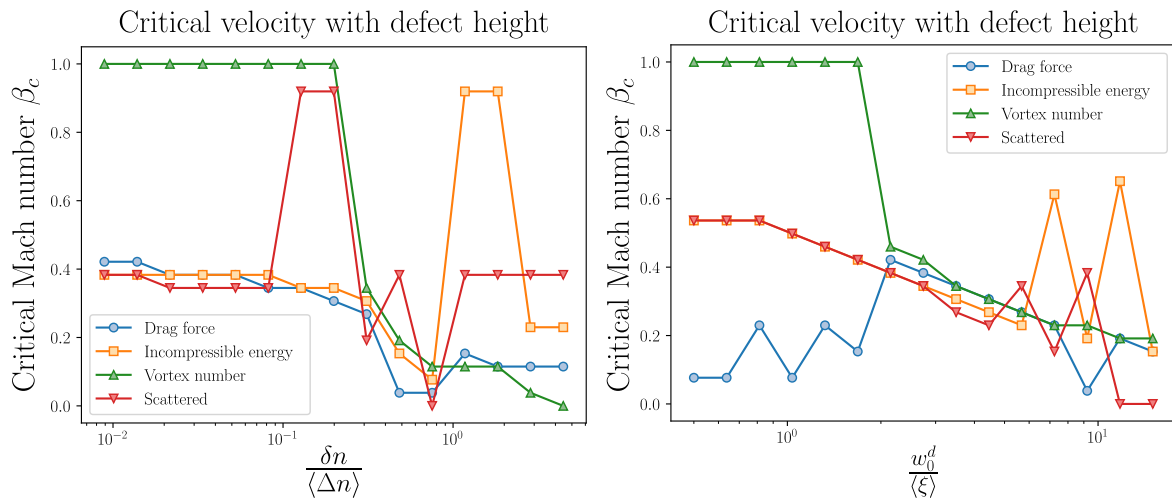
Fig. 4.7 Left: Variation of the estimated critical Mach number \beta_c = \frac{v_c}{\langle c_s \rangle} with defect height. Right: Variation of the estimated critical Mach number with defect waist. The inset describes the observables from which this critical velocity was inferred. In blue, the velocity is inferred from the zero of the drag force. In orange, the maximum of the second derivative of the incompressible energy. In green, the first velocity where the vortex number is non-zero. In red, the maximum of the second derivative of the incompressible energy.
