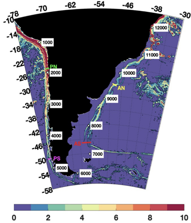
Figure 5.9: Mean Burger number from GLORYS12 over the 1993–2019 period. Black contour is Bu = 1
