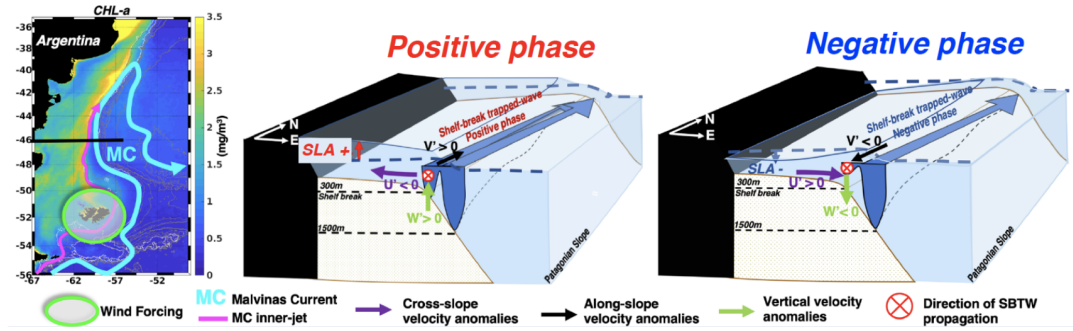
Figure 5.1: Wind-forced shelf-break trapped-waves modulate the intensity of the inner jet. Associated vertical and cross-shelf velocities bring nutrients to the Patagonian platform enhancing primary productivity.
