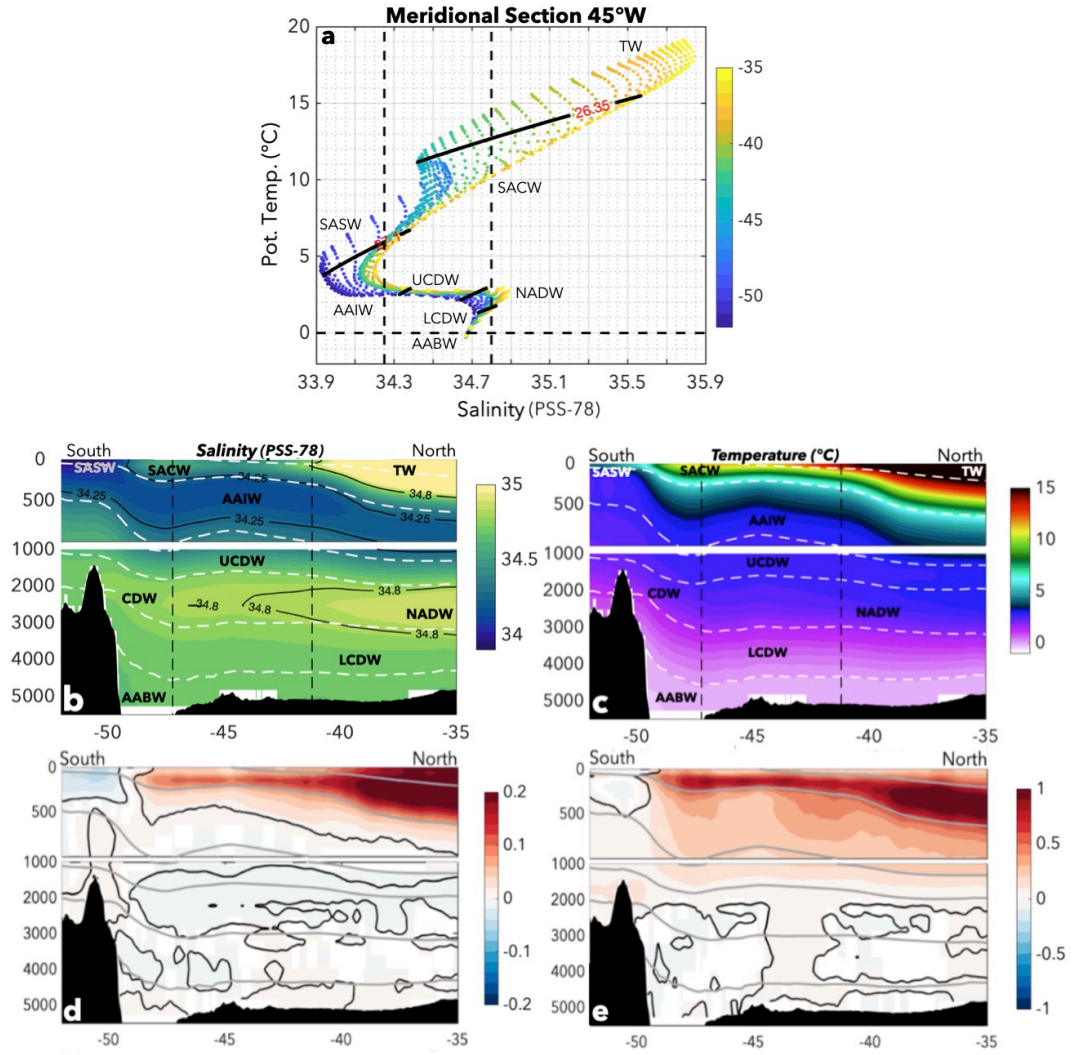
Figure 8: a) Mean \theta/S diagram along the 45^\circ\text{W} section (black line in Figure 1a). Colors indicate latitude. \gamma^n contours in black mark the limits between water masses and dotted black lines the \theta and S criteria of 0^\circ\text{C} and 34.8, 34.25 PSS-78. Main water masses are labelled. b-c) Mean salinity (b) and mean temperature (c) along the 45^\circ\text{W} section as a function of latitude and depth. \gamma^n limits are plotted in white dashed lines, salinity criteria in black. d) Salinity linear trends in \text{PSS-78.decade}^{-1} along the 45^\circ\text{W} section. Shaded values are statistically significant. e) Same as (d) for temperature in ^\circ\text{C.decade}^{-1} . \gamma^n limits are plotted in thick grey lines. Thick black lines indicate regions where the absolute value of the trend exceeds the interannual standard deviation.
