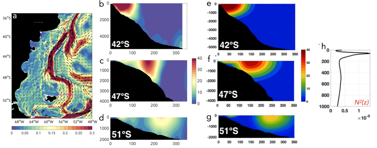
Figure 5.10: a) Mean Surface velocities and mean intensity in (m/s) over 1993-2019 period from GLORYS12. Magenta, red and blue lines correspond to the studied sections called 51°S, 47°S and 42°S respectively. b-c-d) Mean along slope velocities from GLORYS12. e-f-g) Mean flow modelled with the Brink & Chapman toolbox. h) Mean stratification used for the model implementation from GLORYS12.
