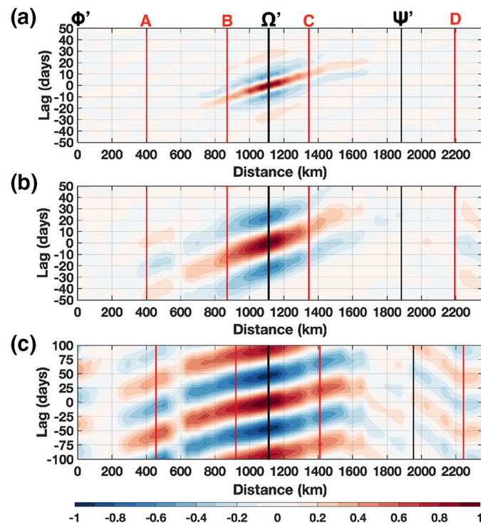
Figure 13. (a) Lagged correlations of 10–40 day band-pass filtered along-slope velocities with the velocities at \Omega (47°S), y-axis is the lag in days, x-axis is the distance along the slope above 1,500 m isobath. (b) Lagged correlations of 30–90-day band-pass filtered along-slope velocities with the velocities at \Omega (47°S), y-axis is the lag in days, x-axis is the distance along the slope. (c) Lagged correlations of 80–110-day band-pass filtered along-slope velocities with the velocities at \Omega (47°S), y-axis is the lag in days, x-axis is the distance along the slope. Phase velocities estimated as in Figure 4: (a) 25 \pm 1 , (b) 20 \pm 1 , and (c) 14 \pm 1 cm/s.
