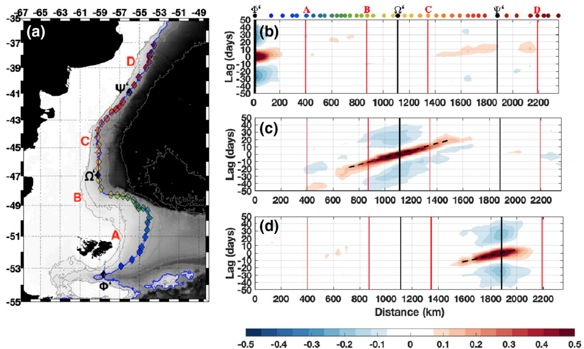
Figure 5. (a) Points along the slope used for the correlations with location \Phi' (58.6°W, 53.35°S), \Omega' (59.2°W, 47°S), and \Psi' (56°W, 41°S), blue line is the 1,500 isobath. Background is bathymetry (in m). (b–d) Lagged correlation diagrams of 110-day high-pass filtered along-slope velocities at 100 m depth over isobath 1,500 m (in the core of the MC) considering point \Phi' (b), \Omega' (c), and \Psi' (d). x-axis is the distance along the isobath and y-axis is the lag in days. Phase velocities estimated as in Figure 4: (c) 23 \pm 2 cm/s and (d) 30 \pm 2 cm/s.
