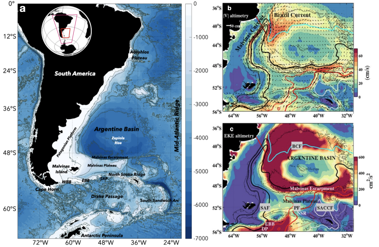
Figure 1.1: a) Bathymetry around South America in from Smith and Sandwell (1994) Mean surface velocity magnitude (in cm/s). b) mean surface velocities (larger than 10 cm/s) from gridded altimetry for the 2007–2016 period. c) Mean eddy kinetic energy per unit mass (in cm 2 /s 2 ) for the 2007–2016 period. The mean locations of the main Antarctic Circumpolar Current (ACC) fronts as defined by Barré et al. (2011) are plotted: Subantarctic Front (SAF), in black (SAF-M solid line and SAF-N dashed line); Polar Front (PF), in red (PF-M solid line and PF-N and PF-S dashed line); and Southern ACC (SACCF) in grey (SACCF-N and SACCF-S in dashed lines). (Pannels b and c from Artana et al., 2018).
