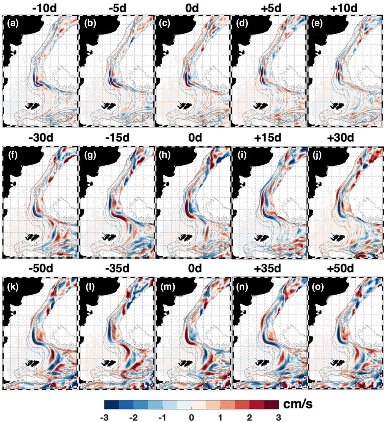
Figure 14. (a–e) Lagged composites of 10–40-day band-pass filtered along-slope velocities at 100 m from the dates when the filtered velocity exceeds the standard deviation at \Omega (47°S). (f–j) Lagged composites of 30–90-day band-pass filtered along-slope velocities at 100 m from the dates when the filtered velocity exceeds the standard deviation at \Omega (47°S). (k–o) Lagged composites of 80–110-day band-pass filtered along-slope velocities at 100 m from the dates when the filtered velocity exceeds the standard deviation at \Omega (47°S).
