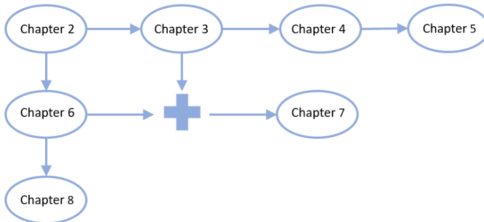
Figure 1.1: Chapters Dependency
