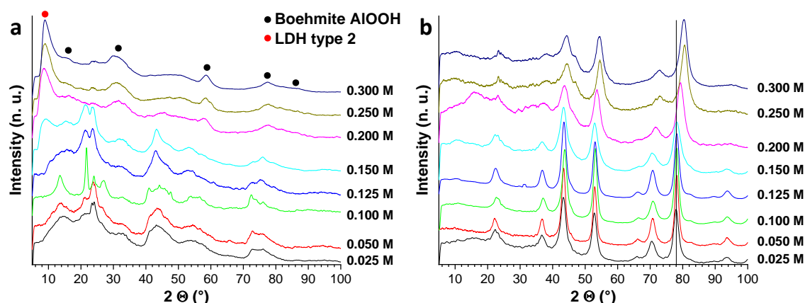
Figure 3.44: XRD of polyol synthesized materials with effect of the concentration a) before and b) after calcination at 900°C, 1 h
