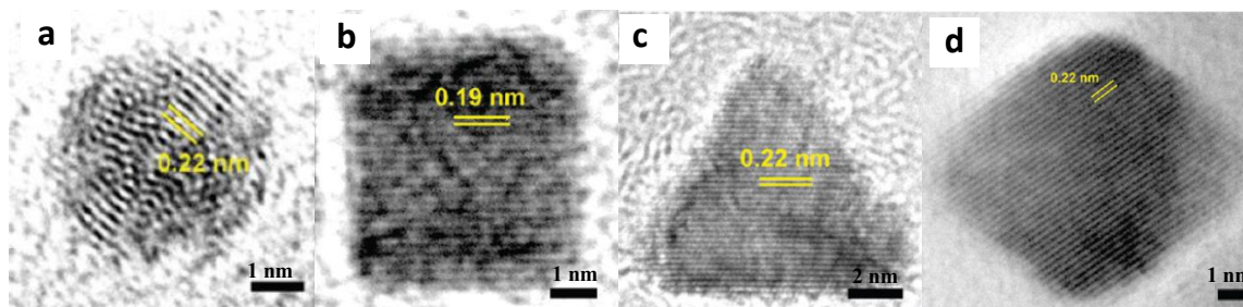
Figure 1.31: TEM of Rh nanoparticles synthesized from a) \text{Rh}_2(\text{COOCF}_3)_4 in EG, b) \text{RhBr}_3 in DEG, c) \text{RhCl}_3 in TrEG and d) \text{RhCl}_3 hot injected in 240°C TEG [160]
