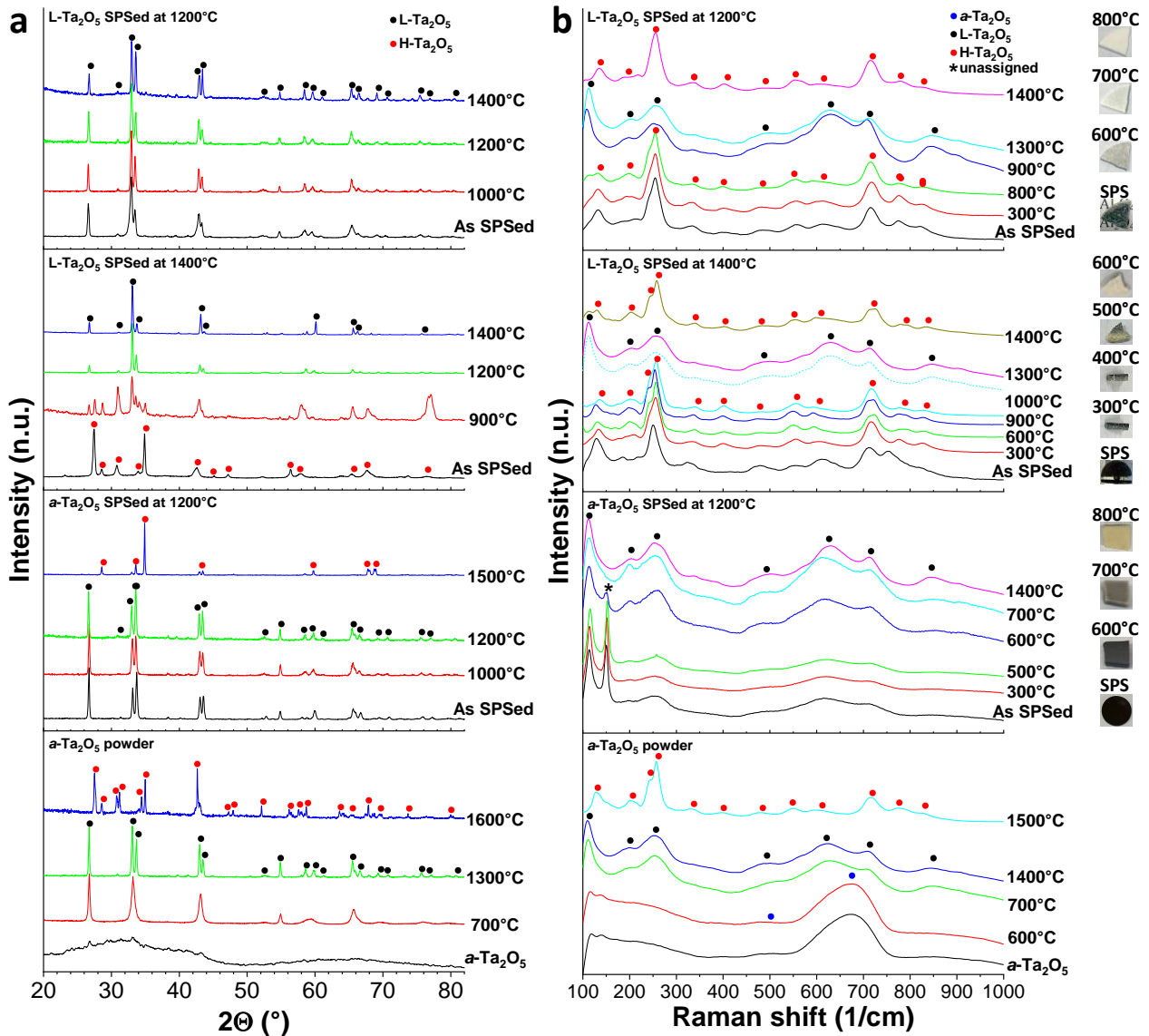
Figure 4.90: a) XRD and b) Raman spectra (cathode side) through 30 min annealing of ceramics SPSed from L- \text{Ta}_2\text{O}_5 at 1200 (1 st row) and 1400°C (2 nd row), \alpha - \text{Ta}_2\text{O}_5 at 1200°C (3 rd row) and of the \alpha - \text{Ta}_2\text{O}_5 powder (4 th row); photographs are provided on the right
