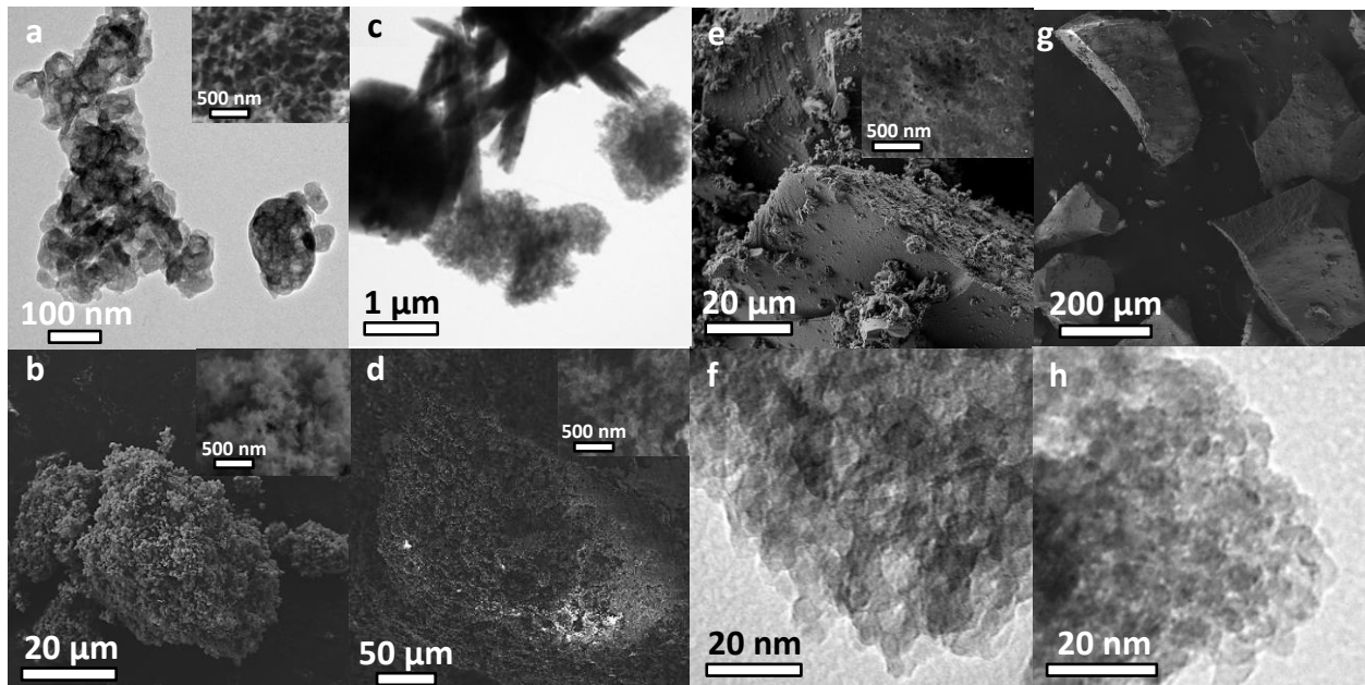
Figure 3.32: Micrographs of the powders synthesized for a)-b) x_i = 0.167 , c)-d) x_i = 0.375 , e)-f) x_i = 0.625 and g)-h) x_i = 0.833 , with a), c), e), g) the as-synthesized materials and b), d), f), h) the materials after calcination at 900^\circ\text{C} , 1 h
