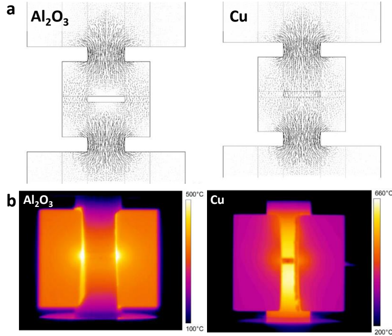
Figure 1.40: a) Modeling of SPS current distributions for \text{Al}_2\text{O}_3 and Cu [207] and b) experimental temperature distributions [208]
