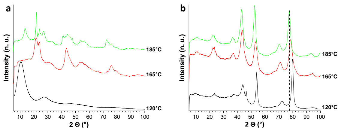
Figure 3.11: XRD patterns of the samples synthesized at different synthesis temperature a) before and b) after calcination at 800°C
