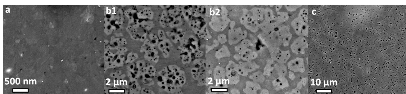
Figure 4.61: SEM of the ceramics from polyol \text{MgO} \cdot n\text{Al}_2\text{O}_3 powders with n = a) 0.716, b) 1 and c) 5, at a,b2,c) 1450 and b1) 1375°C
