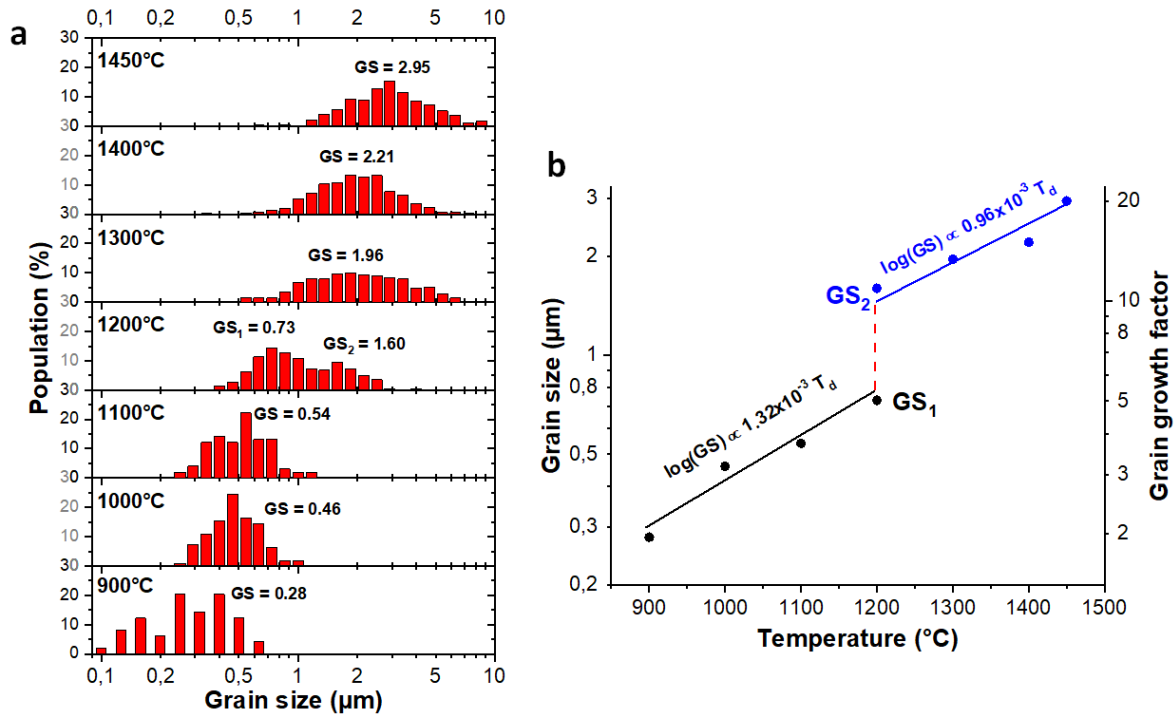
Figure 4.17: a) Histograms of grain size distribution (GSD) of Sasol MAS ceramics SPSeD for 20 min at 900, 1000, 1100, 1200, 1300, 1400 and 1450°C and b) modes of GSD plotted as a function of the sintering temperature
