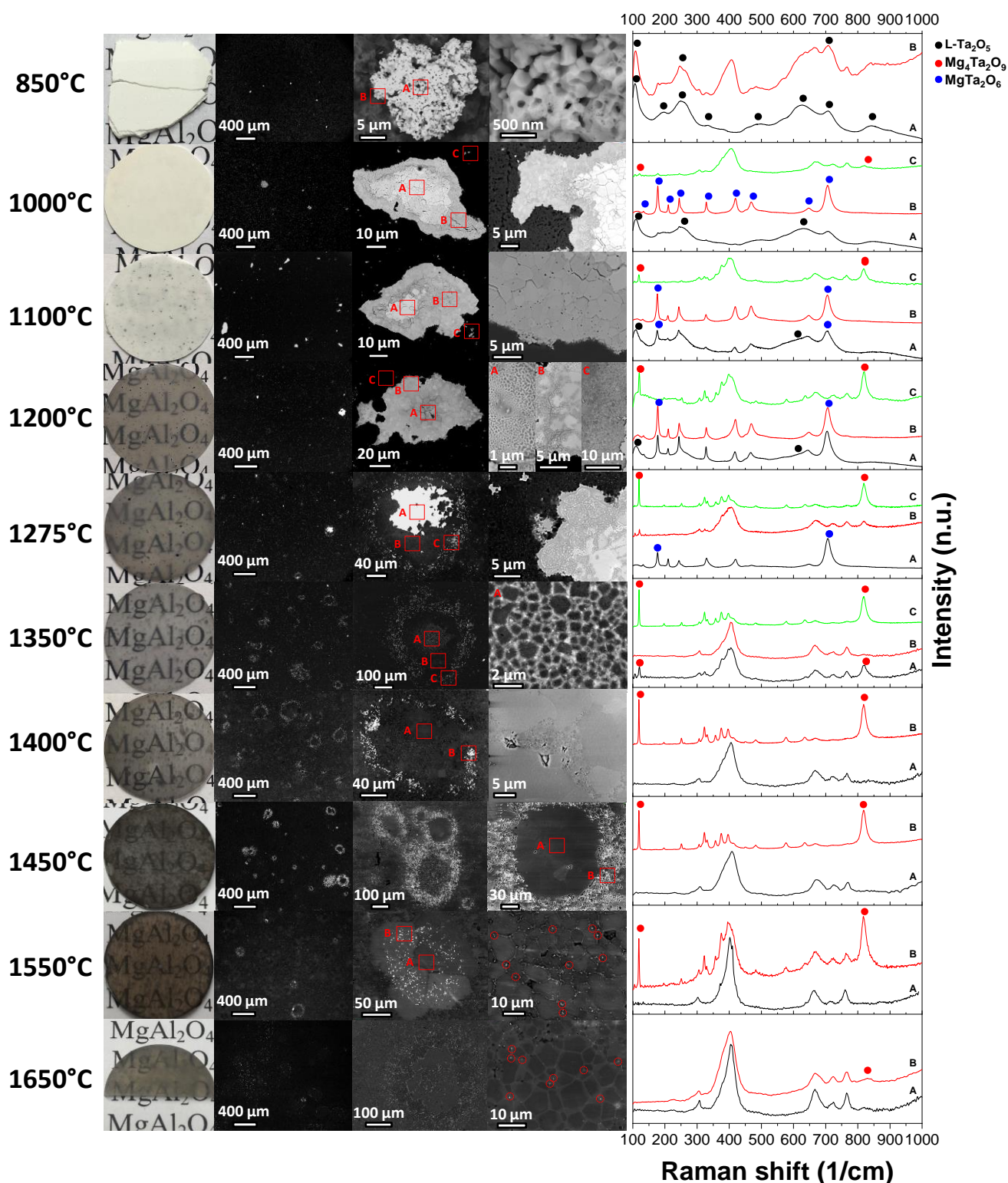
Figure 4.97: Evolution of the \text{Ta}_2\text{O}_5 added MAS ceramics with the sintering temperature from 850^\circ\text{C} ( 1^{\text{st}} row) to 1650^\circ\text{C} (last row): photographs ( 1^{\text{st}} col.), SEM with low magnification ( 2^{\text{nd}} col.), focus on a Ta-based inclusion ( 3^{\text{rd}} col.) and details of such inclusions and/or in their vicinity ( 4^{\text{th}} col.), with local Raman analysis of areas indicated by red squares ( 5^{\text{th}} col.)
