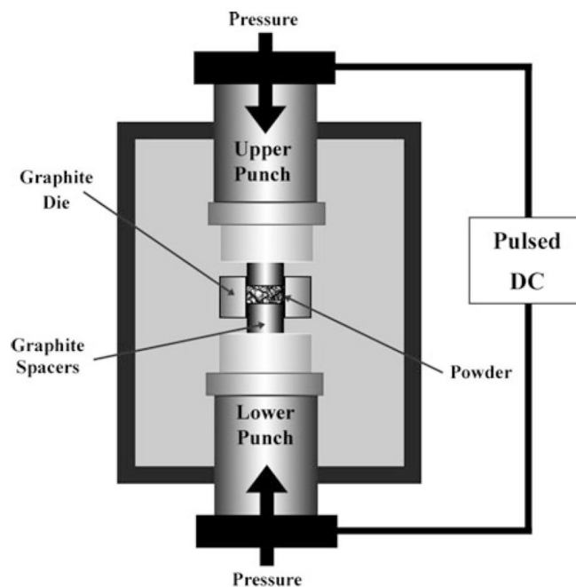
Figure 1.39: Schematic representation of the SPS apparatus principle [80]
