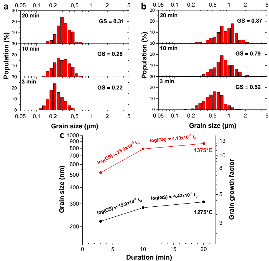
Figure 4.43: Histograms of grain size distribution of S25CR-3MS MAS ceramics SPSeD at a) 1275 and b) 1375°C for 3, 10 and 20 min, and c) modes of GSD plotted as a function of the sintering dwell duration
