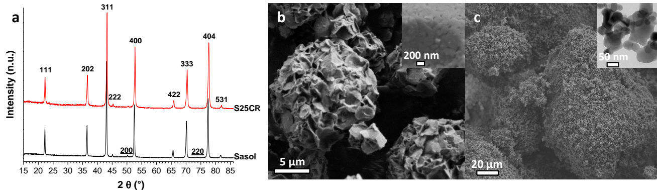
Figure 2.2: a) XRD patterns with indexation for spinel \text{MgAl}_2\text{O}_4 , except underlined indexation for periclase \text{MgO} ; micrographs of the b) Sasol and c) S25CR commercial powders
