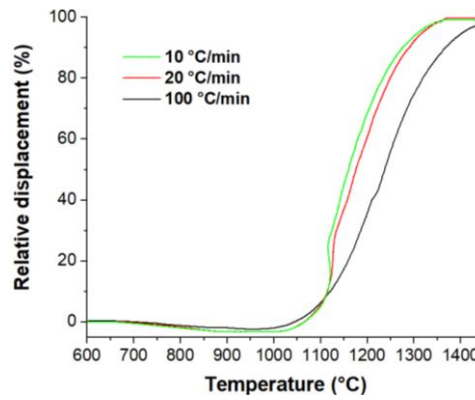
Figure 4.23: Relative displacement of the SPS pistons during sintering of Sasol powder with heating rate of 100, 20 and 10^\circ\text{C/min}
