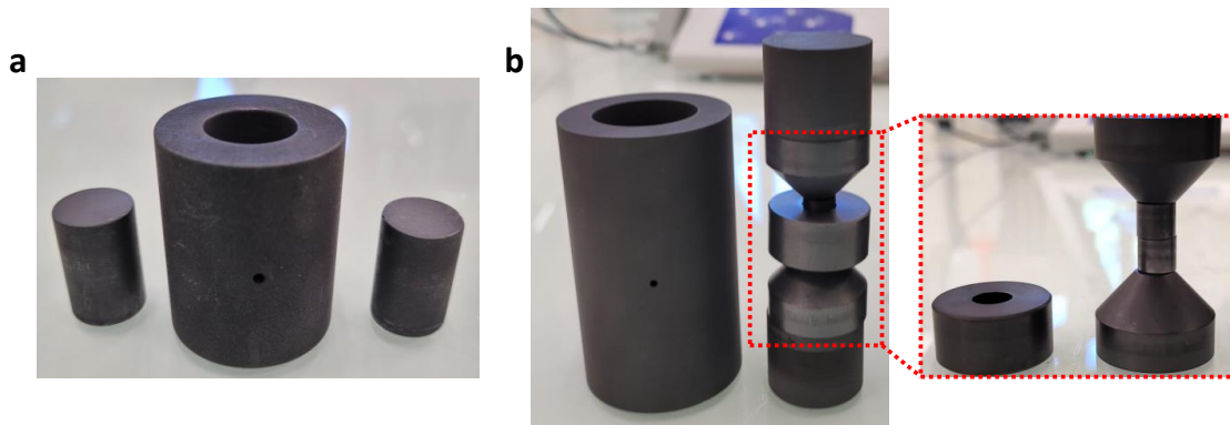
Figure 2.8: a) Graphite die used for standard SPS ( P \leq 100 MPa) and b) SiC inner die within graphite die for HPSPS ( P \leq 1 GPa)
