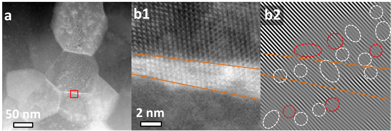
Figure 5.16: a) HAADF-STEM micrograph of the ceramic SPSe at 500 MPa; b1) high magnification on the grain boundary interface in red square area in a), and b2) the corresponding inverse fast Fourier transform (IFFT) constructed from (220) planes, with most of the edge dislocations and stacking fault circled in white and red, respectively; the grain boundary is highlighted in b1) and b2) by orange lines
