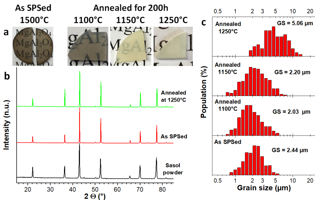
Figure 5.1: Sasol ceramic SPSed at 1500^\circ\text{C} (3 min, 80 MPa) and subsequently annealed at 1100, 1150 and 1250^\circ\text{C} for 200 h: a) photographs, b) XRD patterns and c) grain size distributions
