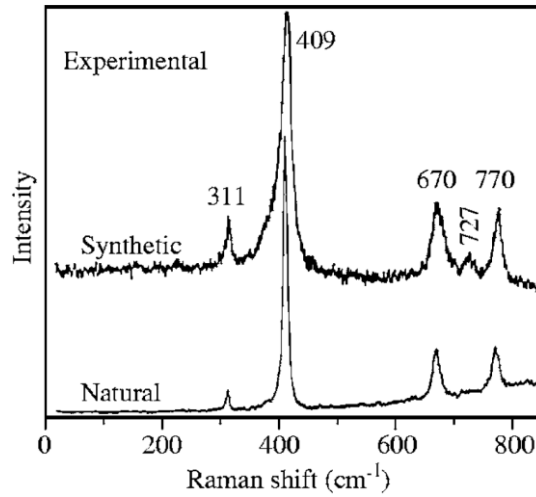
Figure 1.7: Raman spectra for natural (normal) and synthetic (partly inverse) \text{MgAl}_2\text{O}_4 spinels [54]
