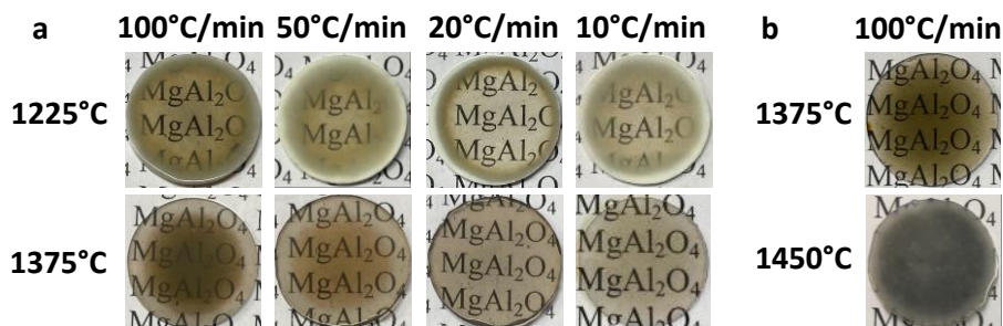
Figure 4.45: Photographs of S25CR-3MS ceramics SPSeD a) at 1225 and 1375°C for 20 min with 10 \leq \alpha \leq 100^\circ\text{C/min} , and b) at 1375 and 1450°C for 3 min with heating rate of 100^\circ\text{C/min}
