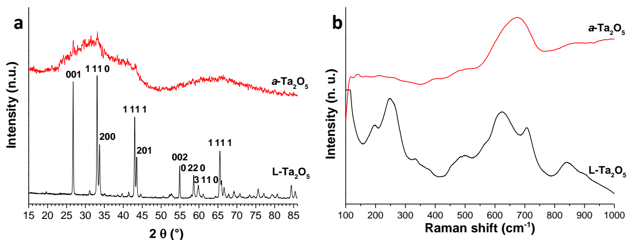
Figure 2.5: a) XRD patterns and b) Raman spectra of \text{Ta}_2\text{O}_5 commercial powders
