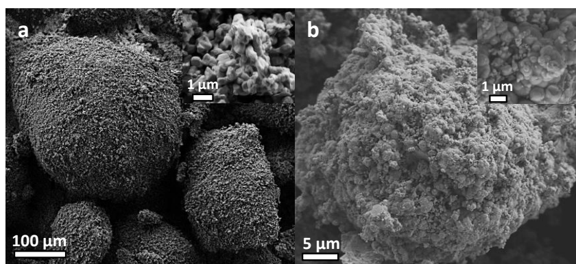
Figure 2.6: Micrographs of a) L- \text{Ta}_2\text{O}_5 and b) a- \text{Ta}_2\text{O}_5 commercial powders
