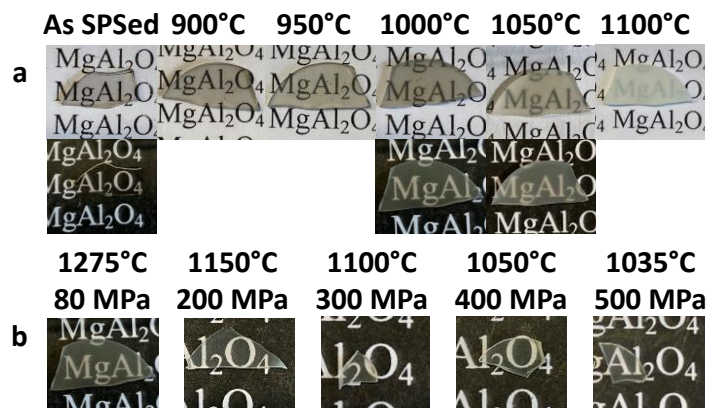
Figure 4.77: Photographs of S25CR-3MS ceramics a) SPSed at 1275°C and 80 MPa successively treated for 200 h at 900-1100°C and b) SPSed at different P-T d conditions treated at 1000°C for 200 h; black background is aimed to emphasize cloudiness
