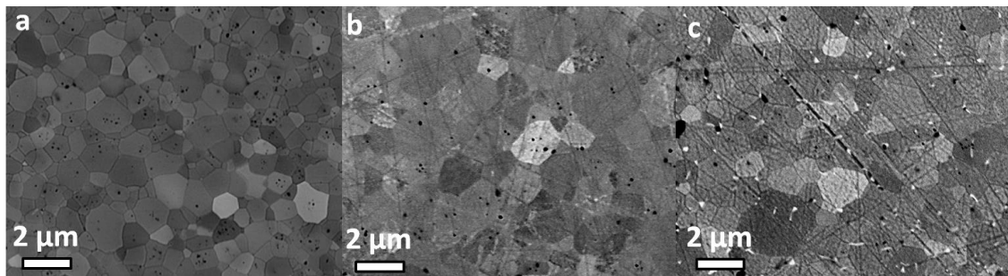
Figure 4.24: SEM of Sasol MAS ceramics SPSed at 1450°C for 3 min with heating rate of a) 100, b) 20 and c) 10^\circ\text{C/min}
