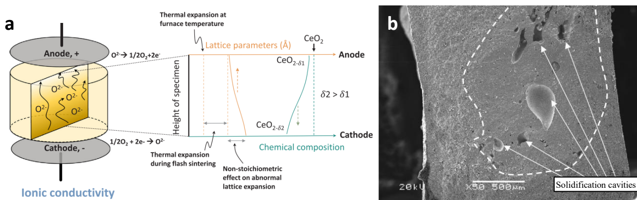
Figure 1.44: a) \text{O}^{2-} migration in \text{CeO}_2 from cathode to anode during FS inducing gradients of composition and cell constant [255]. Hot-spot generated in celcian subjected to FS, with some shrinkage cavities due to local melting [257]
