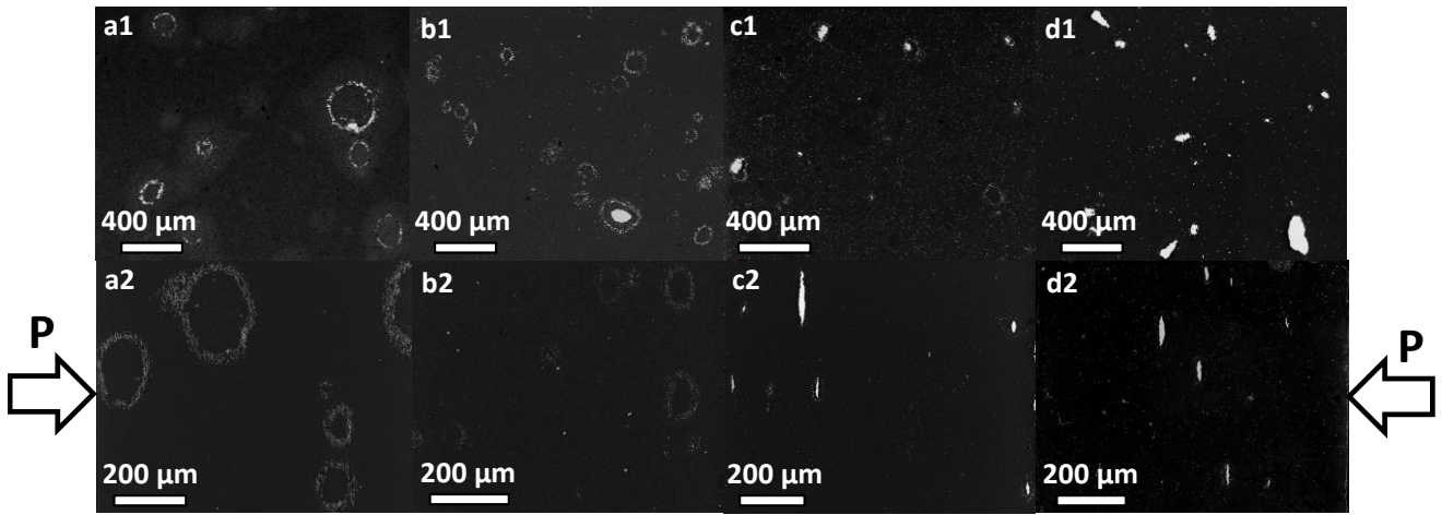
Figure 4.102: SEM micrographs of 1 wt% \text{Ta}_2\text{O}_5 added Sasol ceramics SPSeD at 1450^\circ\text{C} with an applied pressure of a1,a2) 80 MPa, b1,b2) 130 MPa, c1,c2) 180 MPa and d1,d2) 230 MPa, on a1-d1) the radial and a2-d2) the cross sections
