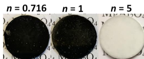
Figure 4.60: Photographs of the ceramics SPSed at 1450°C from the polyol \text{MgO} \cdot n\text{Al}_2\text{O}_3 precursors with n = 0.716 , 1 and 5
