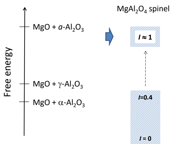
Figure 3.56: Tentative schema of inverse spinel formation ( I \approx 1 ), following Ostwald's rule of phase nucleation
