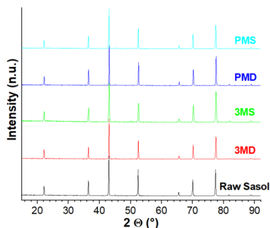
Figure 4.5: X-Ray diffractograms of the ceramics SPSe from the Sasol powder treated by different mechanical processing
