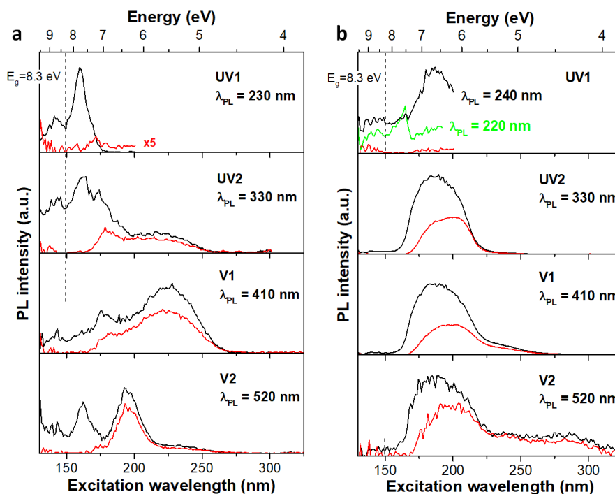
Figure 5.25: PLE spectra (9K) of a) pure and b) 1 wt% Ta 2 O 5 added Sasol MAS ceramics before (black and green curves) and after He + irradiation (red curves) at the different indicated emission band and respective wavelengths of photoluminescence \lambda_{PL}
