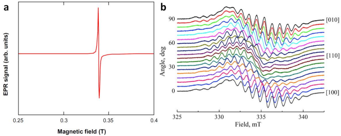
Figure 1.8: EPR spectra of MAS single crystal: a) \text{F}^+ centers [8] and b) \text{V}_1 center with rotation around [001] direction [38]
