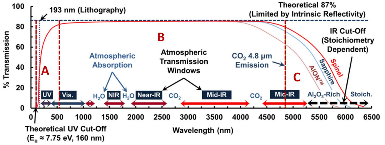
Figure 1.13: Typical transmission spectrum for MAS, along with other transparent materials; (A) the UV cut-off or band gap, (B) the optical transparency window and (C) the multiphonon or IR cut-off [11]
