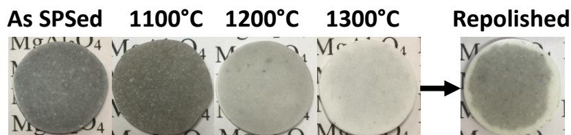
Figure 4.75: Photographs of a MgUPA1250 ceramic successively annealed for 1 h at 1100, 1200 and 1300°C, then repolished
