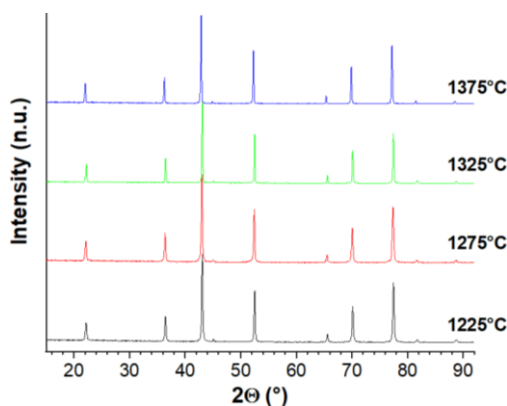
Figure 4.38: XRD patterns of S25CR-3MS MAS ceramics SPSed at 1225, 1275, 1325 and 1375°C for 20 min
