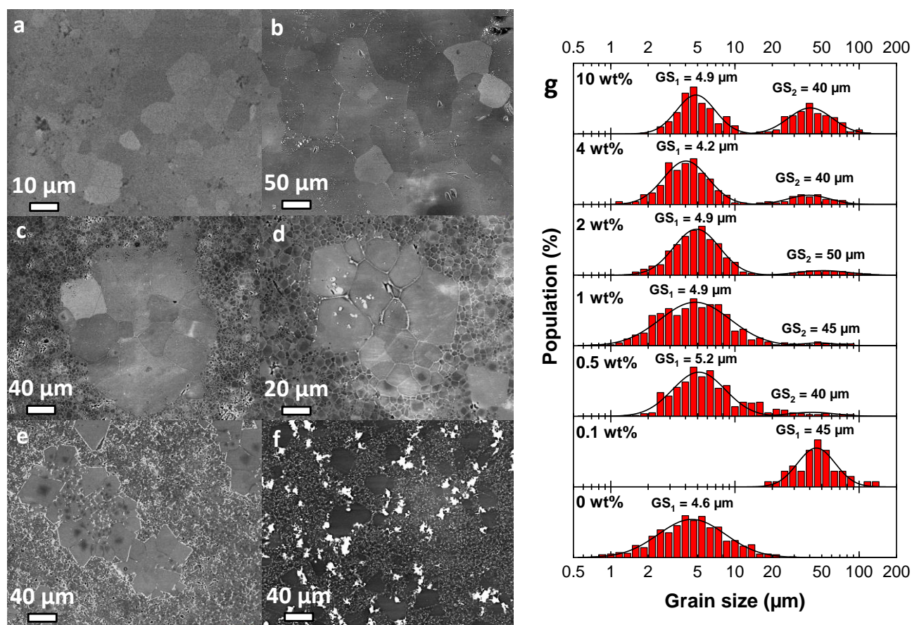
Figure 4.96: SEM micrographs of the MAS ceramics SPSeD at 1650°C with \text{Ta}_2\text{O}_5 addition rate of a) 0 wt% (pure MAS), b) 0.1 wt%, c) 0.5 wt%, d) 1 wt%, e) 4 wt% and f) 10 wt%, and g) the evolution of the grain size distribution with the \text{Ta}_2\text{O}_5 addition rate
