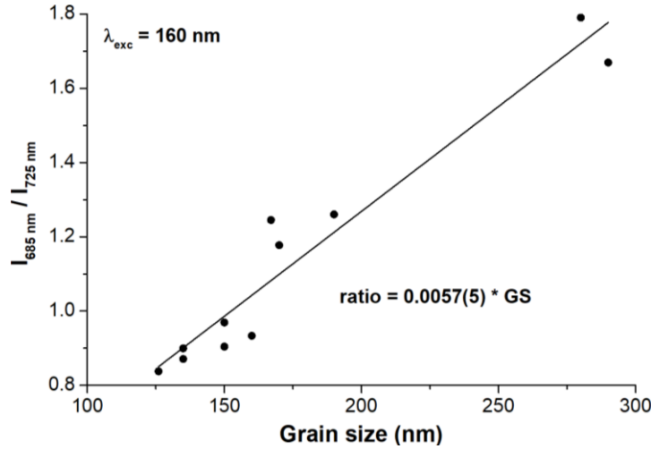
Figure 5.21: Intensity ratio between structured ( \lambda_{em} = 685\text{ nm} ) and non-structured ( \lambda_{em} = 725\text{ nm} ) PL of Cr^{3+} impurity in MgAl_2O_4 ceramics spinel versus crystalline grain size for \lambda_{exc} = 160\text{ nm} ; linear least-squares fit of experimental data is shown by solid line
