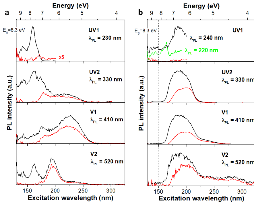
Figure 5.25: PLE spectra (9K) of a) pure and b) 1 wt% \text{Ta}_2\text{O}_5 added Sasol MAS ceramics before (black and green curves) and after \text{He}^+ irradiation (red curves) at the different indicated emission band and respective wavelengths of photoluminescence \lambda_{\text{PL}} .
