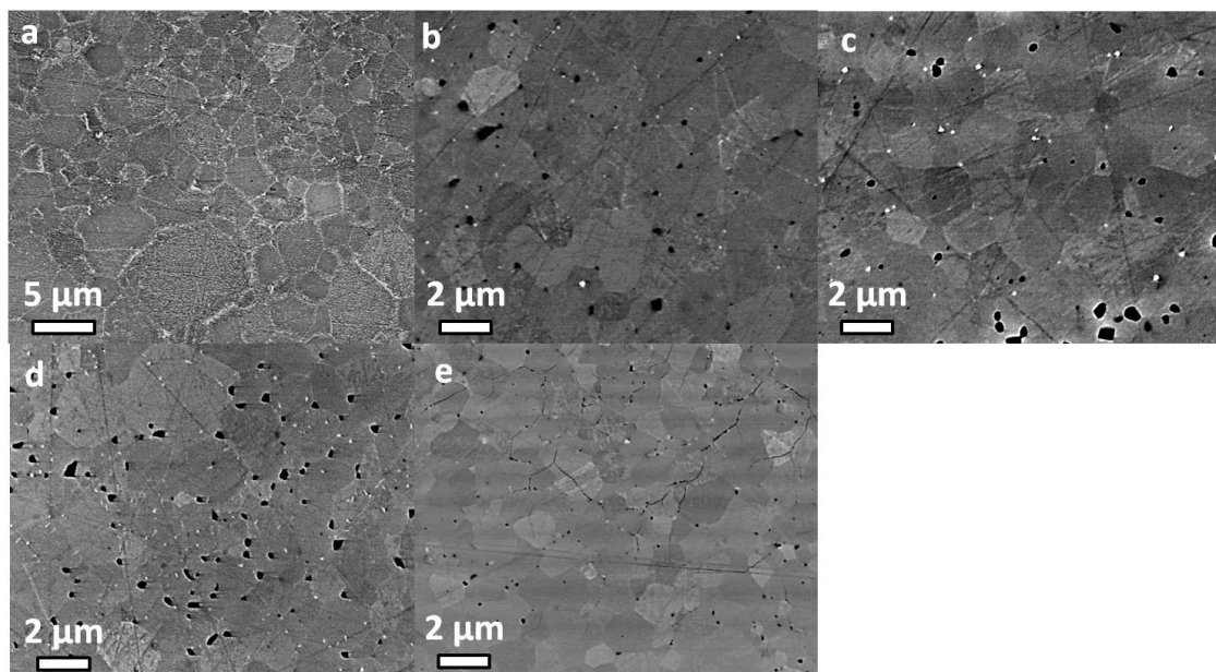
Figure 4.6: SEM of the ceramics SPSe at 1450°C from the Sasol powder a) as received, b) 3MD, c) 3MS, d) PMD200-BPR10 and e) PMS200-BPR10
