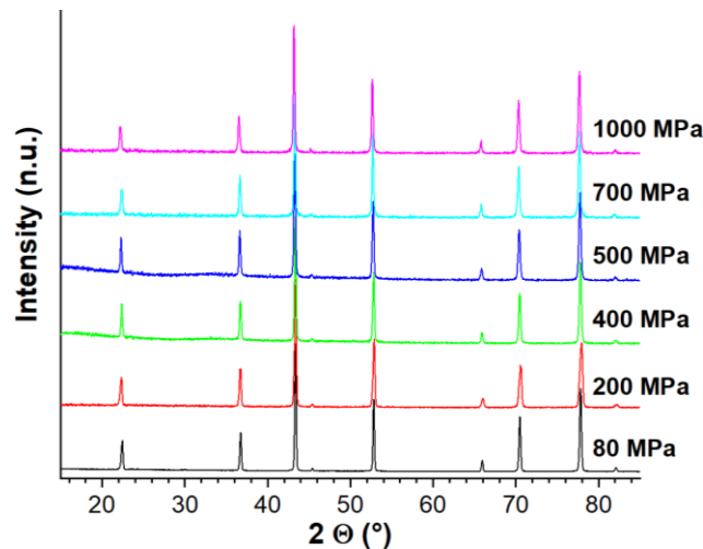
Figure 5.14: XRD patterns of the S25CR-3MS \text{MgAl}_2\text{O}_4 ceramics prepared by SPS at 80-1000 MPa
