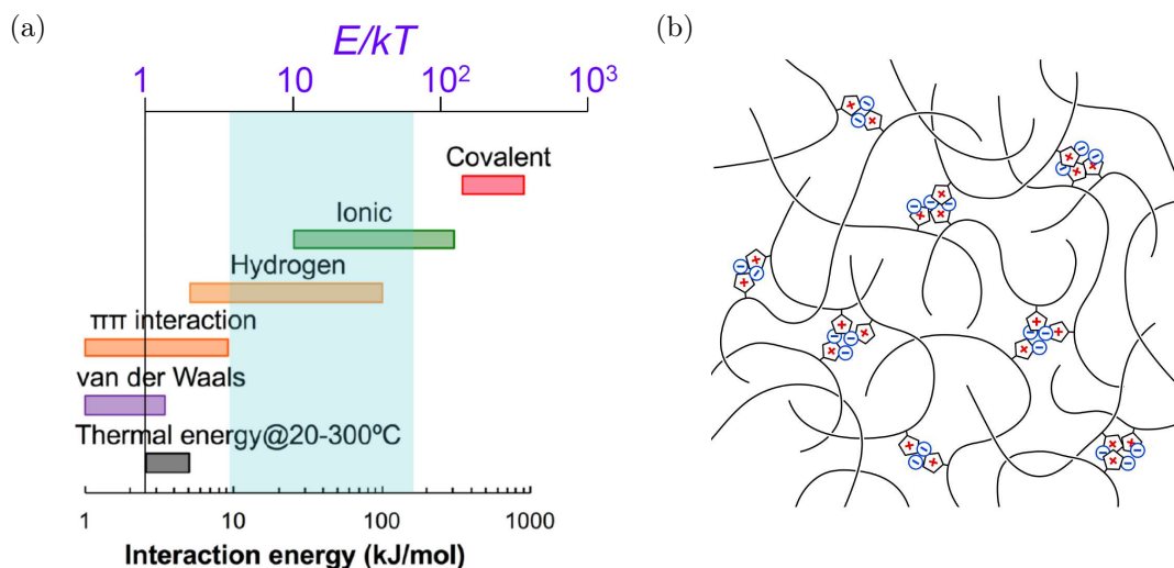
Figure 1.10: (a) Interaction energies of diverse bond types, ideal energies for reversible bond networks, are shown in light blue. Figure taken from Pr. R.H. Colby's lecture at the SOFTMAT summer school 2022, adapted from ref. [110]. (b) Schematic representation of an associating polymer network based on ionic bonds.
