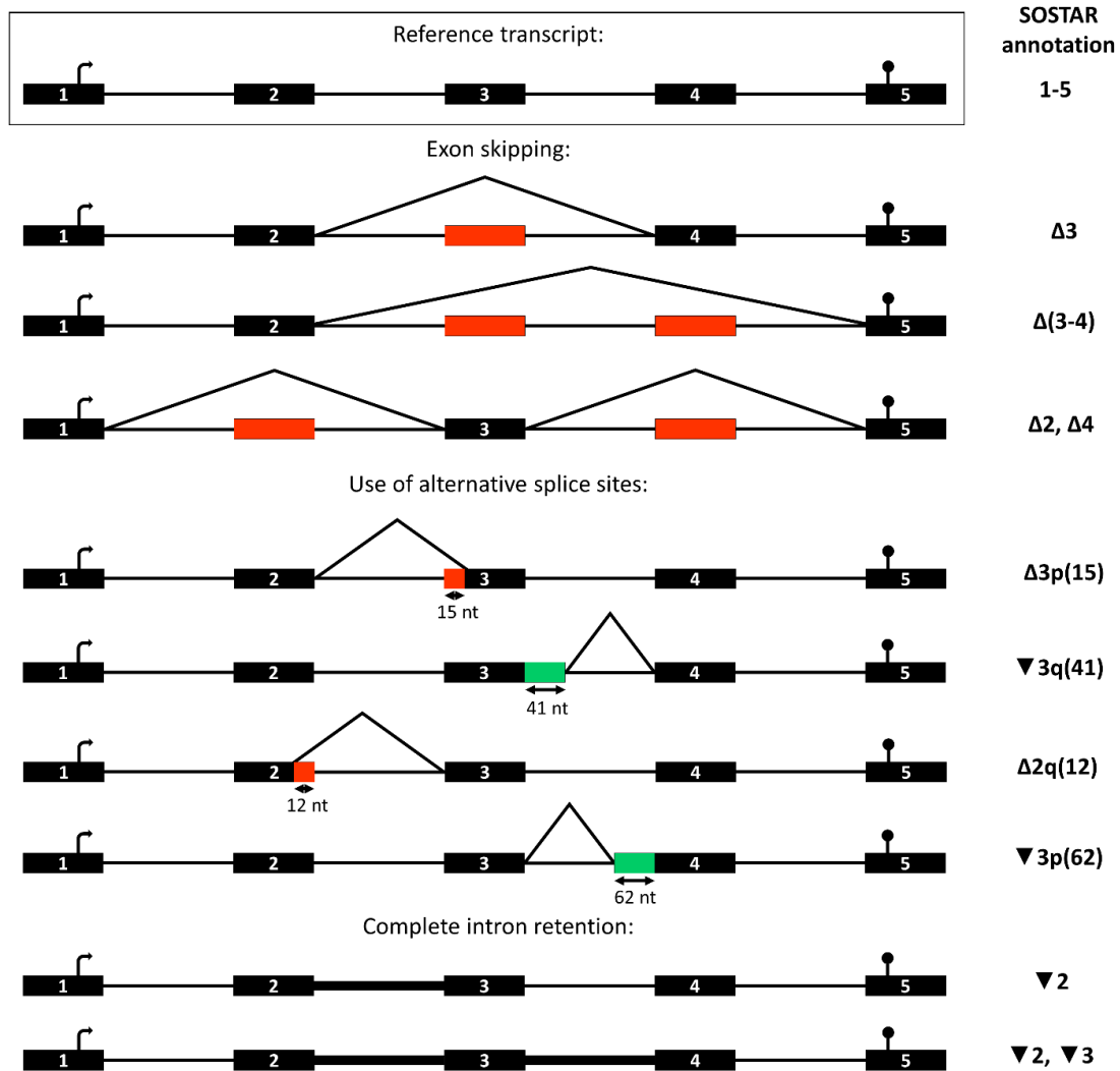
Figure S1: Mechanisms of the transcript diversity with the corresponding SOSTAR annotation. Black boxes: exons, black lines: intron, red boxes: exon (or part of exon) skipping, green boxes: novel exon (or part of exon).
