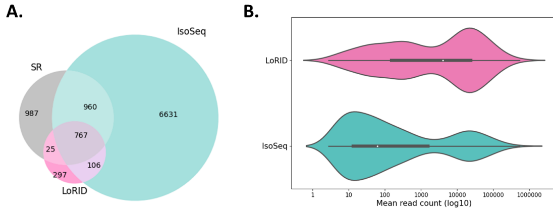
Figure 4: Comparison of splicing junctions between SRS and LRS for the whole gene panel. A. Venn diagram of splicing junctions detected by SRS and LRS B. Violin plot of mean read counts of common junctions between SRS and LRS junctions. Values are plotted on a logarithmic scale.
