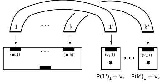
Figure 3.9.: Gluing pattern for surface S^2 \setminus \mathbb{D} with marked points \{v_1, \dots, v_k\} .
