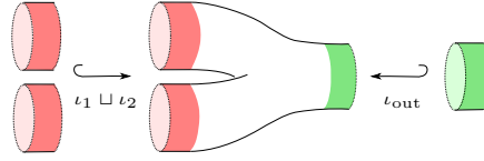
Figure 2.9.: The maps inducing the monoidal structure \otimes_{\text{Pants}} .
