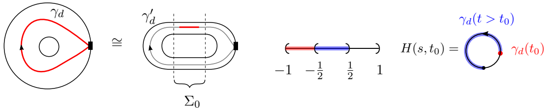
(a) Collar gluing for D -decorated annulus. (b) Sketch of the homotopy H for some fixed t_0 \in [0, 1] .
