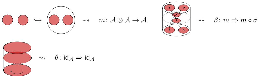
Figure 1.3.: First row : Disk embeddings (or isotopies thereof) in \mathbb{D}\text{isk}_2^{\text{or}} that give rise to the multiplication m and the braiding \beta in \mathcal{A} = \mathcal{A}(\mathbb{R}^2) . Here \sigma denotes the braiding in \mathcal{C} . Second row : Loop in the space of disk embeddings \mathbb{D}\text{isk}_2^{\text{or}} coming from rotating the disk by 2\pi .
