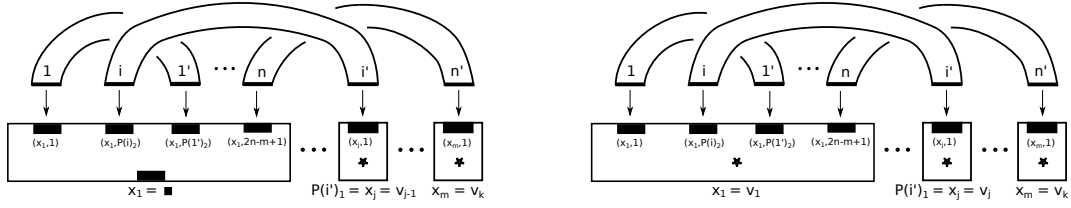
(a) Surface \Sigma with marked interval in its boundary. In the above, n = 2g + r + k - 1 and m = k + 1 .
