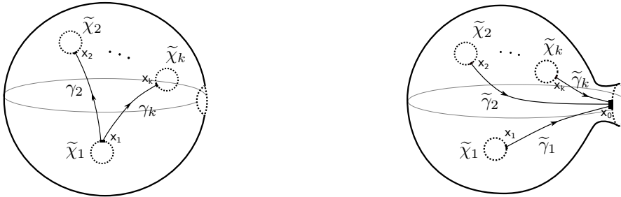
(a) Combinatorial presentation of \bar{\Sigma} \setminus \mathbb{D} used to compute the algebra of dynamical boundary-boundary holonomies.
