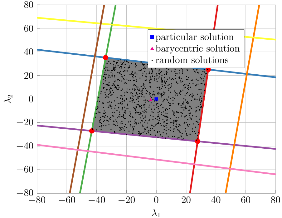
Figure 2.19 – Simulated Feasibility Polygon in the \lambda -space, plotted for pose \mathbf{x} = [2.258, 2.310, 1.000, 0, 0, 0]^T
