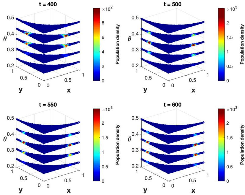
Figure 3.8: Intermediate stages of the population density for different values of \theta : While the differentiation process continues, we observe further loss in plasticity. Around t = 500 (top right) most of the population has reached \theta = 0.375 and at subsequent times the migration continues.
