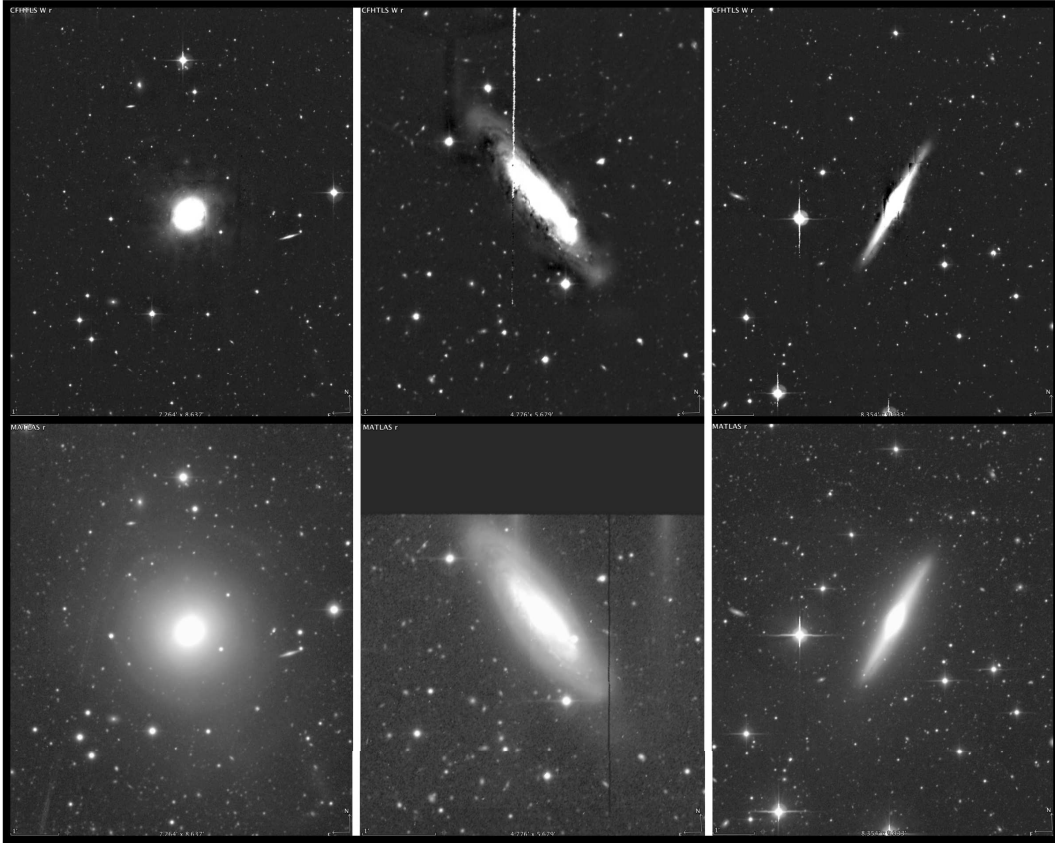
Figure 3.1: Illustration of the over-subtraction of the background after data processing by the Elixir pipeline for CFHTLS-Wide r -band images. Top: CFHTLS-Wide r -band images. Bottom: same galaxies observed by MATLAS in the r -band, treated with an LSB-compliant pipeline.
