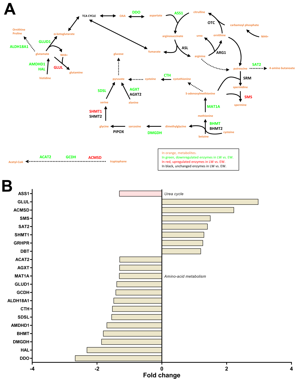
Figure 6. Regulation of liver amino acid metabolism and the urea cycle in grey mouse lemurs during winter. The relative abundance of liver proteins involved in amino acid metabolism and the urea cycle in early (EW) and late (LW) winter mouse lemurs (N = 5/group) is shown using a color code in the corresponding pathways (panel A), and mean fold changes in LW vs. EW can be visualized in (panel B).
