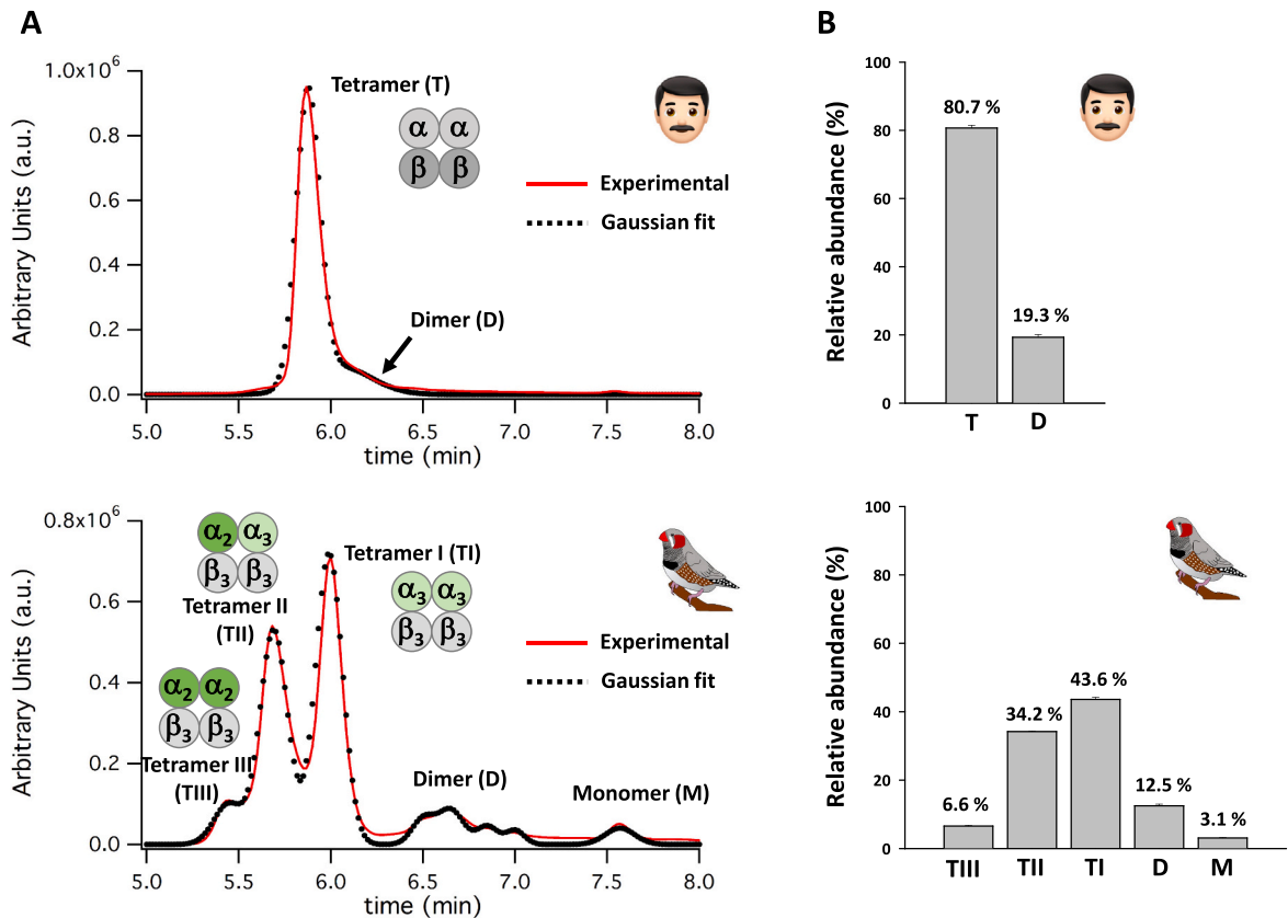
Fig. 4. Oligomeric states and proportions of human and zebra finch hemoglobins LC-UV-MS analysis of whole hemoglobins allowed visualizing different oligomer states (see the representative chromatograms in panel A) and determining their relative proportions (mean \pm sem of 8 independent determinations, panel B). Mass spectra obtained after dissociation of zebra finch tetramers inside the mass spectrometer are shown in Supplementary Figs. 5–6.
