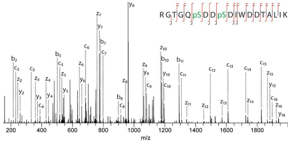
Figure 24: Spectre MS/MS EThcD d'un peptide doublement phosphorylé.
