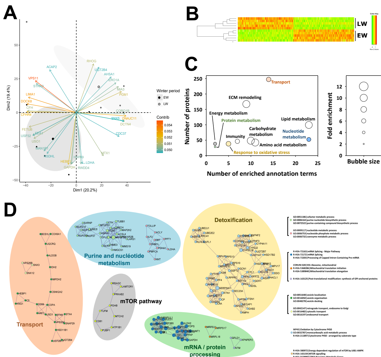
Figure 2. Overview of liver proteomics data. Principal component analysis performed from expression levels of all 4522 proteins analyzed using mass spectrometry (panel A; the 30 most contributing proteins are represented) and hierarchical clustering performed from expression levels of all 538 proteins found differentially expressed between early (EW) and late (LW) winter (panel B) allowed these two conditions to be well discriminated. Functional annotation analysis performed from the list of the 538 differential proteins revealed enriched ontology terms, which allowed the determination of broad functions significantly affected between EW and LW. Complementary “functional information” was obtained using the algorithm from Ease/DAVID (panel C) and that from Metascape (panel D). Colors in (panels C,D) indicate overlapping information. Detailed protein abundances and fold changes are given in Table S1. ECM: extracellular matrix.
