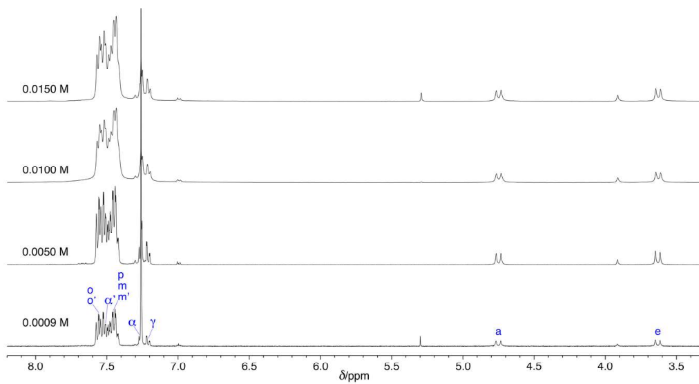
Figure 12. Variable concentration 1 H NMR (CDCl 3 , 600 MHz) of C1.
