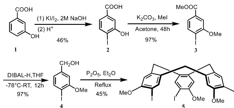
Figure 98. The synthesis route of precursor CTB 5 .
