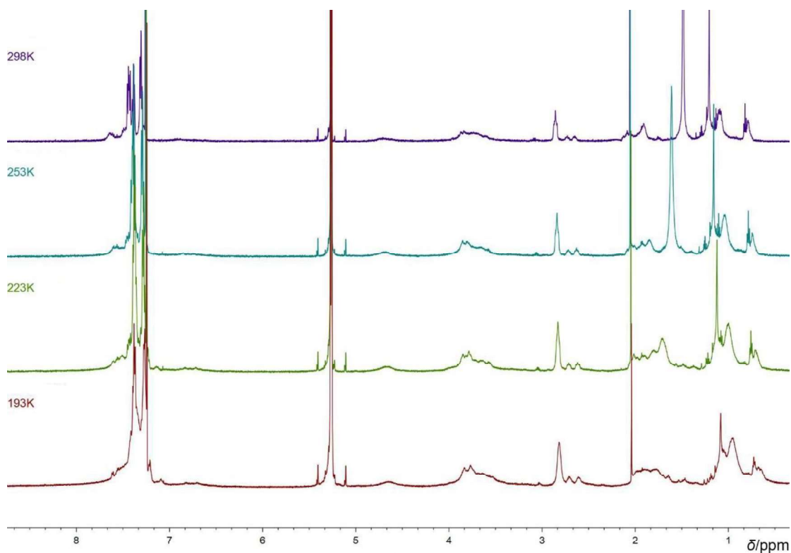
Figure 57: VT ^1\text{H} NMR spectra of compound [\text{cis-Pt}(\text{PEt}_3)_2(\text{Pd}_2(\text{dppp})_2(\text{CTB}(\text{3OMe};\text{2CN},\text{C}_2))\text{Cu}^+)(\text{OTf})_5] in \text{CD}_2\text{Cl}_2 (193-298K).
