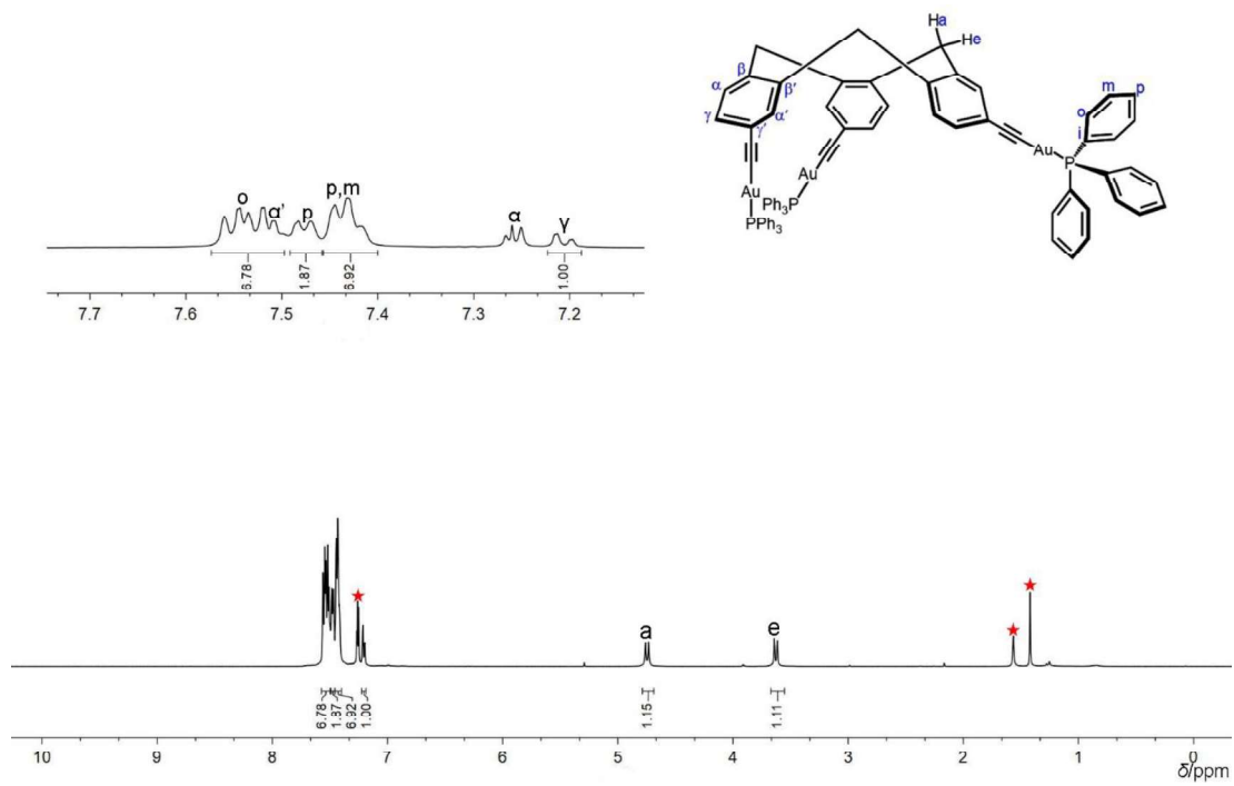
Figure 4. ^1\text{H} NMR spectrum of compound \text{CTB}(\text{H}, \text{C}_2\text{AuPPh}_3) \text{C1}
