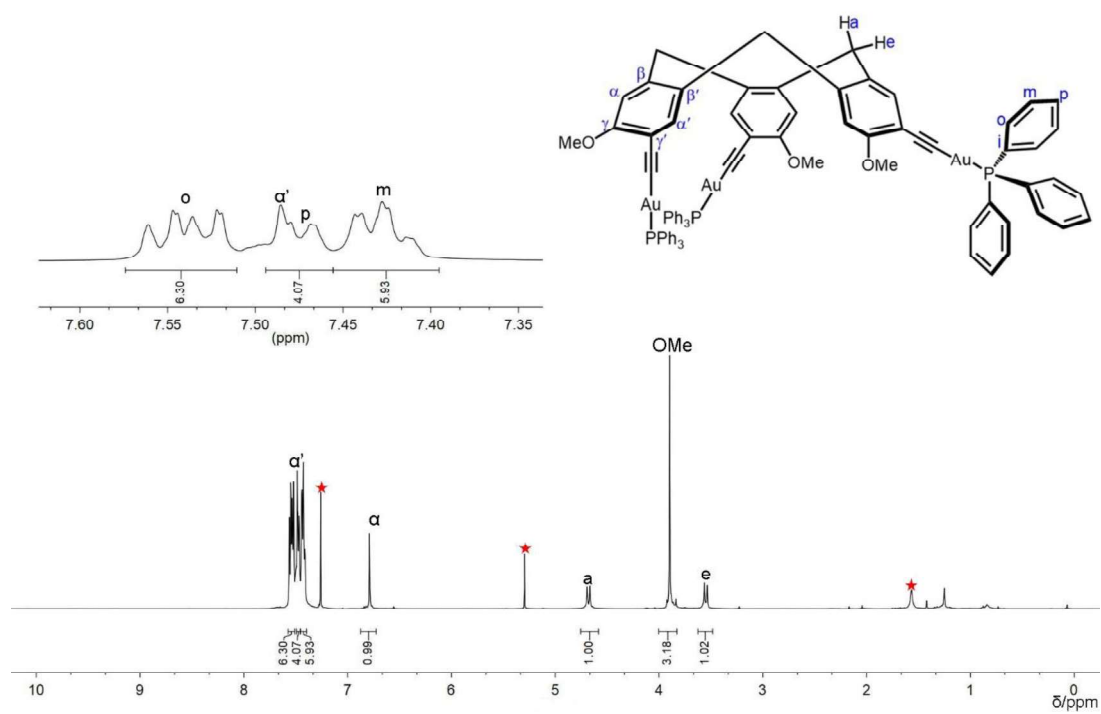
Figure 9. 1 H NMR spectrum of compound CTB(OMe,C 2 AuPPh 3 ) C4
