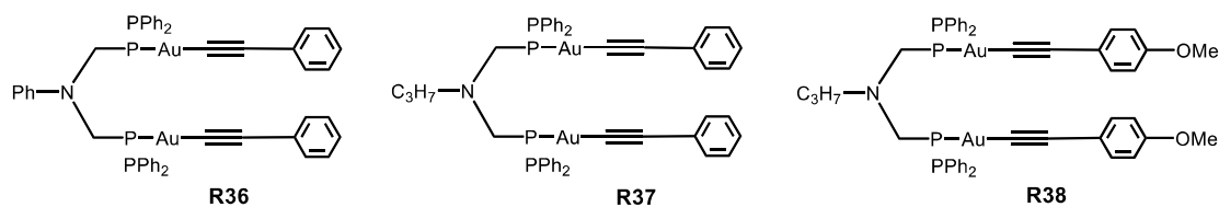
Figure 38. The structures of dinuclear gold(I) alkynyl complexes R36 , R37 and R38 .
