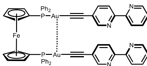
Figure 32. Structure of [(\text{bpyC}\equiv\text{CAu})_2(\mu\text{-dppf})] R32 showing the intramolecular aurophilic interactions.
