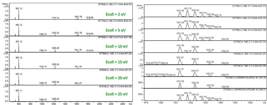
Figure 20. ESI-MS of C5, 2 \times 10^{-5} M in i -PrOH/CHCl 3 /HCO 2 H 0.495:0.495:0.010 and detail of the molecular peak.
