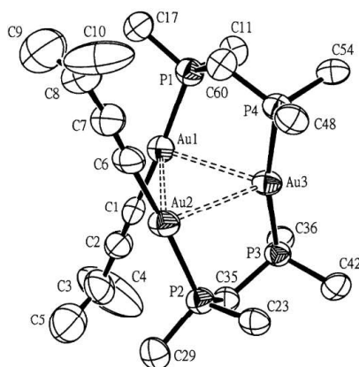
Figure 33. ORTEP view of the trinuclear cationic gold(I) complex [(\text{dppm})_2\text{Au}_3\{\text{C}\equiv\text{CC}(\text{=CH}_2)\text{Me}\}_2] (Reproduced from Ref 104 ).
