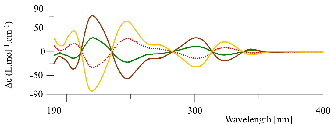
Figure 130. ECD spectra of optically pure compound 18 and saddle-out conformation 19 in acetonitrile. The red-brown and orange solid lines correspond to (-) - 18 and (+) - 18 respectively; the green solid line is the spectrum of (-) - 19 , the red dotted line, the spectrum of (+) - 19 .
