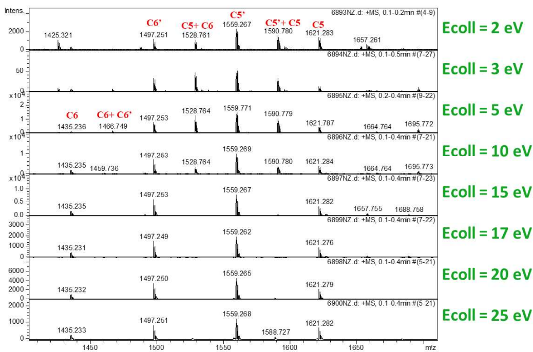
Figure 28. ESI-MS of C5 with C6, detail of the evolution of the molecular peak as a function of E_{coll} .
