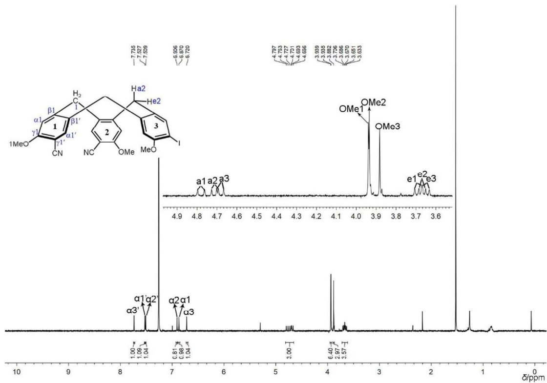
Figure 53. ^1\text{H} NMR spectrum of CTB(3OMe;2CN,I) in CDCl 3 at 298K.
