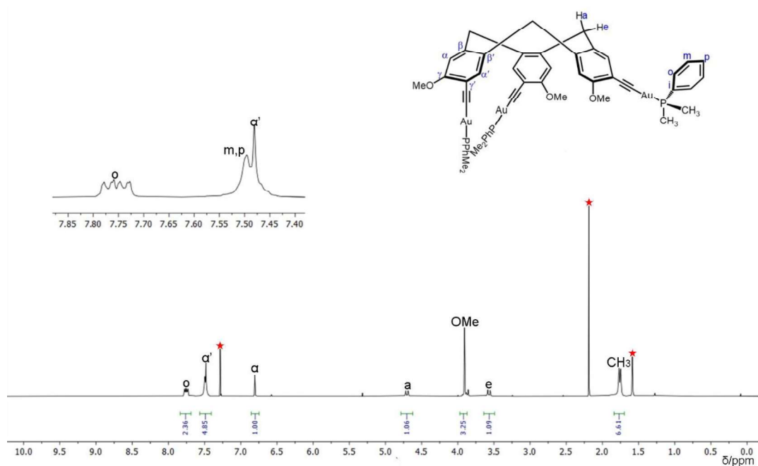
Figure 11. ^1\text{H} NMR spectrum of compound CTB(OMe,C 2 AuPPhMe 2 ) C6
