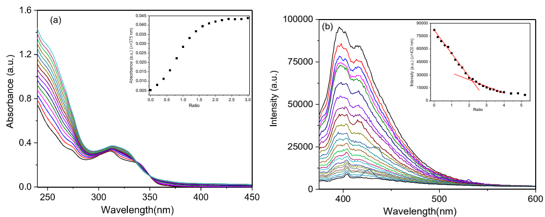
Figure 135. (a) UV-vis spectral changes of 18 ( 1.0 \times 10^{-5} mol L -1 ) in CH 2 Cl 2 upon addition of [Pt(dppp)] 2+ . (b): Emission spectral changes of 18 ( 1.0 \times 10^{-5} mol L -1 ) in CH 2 Cl 2 upon addition of [Pt(dppp)] 2+ . Inserts: plots of the absorbance and emission change at 375 nm and 420 nm as a function of the ratio [Pt(dppp)] 2+ /[ 18 ]
