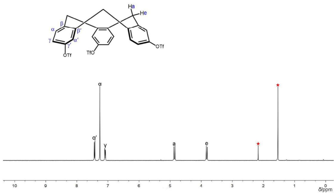
Figure 1. 1 H NMR spectrum of compound CTB(H,OTf)
