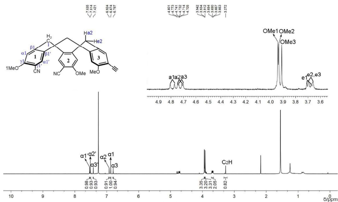
Figure 100. The ^1H NMR spectrum of CTB 9 in CDCl_3 at 298 K.
