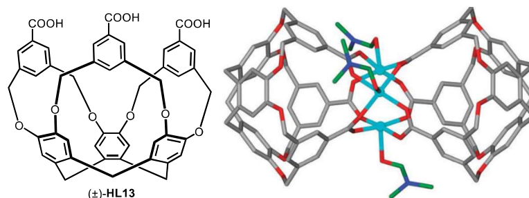
Figure 21. The structure of HL13 and the crystal structure of R14 .
