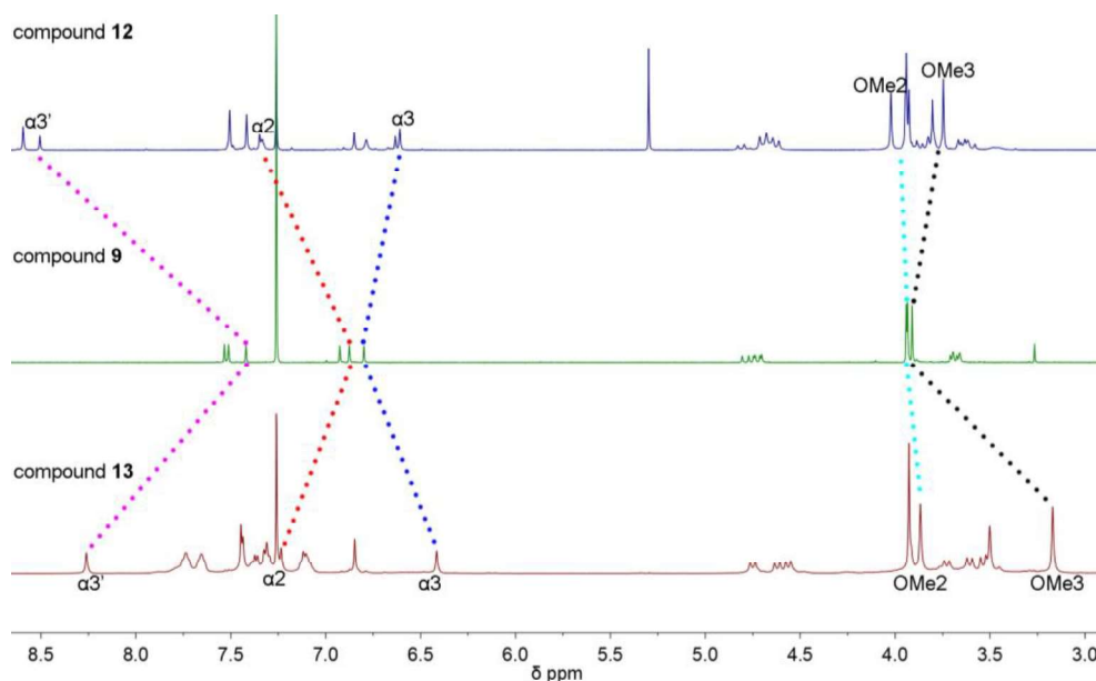
Figure 120. Stacked plots of selected regions of the ^1\text{H} NMR spectra of CTB 9 , precryptophane 12 and precryptophane 13 .
