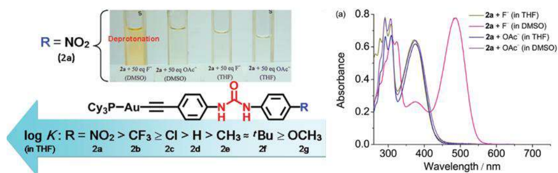
Figure 41. The recognition of F - with the naked eye and the UV-vis absorption spectra of the gold(I) acetylide complex R41 in THF or DMSO in the presence of F - and OAc - (Reproduced from Ref 112).
