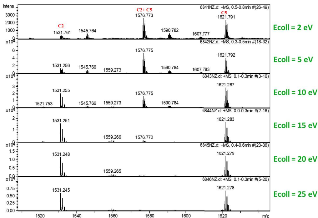
Figure 29. ESI-MS of C2 with C5, detail of the evolution of the molecular peak as a function of E_{coll} .
