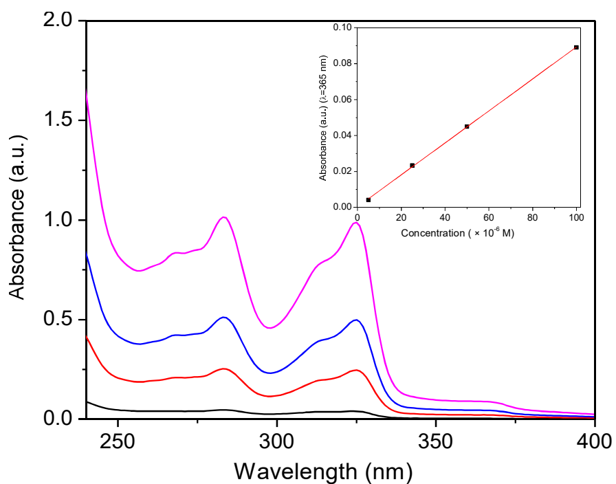
Figure 35. Electronic absorption spectra of C5 in CHCl 3 at concentrations of 5.0 to 100 × 10 -6 M. Inset: Absorbance at 365 nm vs. concentration.
