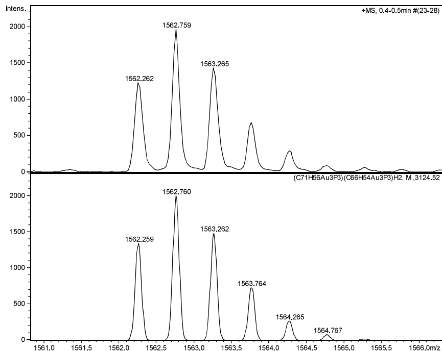
Figure 55. ESI-MS of doubly-charged dimers of composition C2 with C2': Detail of the profile of the molecular peak. The theoretical profile of [C2 + C2' + 2H]^{2+} is shown in the bottom lines.
