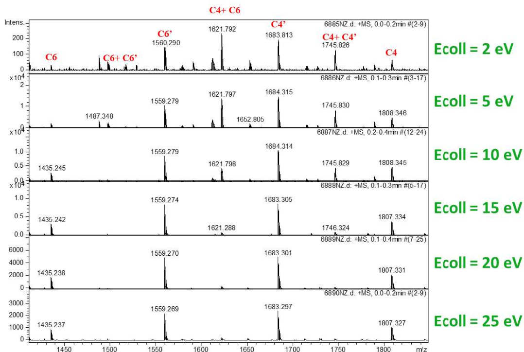
Figure 26. ESI-MS of C4 with C6, detail of the evolution of the molecular peak as a function of E_{coll} .
