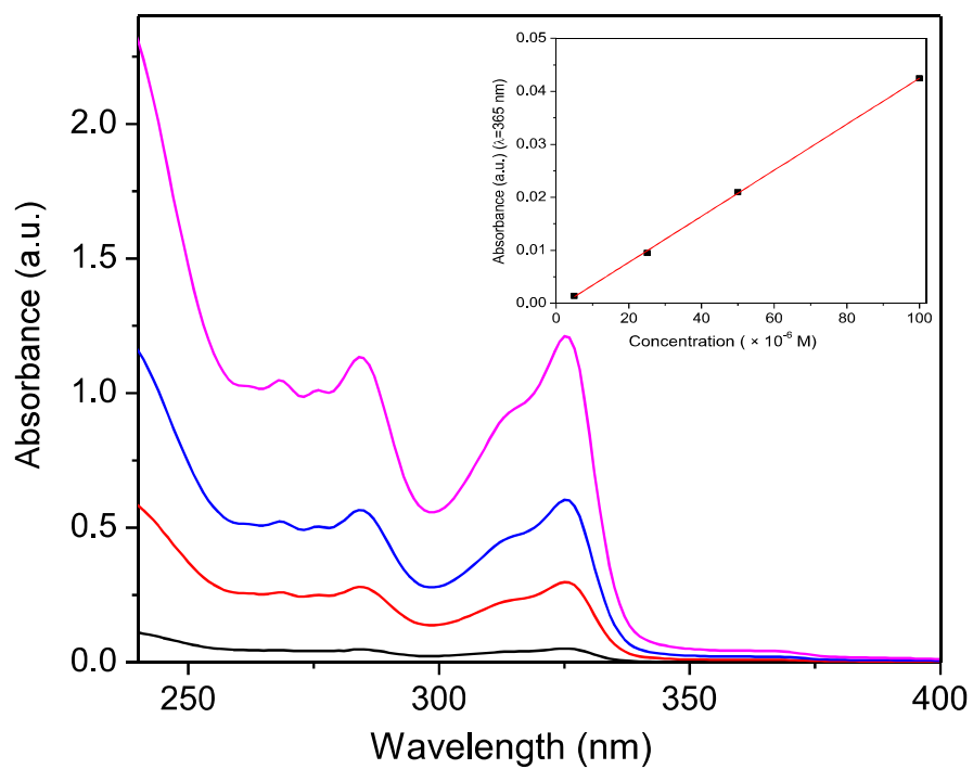
Figure 34. Electronic absorption spectra of C4 in CHCl 3 at concentrations of 5.0 to 100 × 10 -6 M. Inset: Absorbance at 365 nm vs. concentration.
