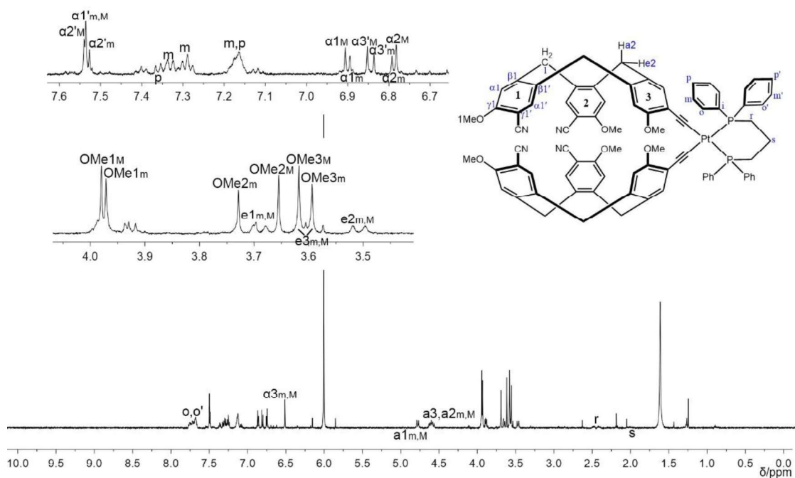
Figure 122. ^1\text{H} NMR spectrum of compound 18 in \text{C}_2\text{D}_2\text{Cl}_4 at 298 K.
