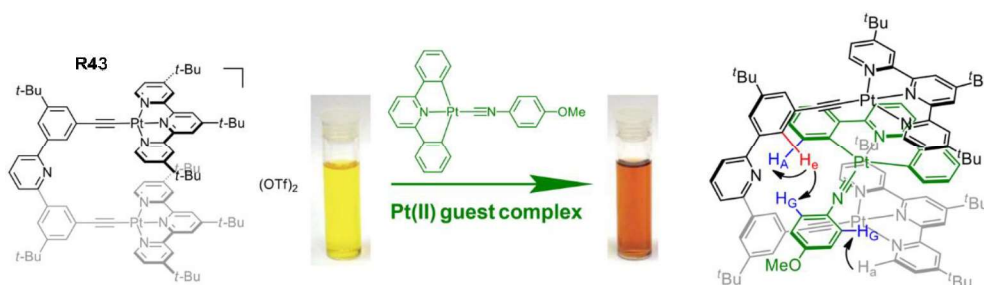
Figure 90. The host-guest association of the alkynylplatinum(II) terpyridine molecular tweezers with the platinum complex [Pt(C^N^C)(C\equiv N-C_6H_4-OMe-p)] produces a drastic color change (Reproduced from Ref [165] ).
