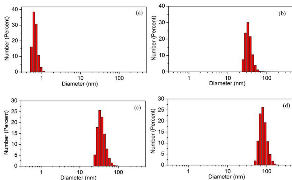
Figure 86. Nanoparticle size distribution diagrams for 10^{-5} M solutions of C1 in CHCl 3 /MeOH mixtures: (a) 80:20, (b) 50:50, (c) 20:80, and (d) 1:99.
