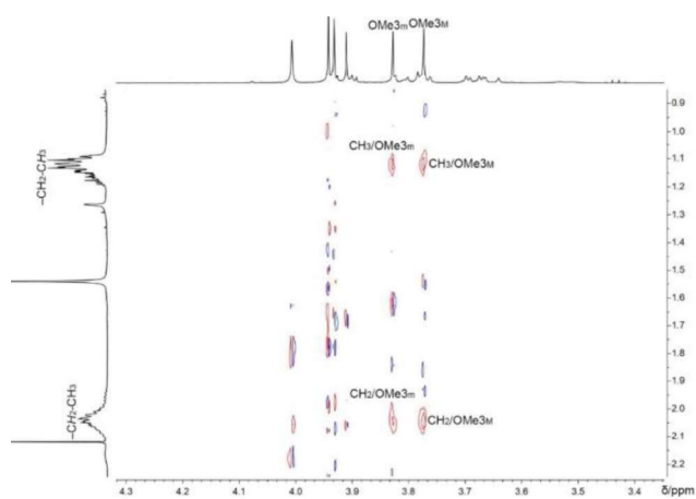
Figure 121. Detail of the ROESY map of compound 12 , showing the through space correlations between the protons of the \text{PET}_3 ancillary ligands of the platinum bridge and the protons of the -\text{OMe}_3 substituents of the CTB ligands.
