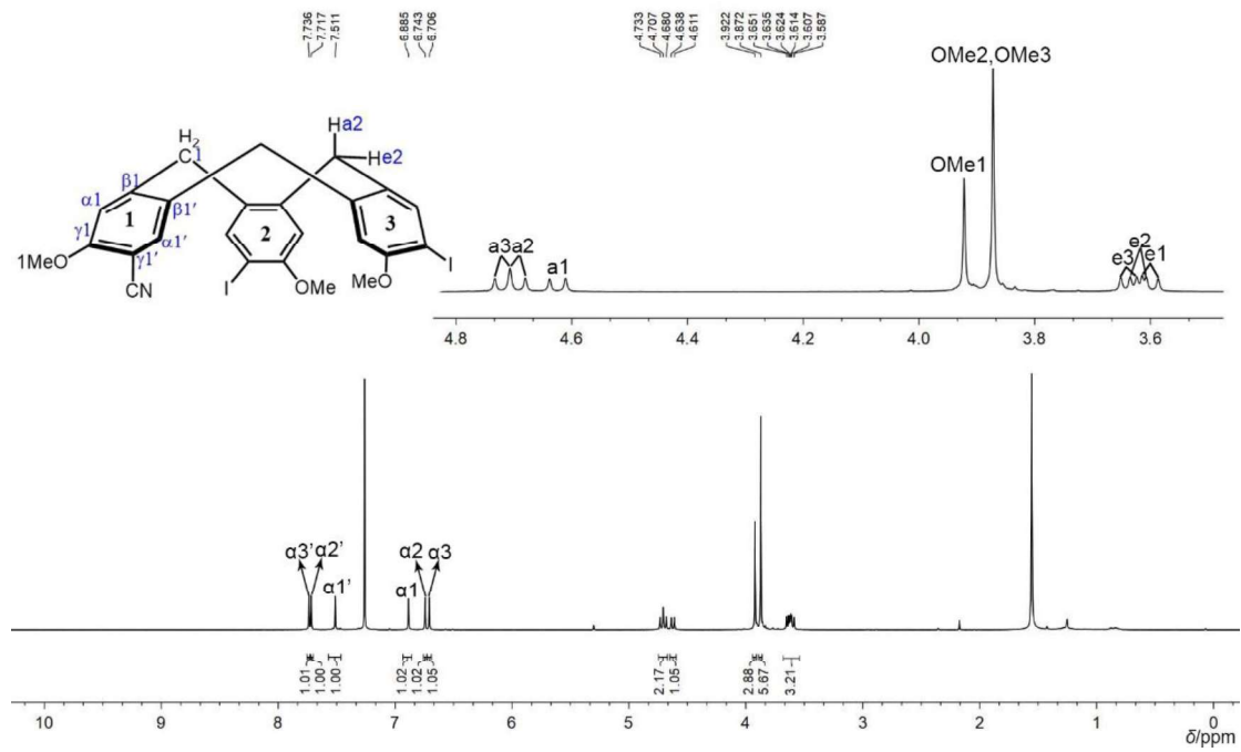
Figure 54. 1 H NMR spectrum of CTB(3OMe;CN,2I) in CDCl 3 at 298K.
