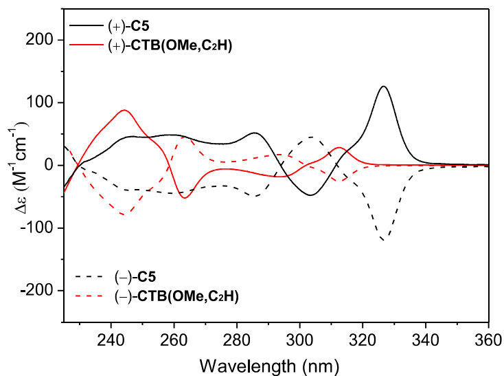
Figure 62. Superposition of the ECD spectra of the enantiomers of CTB(OMe,C 2 H) and of complex C5 in CH 2 Cl 2 . Concentrations: (–)-CTB(OMe,C 2 H): 23.8×10 -5 M; (+)-CTB(OMe,C 2 H): 25.1×10 -5 M; (–)-C5: 15.6×10 -5 M; (+)-C5: 17.5×10 -5 M.
