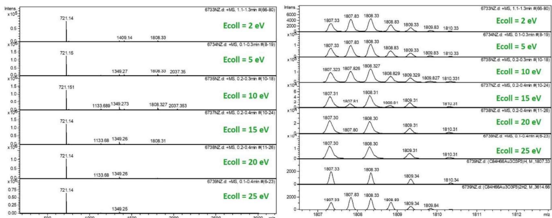
Figure 19. ESI-MS of C4, 2 \times 10^{-5} M in i -PrOH/CHCl 3 /HCO 2 H 0.495:0.495:0.010 and detail of the molecular peak.
