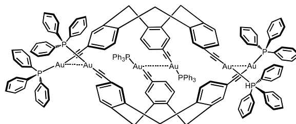
Figure 50. The dimer model of C1.
