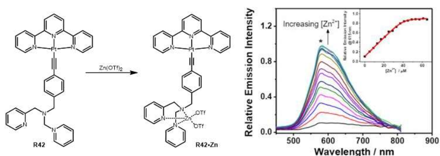
Figure 89. Host-guest association of the dipicolylamine-substituted alkynylplatinum(II) terpyridine complex with Zn^{2+} , and the corresponding luminescence change (Reproduced from Ref [164] ).
