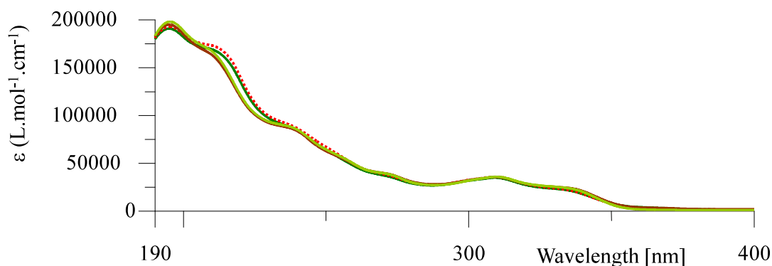
Figure 131. UV-vis absorbance spectra of optically pure compound 18 and saddle conformation 19 in acetonitrile. The red-brown and orange solid lines correspond to (-) - 18 and (+) - 18 respectively; the green solid line is the spectrum of (-) - 19 , the red dotted line, the spectrum of (+) - 19 .
