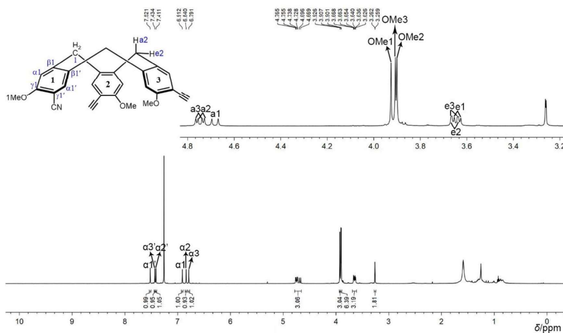
Figure 101. The ^1\text{H} NMR spectrum of CTB 11 in \text{CDCl}_3 at 298 K.
