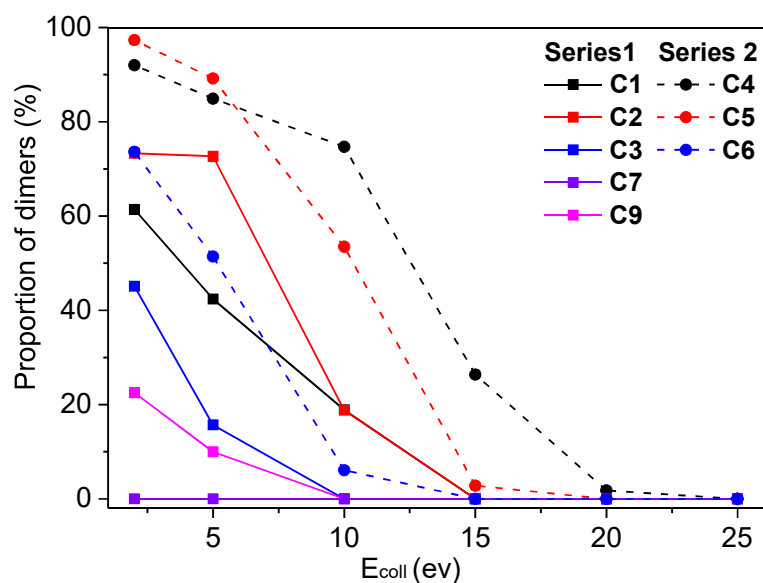
Figure 53. Plot of the proportions of dimers [\text{2M} + 2\text{H}]^{2+} in the dimer/monomer mixture for the Au(I) CTB complexes C1 – C9 , except C8 , which does not show any dimer, as C7 .
