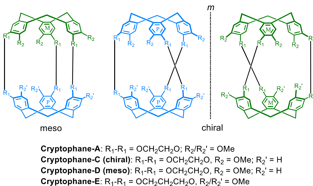
Figure 10. Schematical representations of the molecular structures of the (a) achiral syn and (b) chiral anti forms of the cryptophanes. The straight lines in black stand for organic linkers in classical cryptophanes, but they could also represent other kinds of bonds in self-assembled systems.
