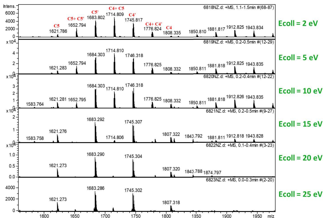
Figure 27. ESI-MS of C4 with C5, detail of the evolution of the molecular peak as a function of E_{coll} .
