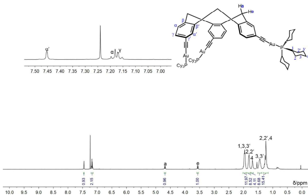
Figure 8. ^1\text{H} NMR spectrum of compound \text{CTB}(\text{H},\text{C}_2\text{AuPCy}_3) C9
