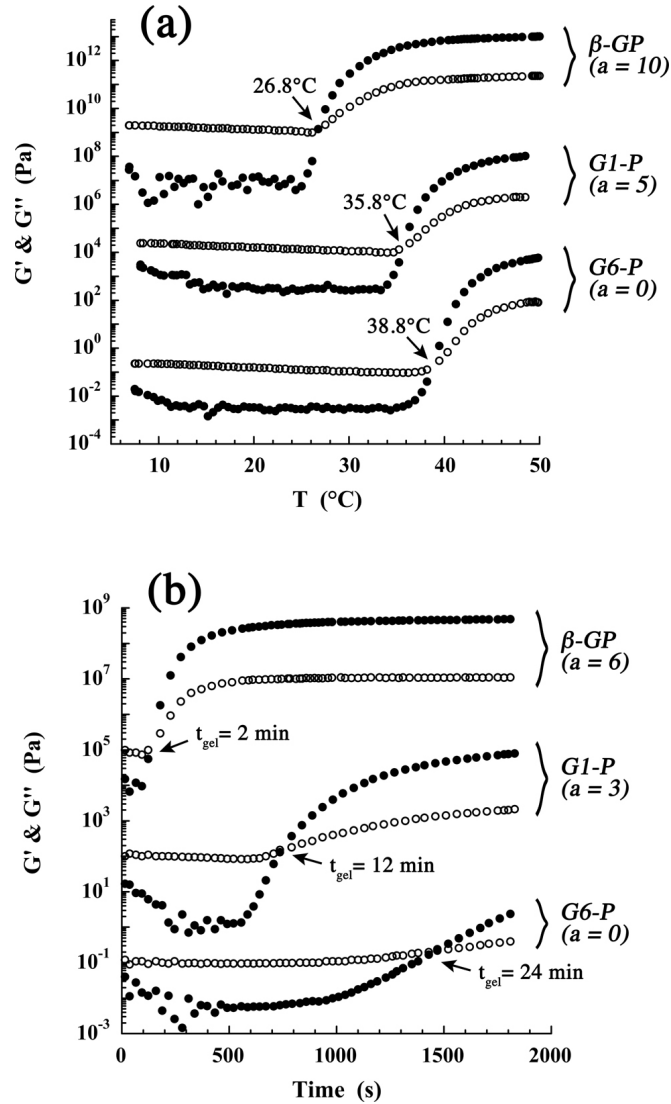
Figure II-7: (a) Temperature dependence of storage modulus ( G' , ●) and loss modulus ( G'' , ○) of CS / \beta -GP, CS / G1-P and CS / G6-P solutions for a gelling agent concentration of 0.43 mmol/g. (b) Time dependence of storage modulus ( G' , ●) and loss modulus ( G'' , ○) of CS / \beta -GP, CS / G1-P and CS / G6-P solutions for a gelling agent concentration of 0.43 mmol/g, at 37^{\circ}\text{C} . The data are shifted along the vertical axis by a factor of 10^a to avoid overlapping.
