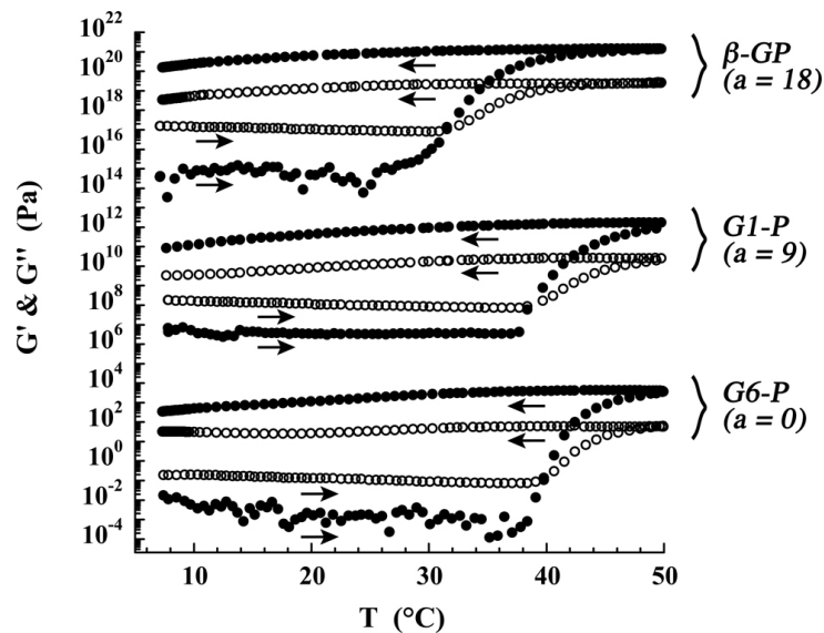
Figure II-8: Temperature dependence of storage modulus ( G' , ●) and loss modulus ( G'' , ○) of CS / \beta -GP, CS / G1-P and CS / G6-P solutions (gelling agent concentration: 0.26 mmol/g) in a heating and cooling process. The data are shifted along the vertical axis by a factor of 10^a to avoid overlapping.
