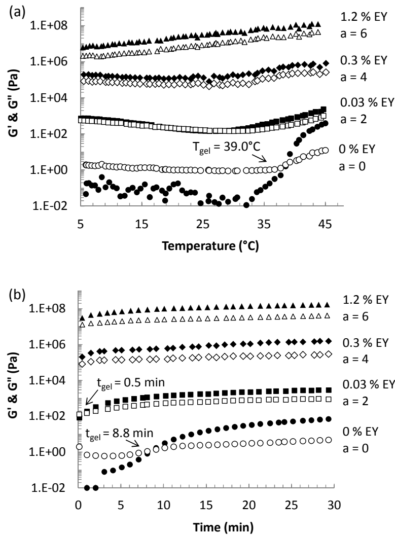
Figure IV-6: (a) Temperature and (b) time dependence at 37^{\circ}\text{C} of storage modulus ( G' , closed symbols) and loss modulus ( G'' , opened symbols) of CS / G1-P / EY solutions for EY concentrations from 0 to 1.2 wt.%. The data are shifted along the vertical axis by a factor of 10^a to avoid overlapping ( n = 1 ).
