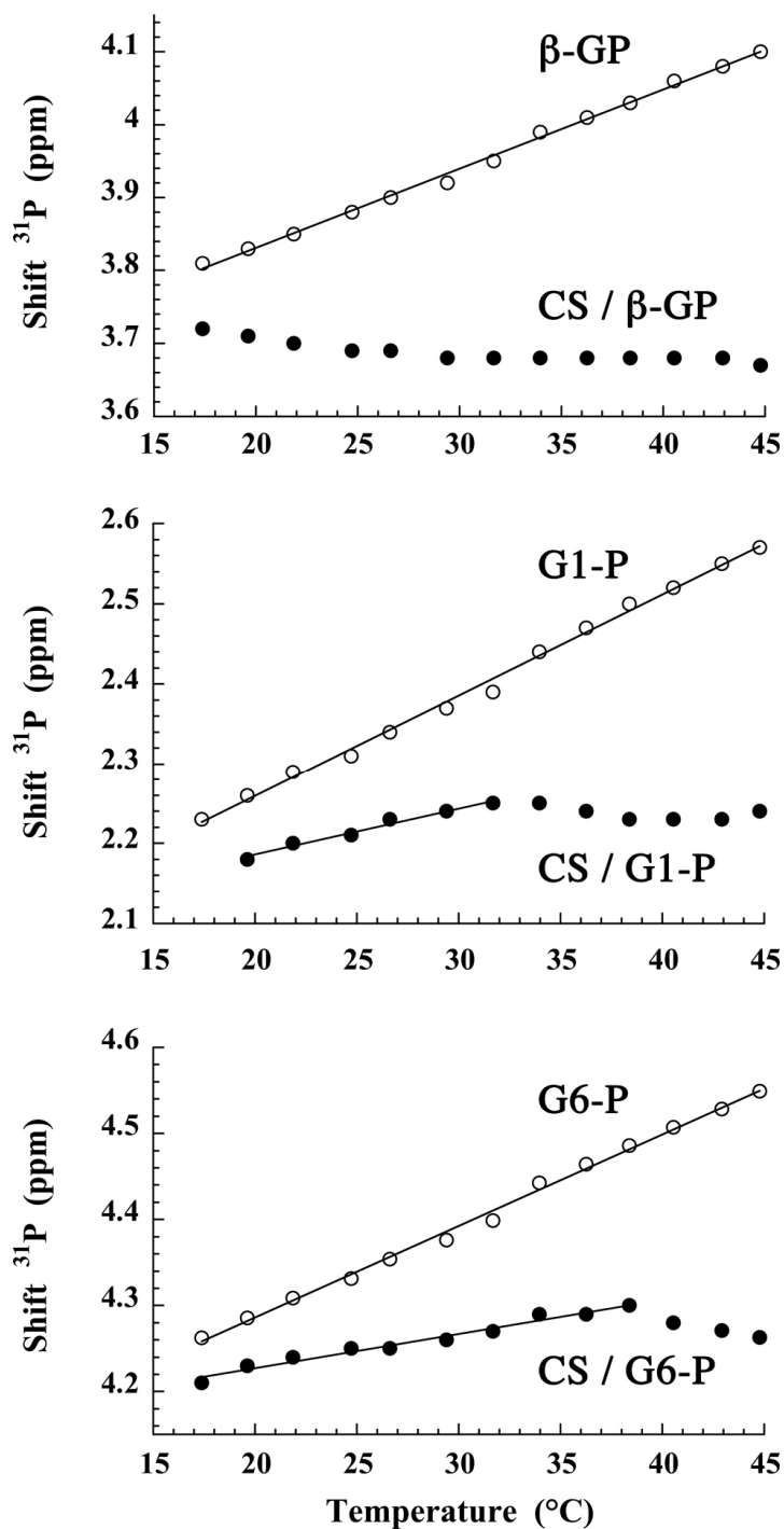
Figure II-10: Temperature dependence of the chemical shift of ^{31}\text{P} nuclei from 17 to 45 ^{\circ}\text{C} of gelling agent solutions and CS/gelling agent systems (gelling agent concentrations: 0.43 mmol/g).
