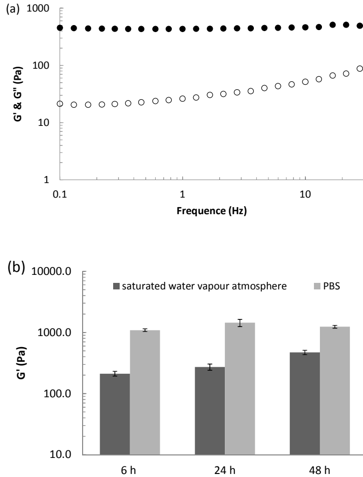
Figure III-4: (a) Frequency dependence of storage modulus ( G' , ●) and loss modulus ( G'' , ○) of CS / G1-P hydrogel (1.5 wt.% CS and 0.40 mmol/g G1-P) after 6 h in a saturated water vapor atmosphere at 37°C. (b) Strength of CS / G1-P hydrogels (1.5 wt.% CS and 0.27 mmol/g G1-P) after 6 h, 24 h and 48 h incubation either in a saturated water vapor atmosphere or in PBS at 37°C ( n = 3 ).
