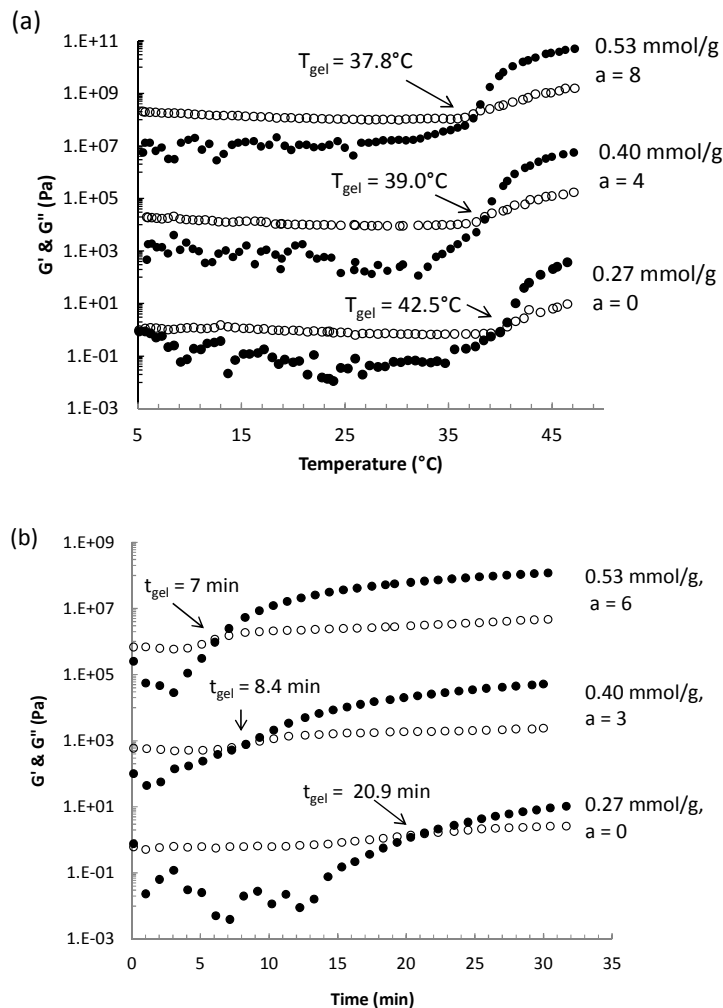
Figure III-2: (a) Temperature and (b) time dependence at 37°C of storage modulus ( G' , ●) and loss modulus ( G'' , ○) of CS / G1-P solutions (1.5 wt.% CS) for G1-P concentrations ranging from 0.27 to 0.53 mmol/g. The data are shifted along the vertical axis by a factor of 10^a to avoid overlapping ( n = 3 ).
