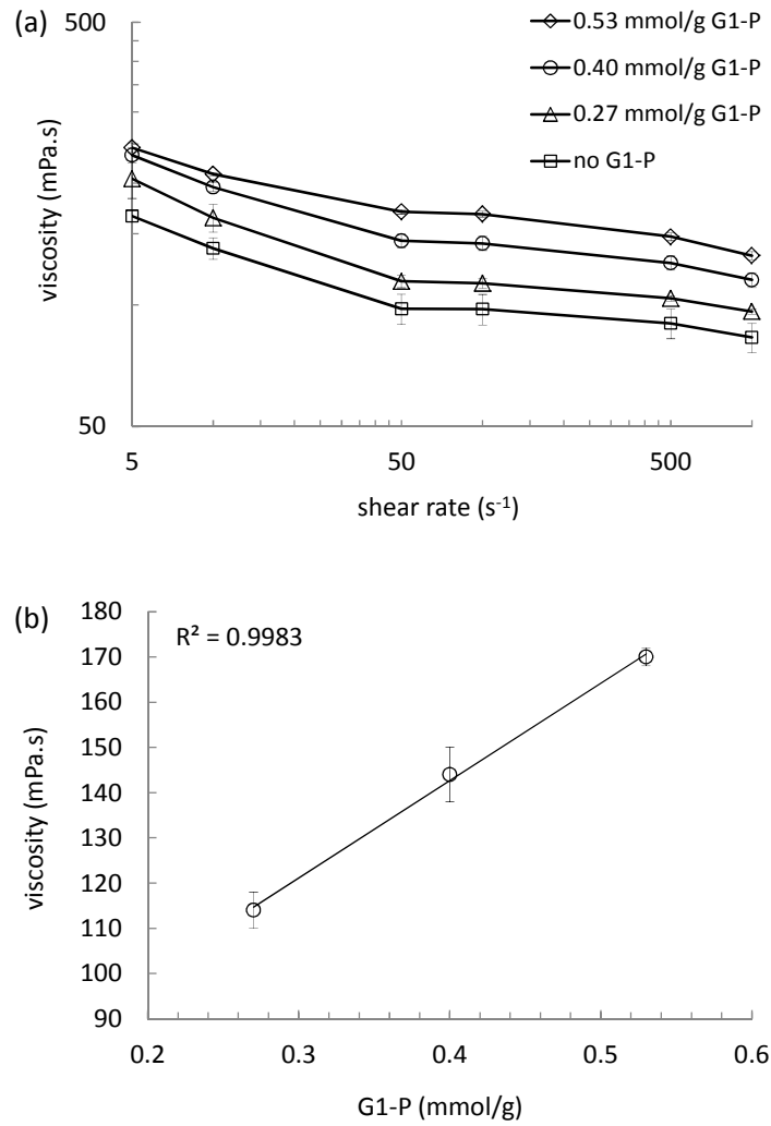
Figure III-1: Influence of G1-P concentration on apparent shear viscosities of 1.5 wt.% CS solution over a step test (a) and at a shear rate of 50 \text{ s}^{-1} (b) for G1-P concentrations ranging from 0.27 to 0.53 mmol/g ( n = 3 ).
