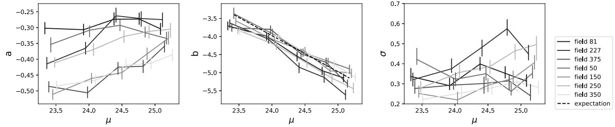
Figure IV.9: Changes to the best parameters of the recovery fraction model as a function of the distance modulus to the dwarf galaxy. Each point is slightly shifted in distance, in order to make the graph more legible. The black dashed line represents the theoretical change of M_V in function of the distance modulus for the field 50. Parameters a and b smoothly change with distance, which allows us to easily model the influence of the distance on the recovery fractions.
