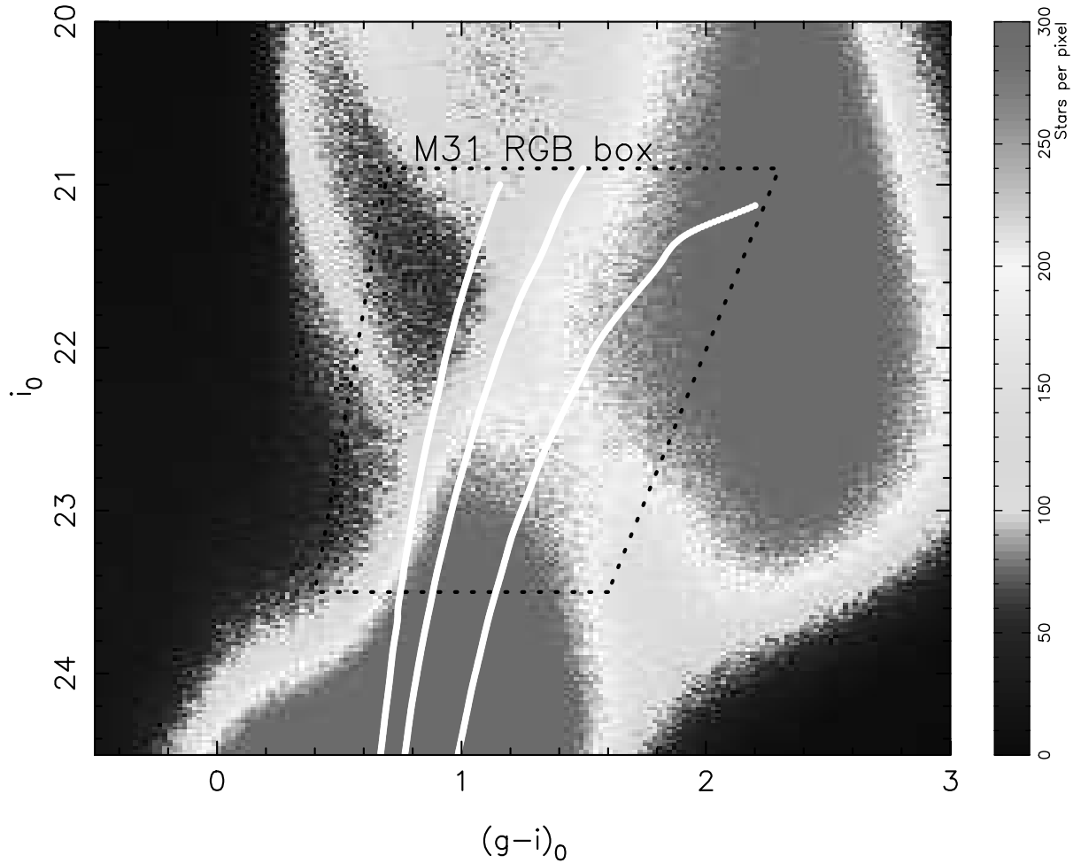
Figure III.1: CMD of all non-masked stellar sources in the PAndAS survey (i.e., located away from the crowded regions around M31 and its brightest satellites). The color gradient indicates the density of stars. Overlaid are the isochrones (Marigo et al., 2008) of stellar populations at the distance of M31, with ages of 13 Gyr and [\text{Fe}/\text{H}] of -2.3 , -1.4 and -0.7 dex (from left to right). To target old, metal poor stars a selection box denoted by a black dotted line is used. Figure credit: Martin et al. (2013a).
