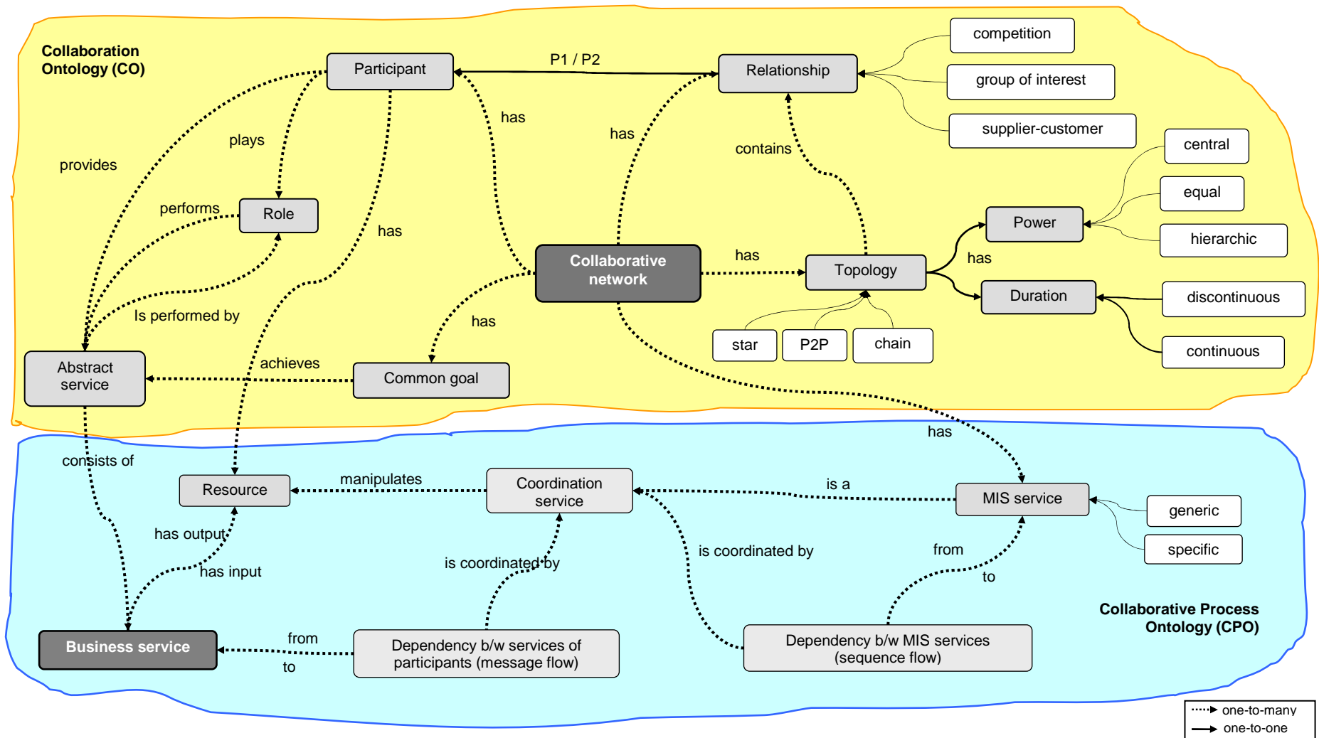
Fig.III. 8 CNO composed of Collaboration and Collaborative process ontologies
