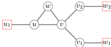
Figure 10.6. u and v share a 2-neighbor
