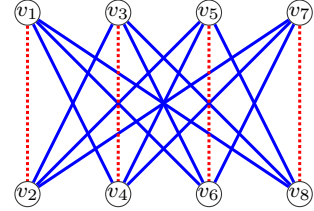
Figure 3.13. (K_{4,4}, M)
