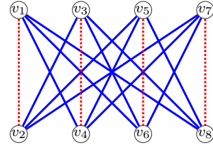
Figure 3.13. (K_{4,4}, M)
