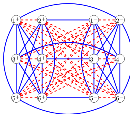
Figure 10.2. \text{DSG}(K_6, M)
