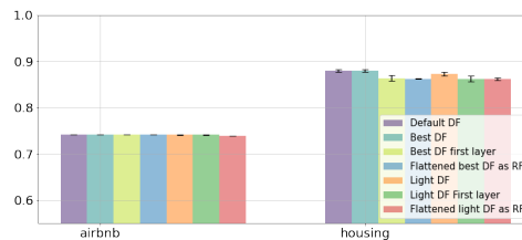
Figure 2.3: R^2 score of different DF architectures for regression datasets (10 runs per bar plot).
