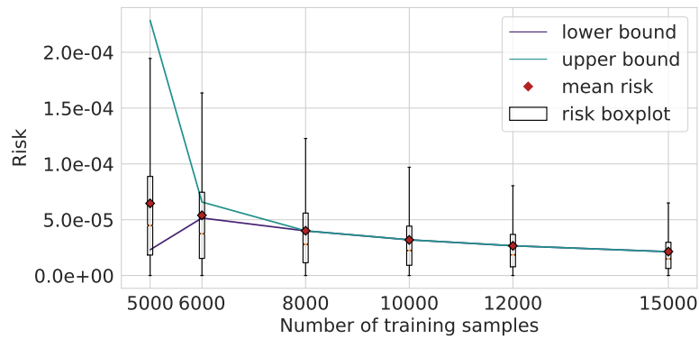
Figure S40: Illustration of the theoretical bounds for a shallow tree network of Proposition 2.4.6 2. for a chessboard with parameters k^* = 4 , N_B = 2^{k^* - 1} and p = 0.8 . The first-layer tree is of depth k = 6 . We draw a sample of size n (x-axis), and a single tree f_{k,0,n} is fitted for which the theoretical risk is evaluated. Each boxplot is built out of 20 000 repetitions. The outliers are not shown for the sake of presentation. Note that in such a case, the theoretical lower bound is constant and equal to the bias term.
