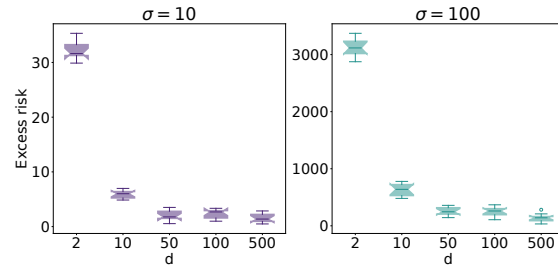
Figure S13: Decrease of the variance of an interpolating Breiman RF with \text{max-features}=\lfloor d/3 \rfloor w.r.t. dimension d . 10 repetitions per boxplot, 5000 training points and 50000 testing points were used for each repetition. The Breiman RF contains 1000 trees.
