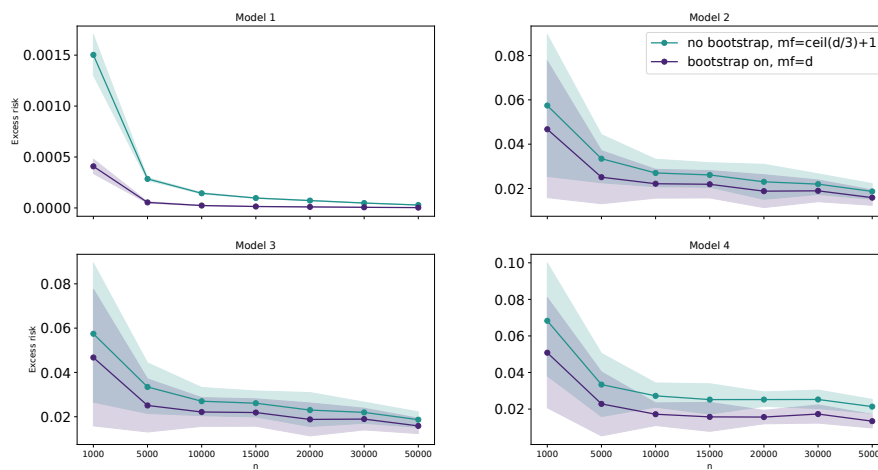
Figure 4.2: Consistency of two Breiman RF: excess risk w.r.t. sample size n . Mean over 10 tries (bold lines) and mean \pm std (filled zone), when using 2000 trees per forest, and max-depth =None. See Appendix S3 for the model definitions.
