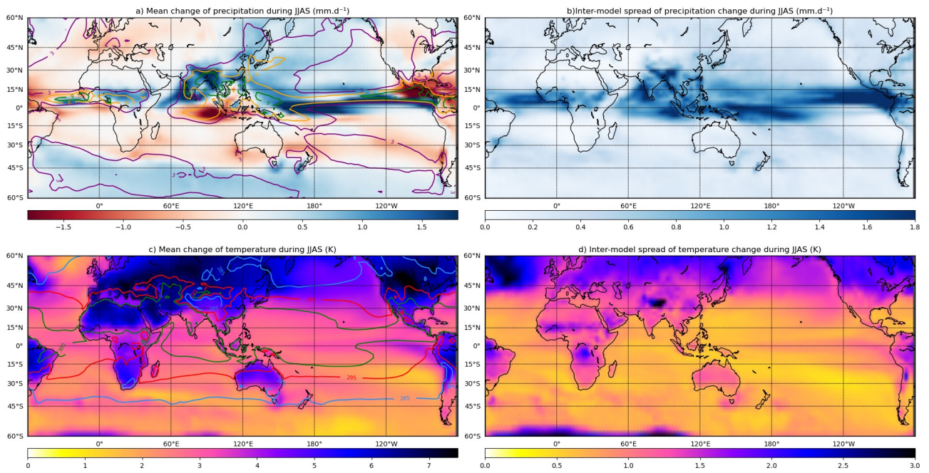
Fig.S2: same as Fig.2 but without the scaling by global temperature change.
