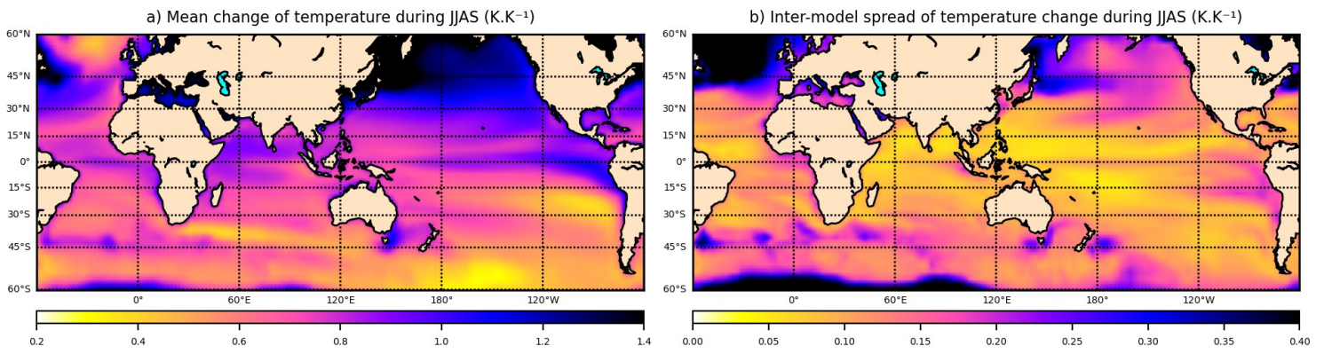
Fig. S1. (a) MMM temperature change ( K.K^{-1} ), (b) inter-model spread of temperature change ( K.K^{-1} ), during JJAS and ocean-only. Computed for the 32 CMIP6 models.
