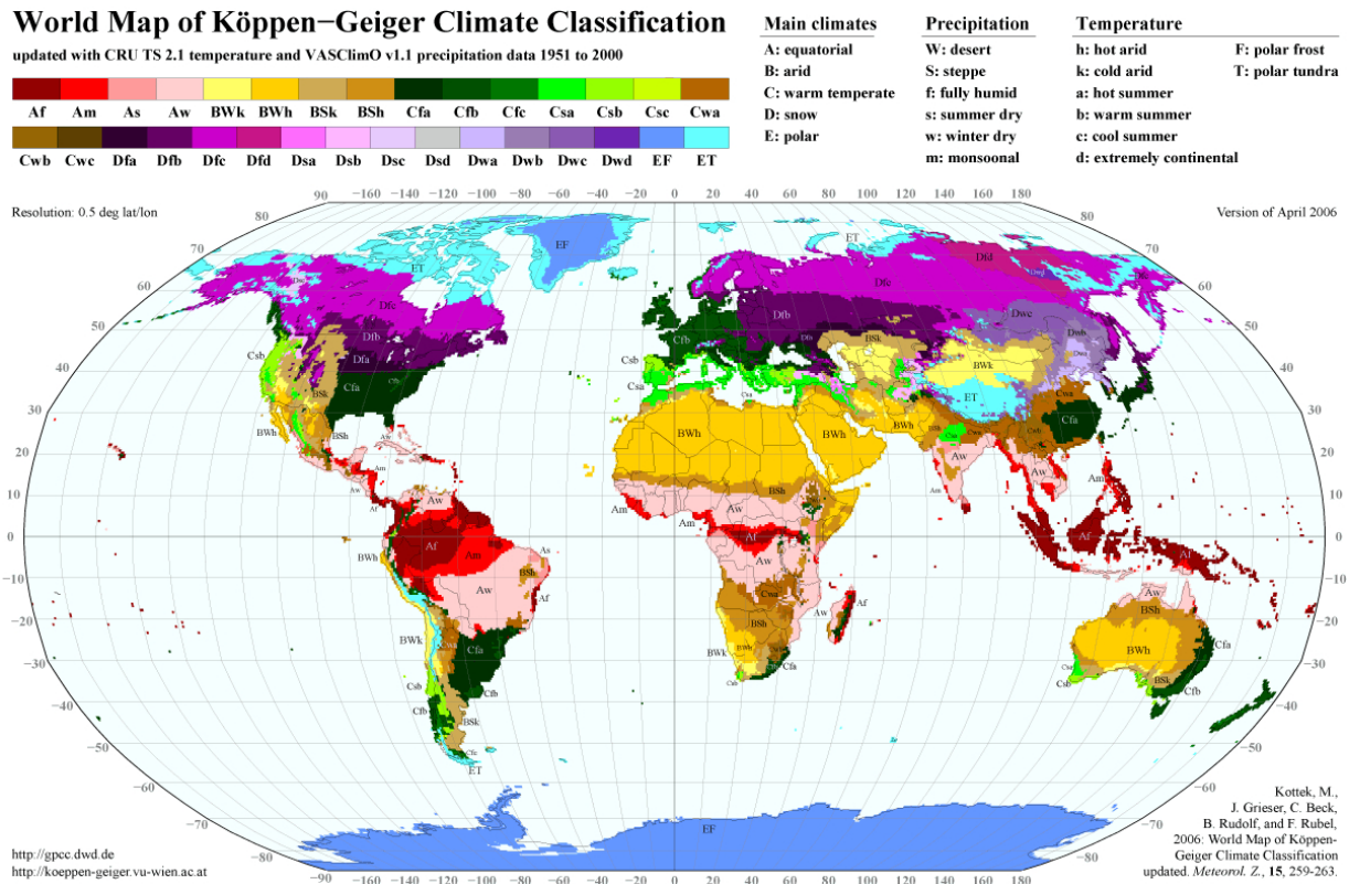
Figure 1.1: World map of Köppen climate classification (Kottek et al, 2006).
