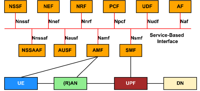
Fig. 2. 5G Service-Based Architecture.
