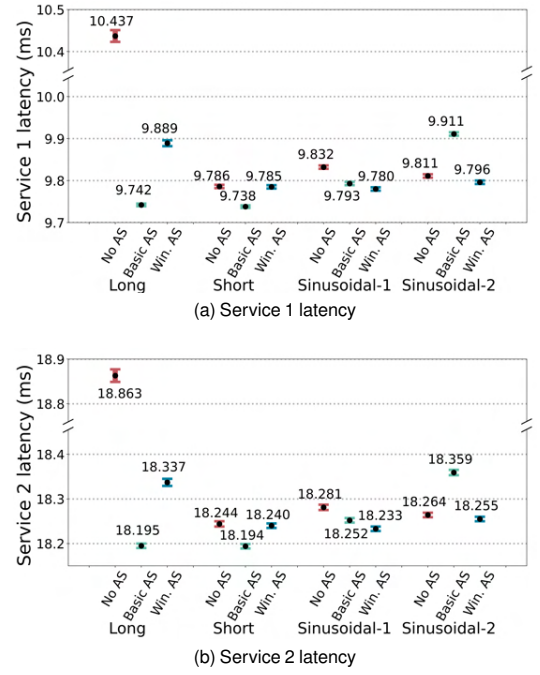
Fig. 13. Service 1 (a) and Service 2 (b) latency values and confidential intervals in case 1.
