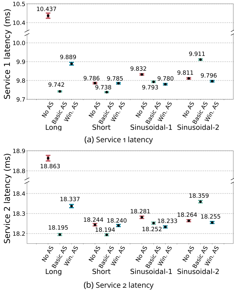
Figure 4.12: Service 1 (a) and Service 2 (b) latency values and confidential intervals in under different traffic. Figure from Paper V [26].
