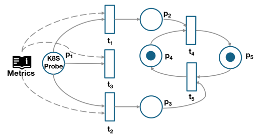
Figure 3. Petri Net of autoscaling process.
