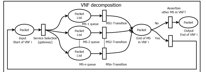
Fig. 3. Petri Net of VNF decomposition.
