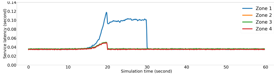
Figure 4.20: Network service latency of users from different zones. Figure from Paper IV [25].
