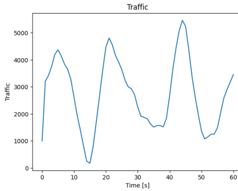
Figure B.8: Packet arrival rate of traffic pattern 3: a sinusoidal traffic variation.
