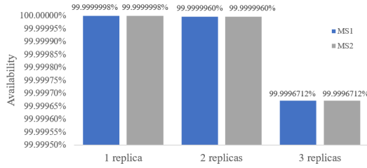
Fig. 6. Microservice availability with immediate detection.
