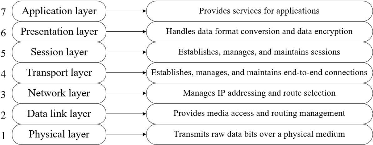
Figure 5.1 Open System Interconnection (OSI) model
