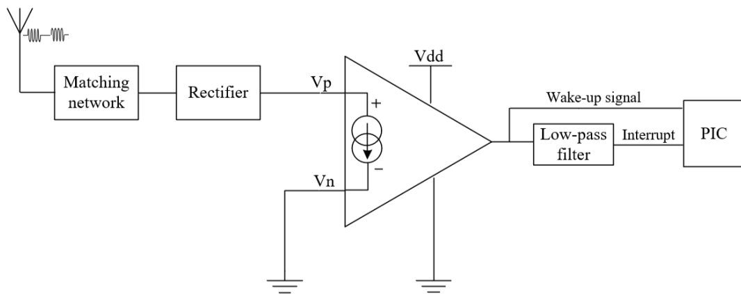
Figure 6.1 Block diagram of wake-up radio with comparator cathode grounded (Gnd as the reference)
