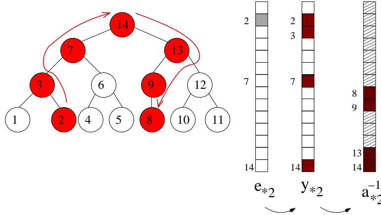
Figure 8.14: Illustration of tree traversal to compute a_{8,2}^{-1} . a_{*,2}^{-1} corresponds to column 2 of A^{-1} . Filled entries in a_{*,2}^{-1} correspond to entries in column 2 of A^{-1} while computing a_{8,2}^{-1} . a_{8,2}^{-1} = (U^{-1}L^{-1}e_2)_{i=8} ; y_2 = L^{-1}e_2 ; a_{8,2}^{-1} = (U^{-1}y_2)_{i=8} ;
