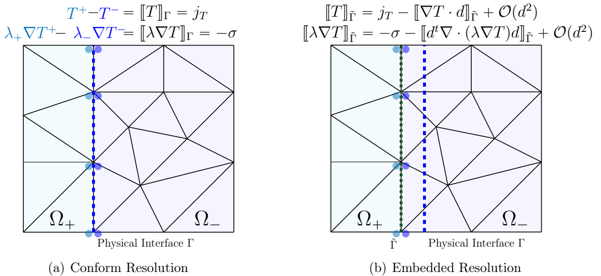
Figure 2.2: Set 1 : Visualization of the imposition of the boundary conditions
