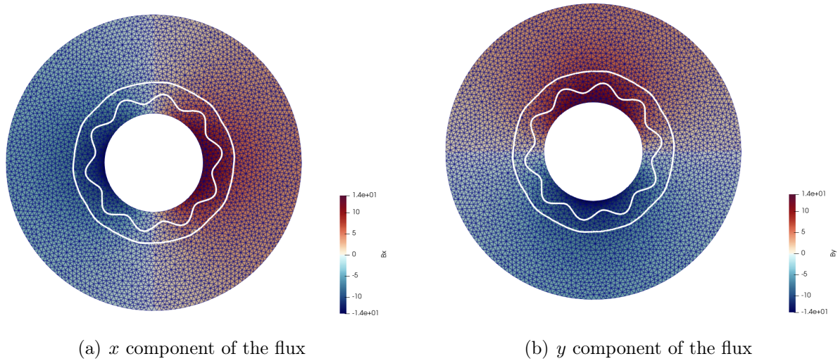
Figure 4.28: Profile of the flux and the interface position at initialization and after 600 iterations
