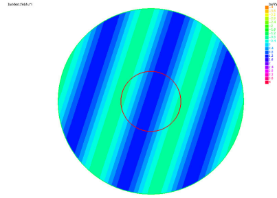
Figure 2.2: Incident field u^i .
