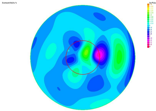
Figure 3.4: Scattered field u_{A,q}^s(\cdot, d)
