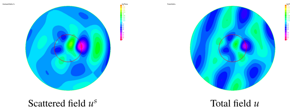
Figure 2.4: The case for A = 2.5(-\sin(\theta), \cos(\theta)) in D where \theta \in (0, 2\pi) and A = 0 outside D ( \operatorname{div}(A) = 0 in \mathbb{R}^3 ).
