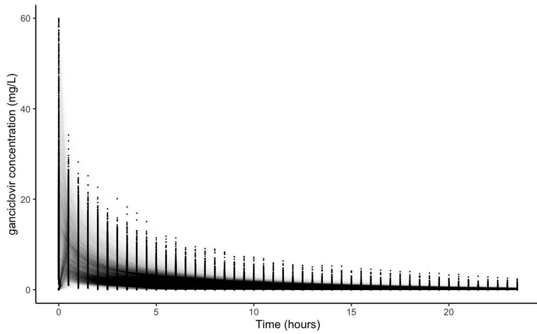
Supplemental Figure B : Spaghetti plot representing ganciclovir concentration vs time in the simulation dataset for intravenous GCV
