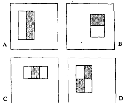
Figure 2.2: Example rectangle features shown relative to the enclosing detection window. The sum of the pixels which lie within the white rectangles are subtracted from the sum of pixels in the gray rectangles. From (Viola & Jones, 2001).
