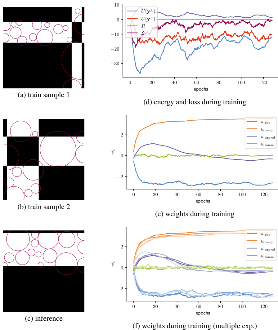
Figure 6.1: Example of contrastive divergence for training. (a) and (b) show two training samples, a synthetic image with configuration of circles in lilac. (c) shows a configuration inferred from the model using the estimated parameters. In (d) we plot the loss and its components (see (5.29)) through the estimation procedure steps. (e) shows the weights value through the estimation procedure, as in (f) where we compare over multiple random initialization.
