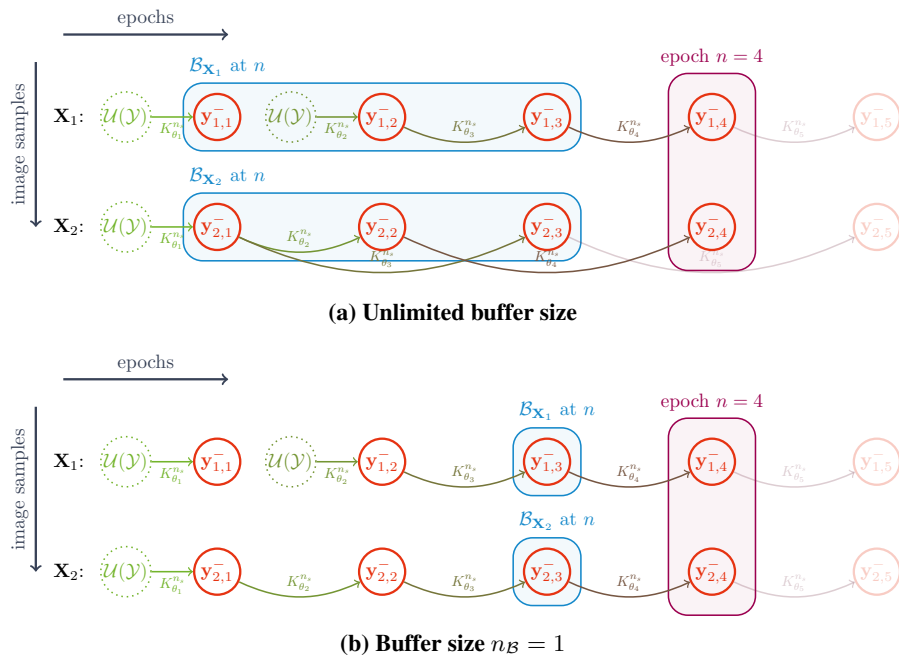
Figure 5.5: Buffer size effect on contrastive samples. Buffers are represented in blue. In this example the Markov chain starts from \mathbf{y}_{\cdot,0} \sim \mathcal{U}(\mathcal{Y}) , thus the unlimited buffer is only of size 3 at epoch n = 4 . Configuration \mathbf{y}_{k,n}^- corresponds to contrastive sample for image \mathbf{X}_k at epoch n , and K_{\theta_n}^{n_s} is the application of the transition kernel of the RJMCMC n_s times with parameters \theta_n .
