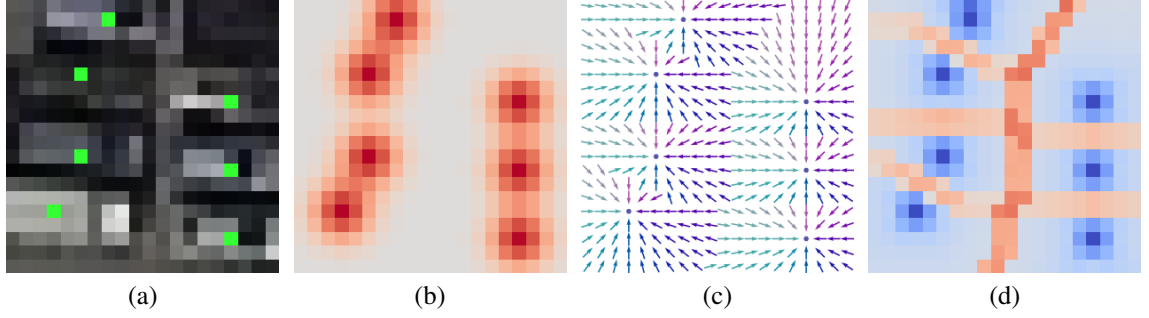
Figure 4.8: (a) Closeup image with centers overlay; (b) centers heatmap \mathbf{H} ; (c) vector field \mathbf{H}_\nabla ; (d) divergence. For (b) and (d): red > 0 , blue < 0 .
