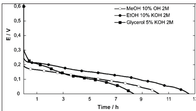
Figure 20: Galvanostatic traces of DAFCs fuelled with methanol, ethanol or glycerol oxidation at 102 mA
