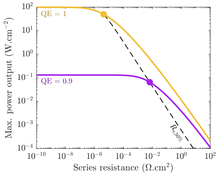
Figure 3.7: Impact of series resistance on maximum power output in the two cases considered in Section 3.3.1.2.
