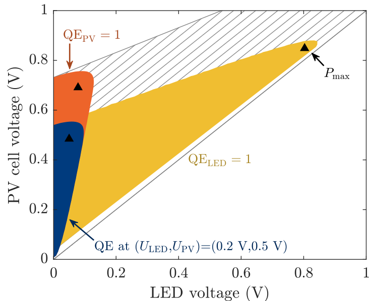
Figure 5.20: Power production region obtained with the detailed-balance model, for different QEs. The hatched region corresponds to the heat engine operating region obtained at the radiative limit in 3.3.1.1.
