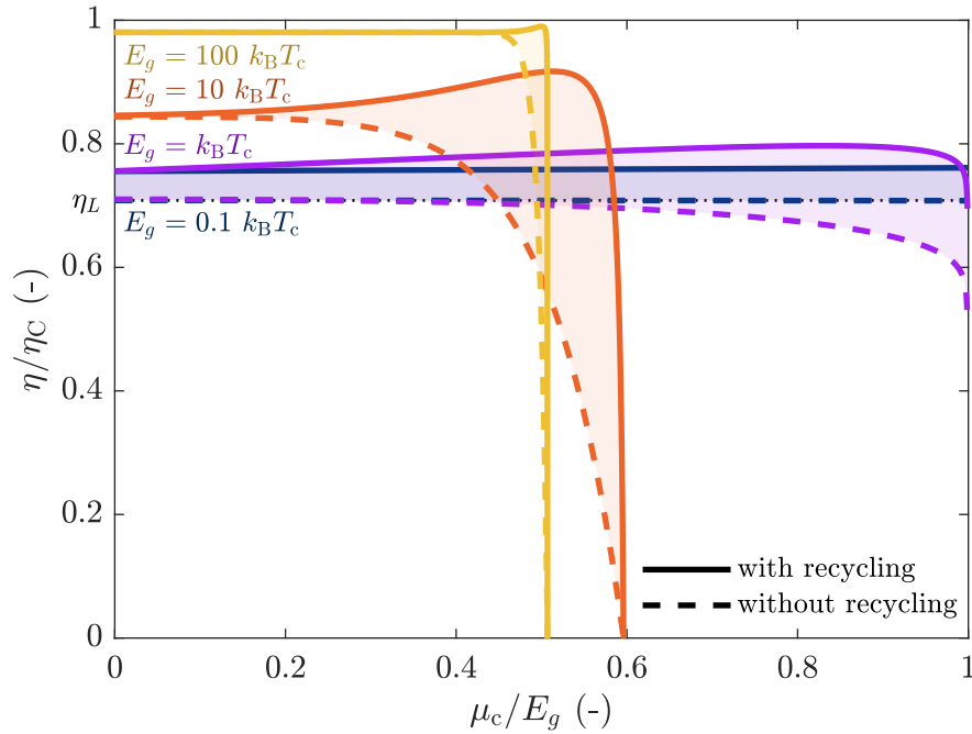
Figure 2.2: Variation of efficiency with chemical potential of radiation emitted by the cold absorber, obtained for T_h = 600 K and T_c = 300 K and for complete above- E_g radiation.
