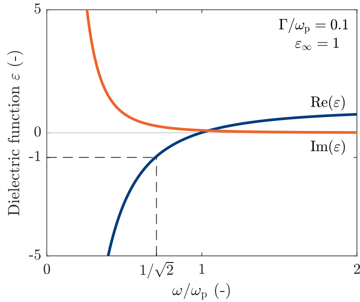
Figure 1.10: Typical dielectric function obtained with a Drude model for the plasmonic contribution.
