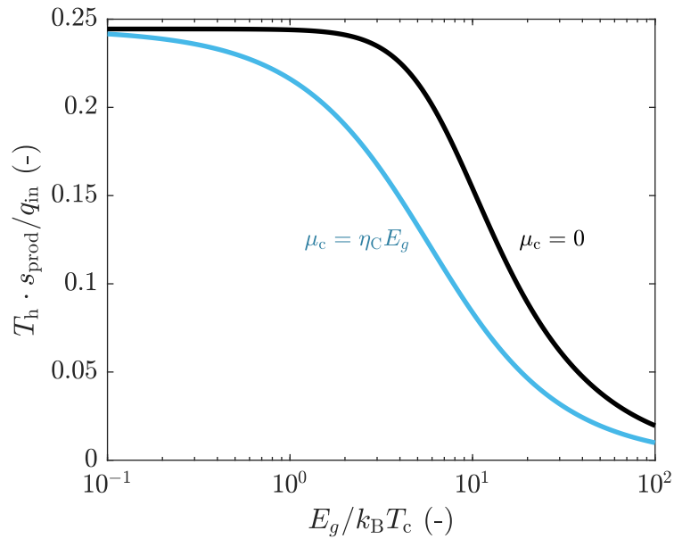
Figure 2.3: Entropy production in the passive emitter, normalised by the entropy flux coming from the heat source, as a function of the cut-off energy. The results are obtained for T_h = 600 K and T_c = 300 K.
