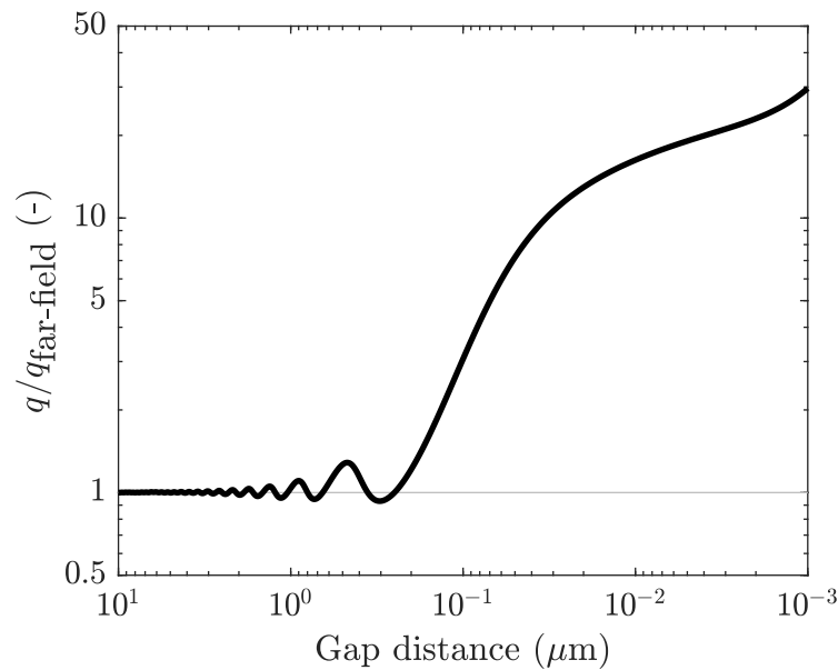
Figure 1.7: Typical variation of the heat flux with the gap distance, given with respect to the far-field value.
