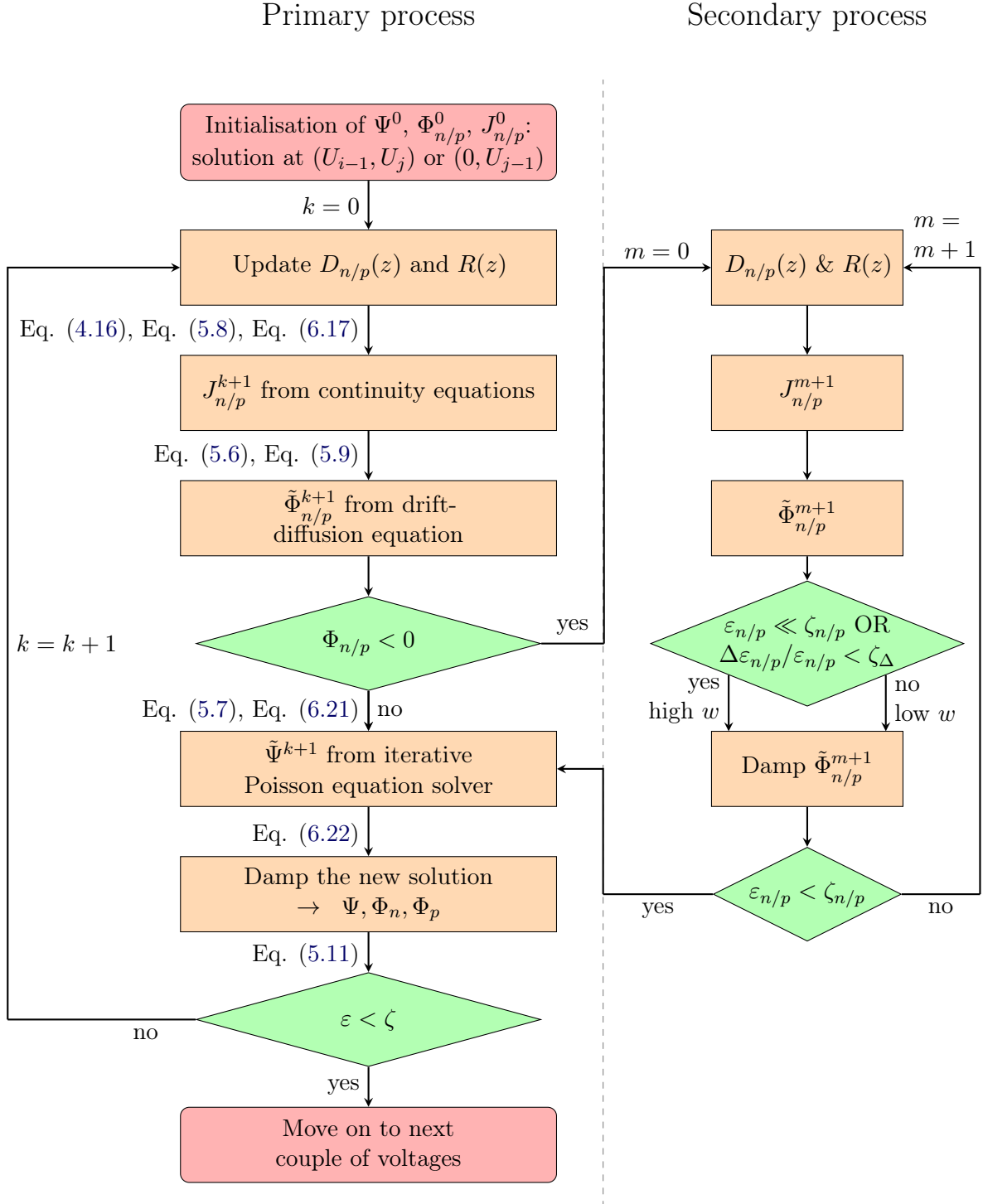
Figure 6.5: Flowchart of the drift-diffusion solver for heterostructures at (U_{\text{LED}}, U_{\text{PV}}) = (U_i, U_j) .
