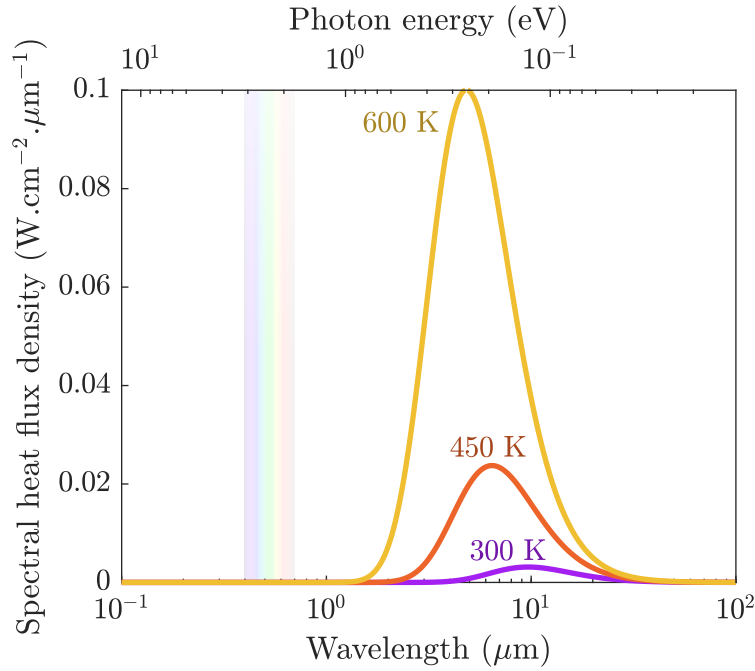
Figure 1.1: Blackbody spectrum obtained with Planck's law of radiation for different temperatures.
