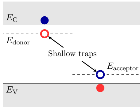
Figure 4.1: Impact of doping on the charge distribution (left: donor atom, right: acceptor atom).
