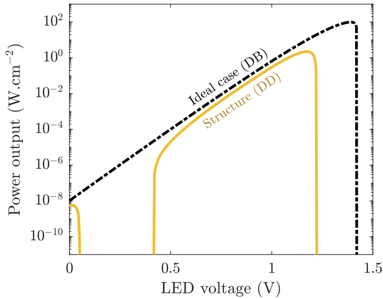
Figure 5.7: P- V_{LED} characteristic of the AlGaAs-GaAs homostructure.
