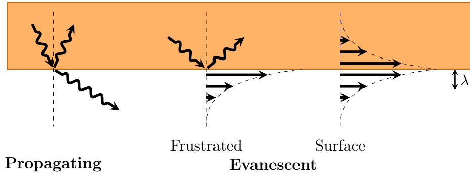
Figure 1.8: Radiation modes occurring around an interface between vacuum and a body with higher refractive index.
