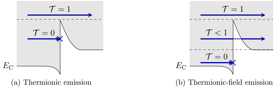
Figure 6.2: Transmission coefficient of charge carriers (here, electrons) through a heterojunction.
