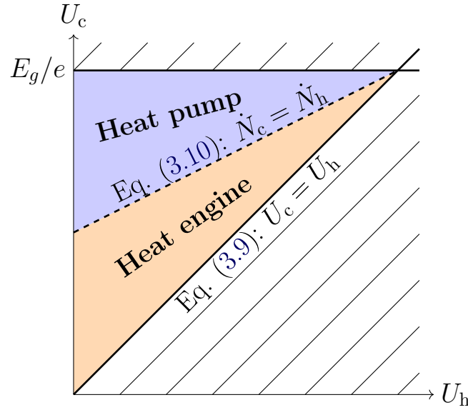
Figure 3.4: Equivalent Raveau diagram for TPX heat engines at the radiative limit ( QE = 1 ).
