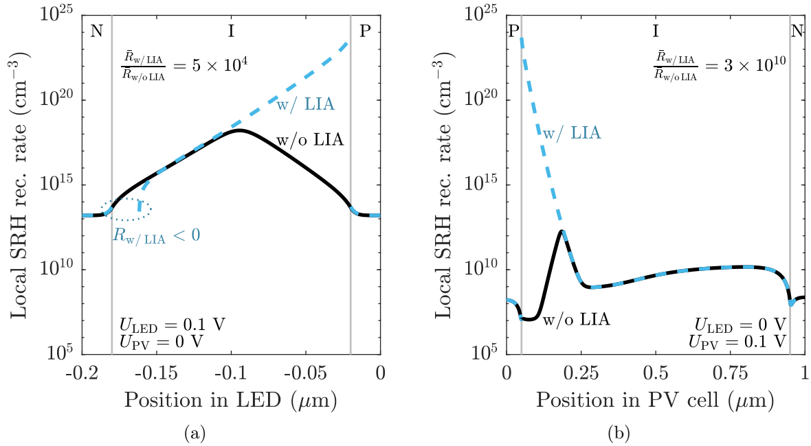
Figure 5.12: Effect of using the low-injection approximation to compute the local SRH recombination rate (a) in the LED, (b) in the PV cell at low voltage. The values of n and p used correspond to those obtained with the drift-diffusion solver, i.e. without the LIA.
