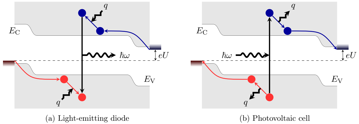
Figure 1.4: Basic principle of conversion in light-emitting diodes and photovoltaic cells. The two rectangles at the ends of the band diagram correspond to electrical contacts.
