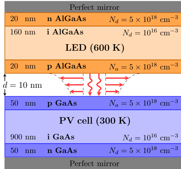
Figure 5.4: Schematic of the AlGaAs-GaAs homostructure under consideration, obtained from optimisation algorithms.
