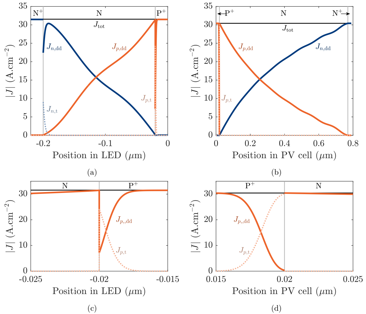
Figure 6.16: Spatially-resolved electron and hole current densities related to drift and diffusion (subscript dd ) or to tunnelling (subscript t ) at maximum power point (a) in the LED, (b) in the PV cell. Panels (c) and (d) correspond to a zoom of panels (a) and (b) around the interface where hole tunnelling occurs.
