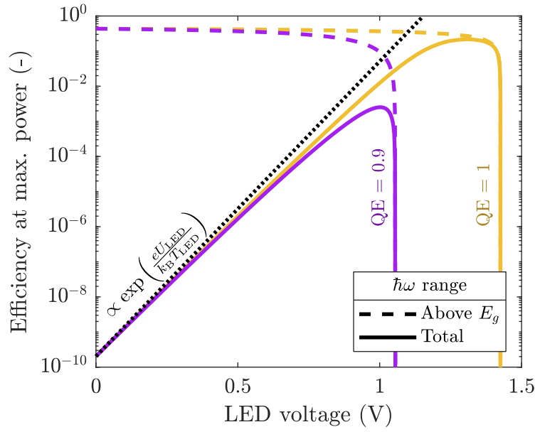
Figure 3.13: \eta -V characteristic of an AlGaAs NF-TPX device considering only above-bandgap photons or complete spectrum, for a 10 nm gap distance ( T_{\text{LED}} = 600 K, T_{\text{PV}} = 300 K).
