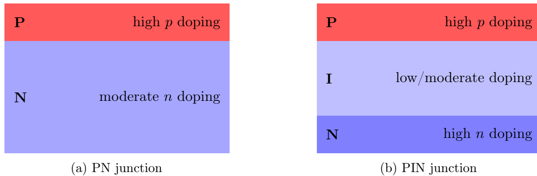
Figure 4.4: Basic semiconductor junctions.
