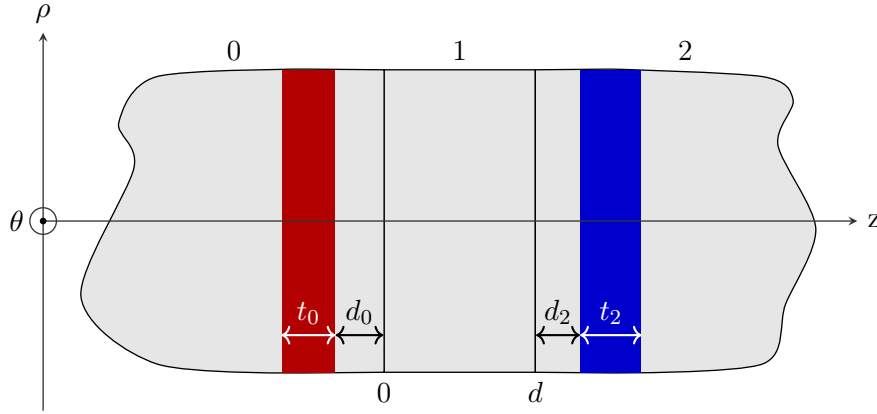
Figure A.2: Schematic of the system considered, the transmission coefficient being derived between the two coloured layers.
