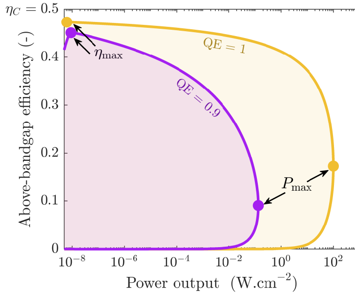
Figure 3.12: \eta - P characteristic of an AlGaAs NF-TPX device considering only above-bandgap photons, for a 10 nm gap distance ( T_{\text{LED}} = 600 K, T_{\text{PV}} = 300 K). The full line represents the convex envelope in which any point can be reached by setting the voltages properly.
