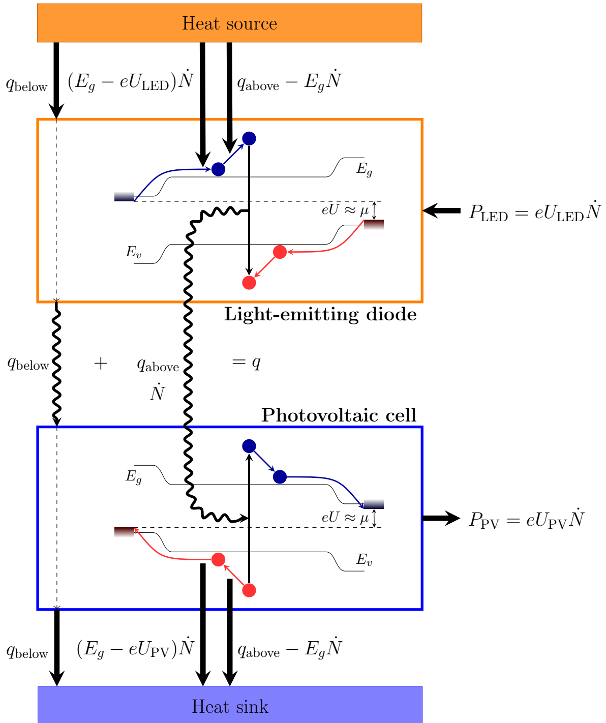
Figure 2.5: Schematic of the energy flow through a thermophotonic heat engine at the radiative limit.
