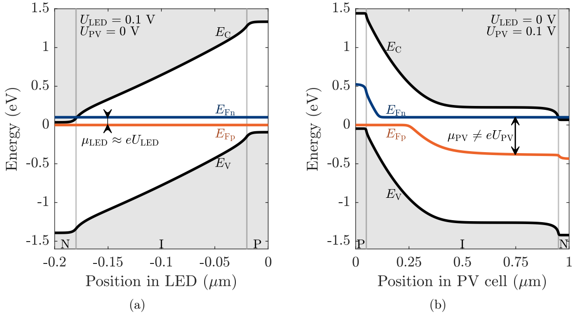
Figure 5.14: Band diagrams obtained (a) in the LED, (b) in the PV cell, with a voltage applied to the component under consideration equal to 0.1 V while the opposite component remains unbiased.
