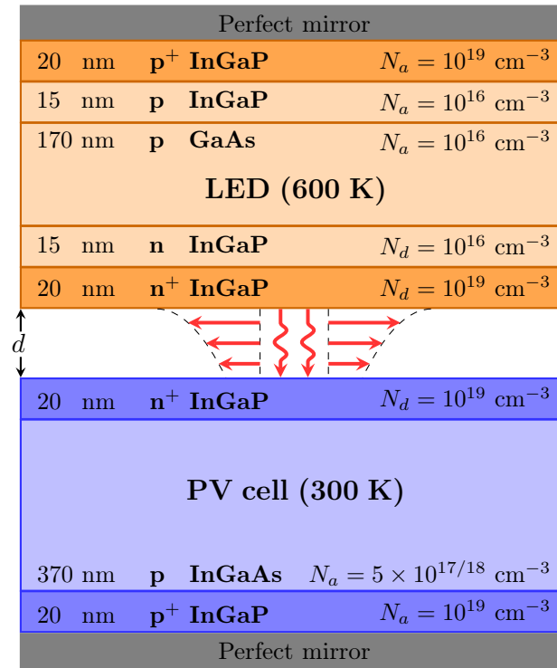
Figure 6.19: Proposed InGaAs/InGaP TPX structure for the reduction of non-radiative recombinations.
