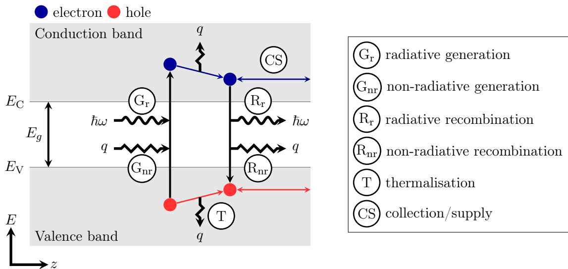
Figure 1.3: Main physical phenomena occurring in semiconductors.
