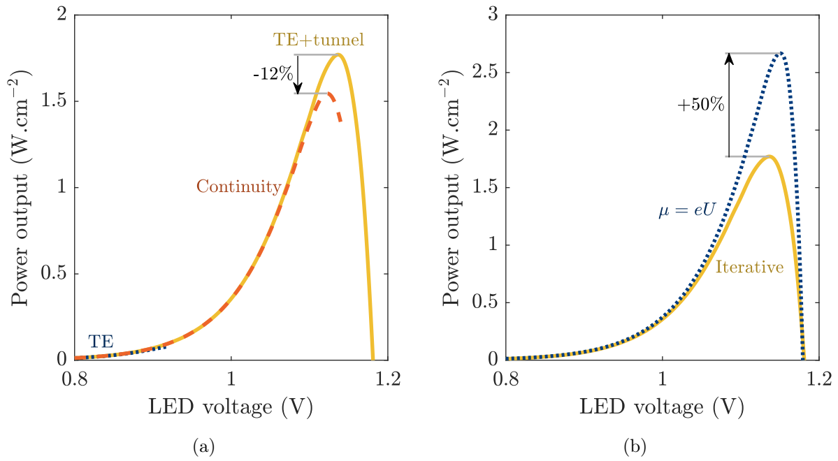
Figure 6.14: Influence of (a) the heterojunction model, (b) the iterative resolution of the photon chemical potential on the P - V_{LED} characteristic of the 10-nm-optimised TPX device.
