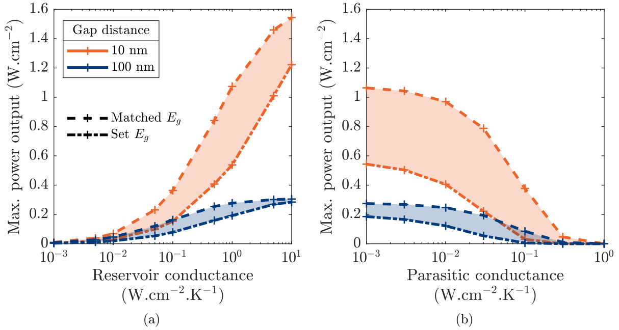
Figure 3.18: Impact of (a) reservoir and (b) parasitic thermal conductance on the performance of the NF-TPX device, with only above-bandgap photons considered.
