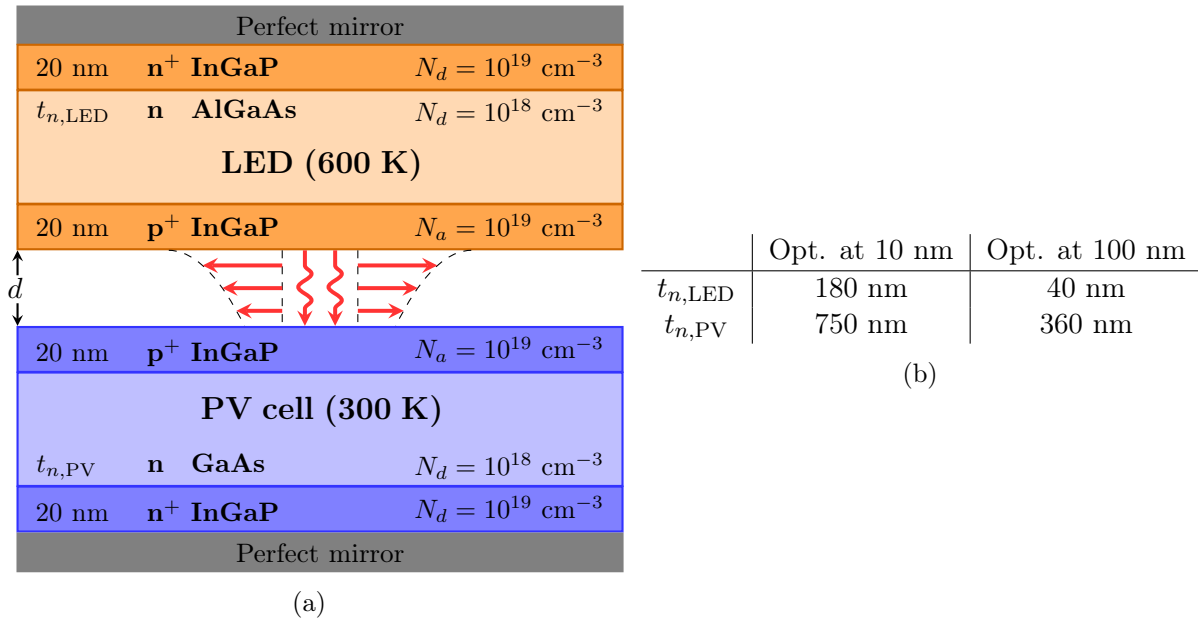
Figure 6.10: (a) Heterostructure-based AlGaAs/InGaP TPX device considered for optimisation. (b) Result of the active layer thickness optimisation.
