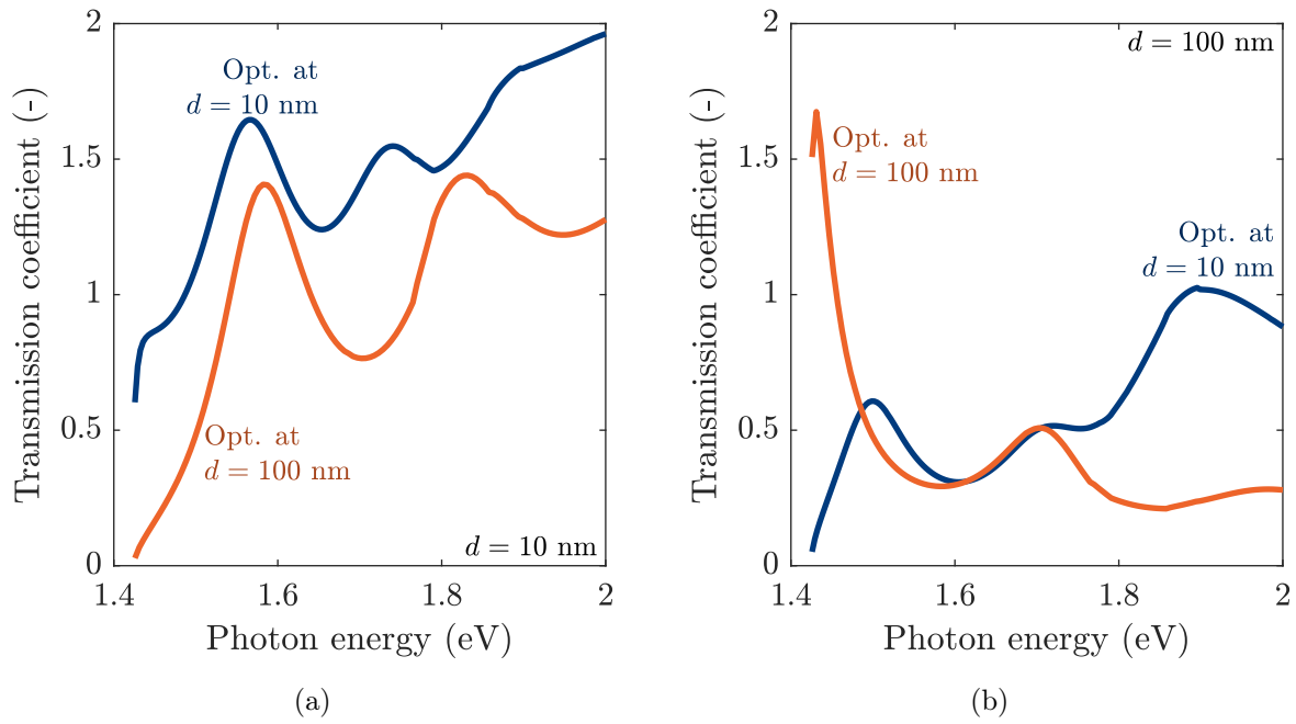
Figure 6.12: Transmission coefficient of radiation between the LED and the PV cell at normal incidence and for a gap distance of (a) 10 nm, (b) 100 nm. Since we consider unpolarised light, the transmission coefficient is equal to the sum of TM and TE transmission coefficients and is therefore bounded by 2.
