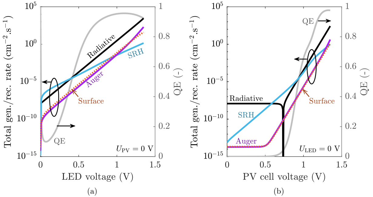
Figure 5.18: Total generation-recombination rate (a) in the LED, (b) in the PV cell, given as a function of the component voltage. The rates are given in absolute value.
