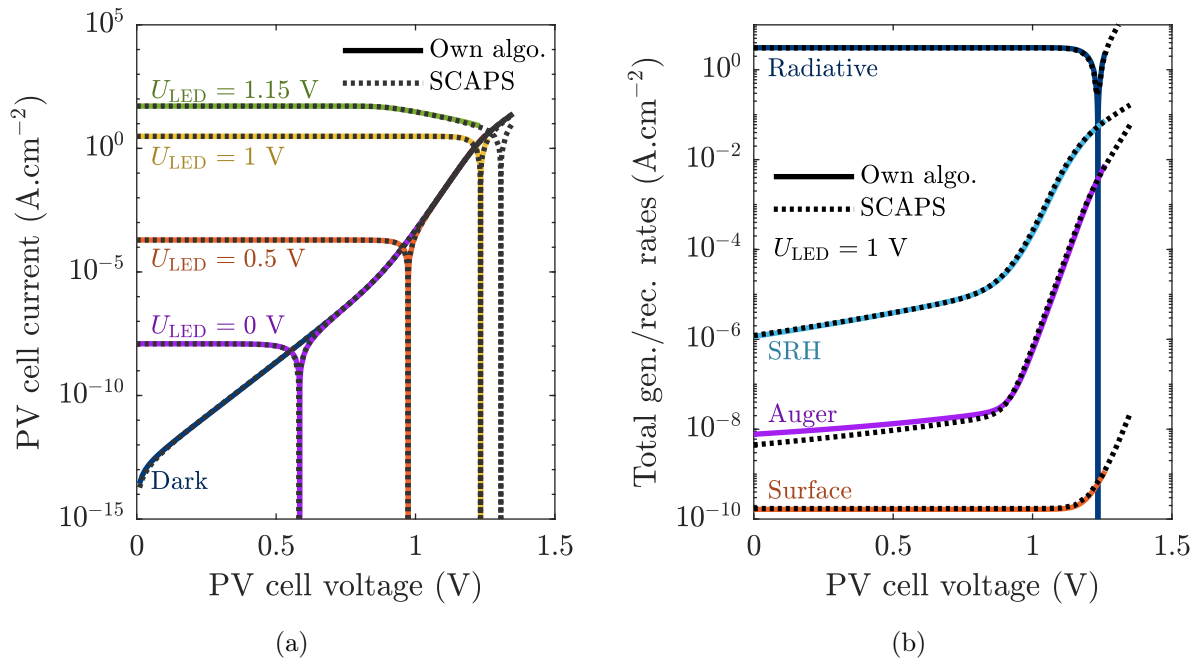
Figure 6.9: Comparison of the PV cell (a) I-V characteristic, (b) total generation-recombination rates obtained with the in-house algorithm and SCAPS considering the structure shown in Figure 6.8.
