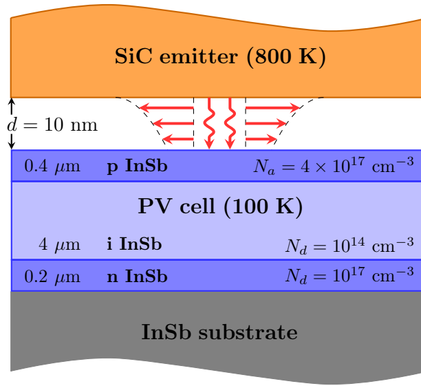
Figure 5.2: Structure used for the validation of the drift-diffusion solver.
