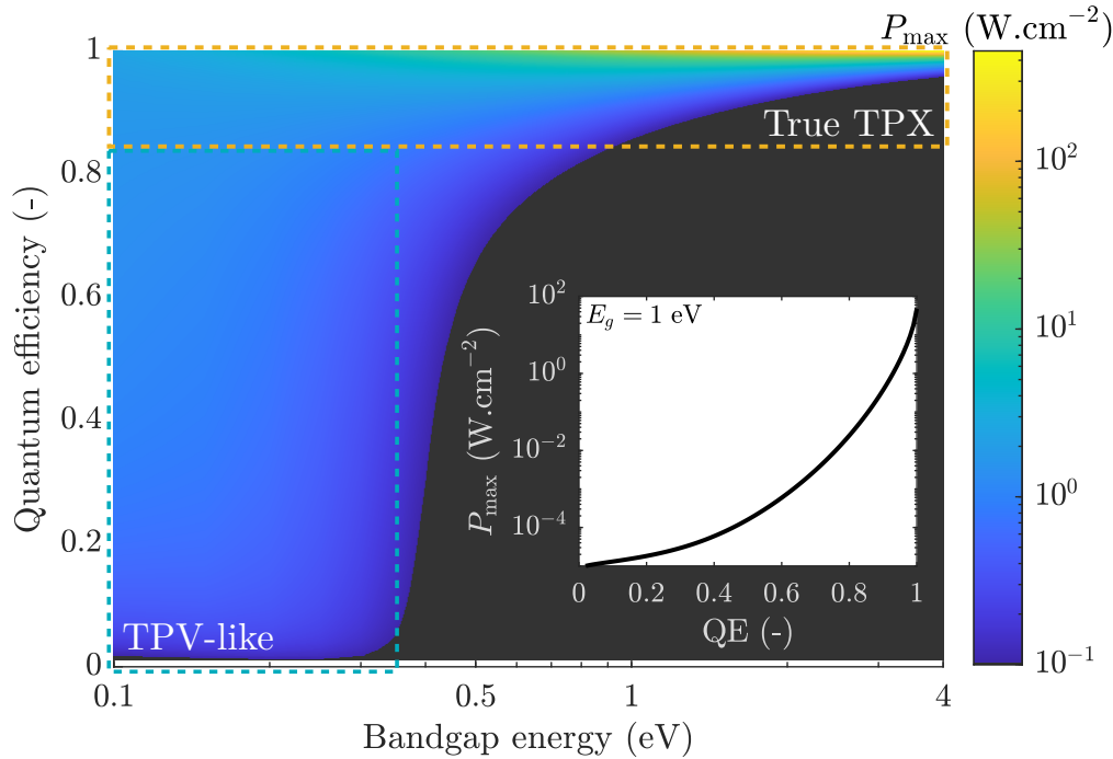
Figure 3.1: Maximum power production of NF-TPX devices with constant interband dielectric function 10 + 1i , with respect to the bandgap and the quantum efficiency. The gap distance is set to 10 nm, the LED and PV cell temperatures to 600 K and 300 K respectively.
