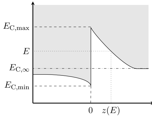
Figure 6.3: Representation of the different quantities useful for thermionic-field emission.
