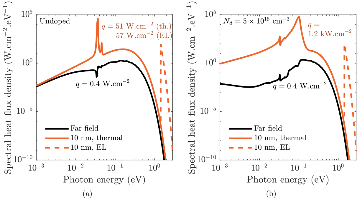
Figure 3.10: Spectral thermal heat flux density exchanged between the LED and the PV cell for different gap distances and for (a) undoped and (b) n-doped materials ( 5 \times 10^{18} \text{ cm}^{-3} ). For the electroluminescent (EL) case, the voltages obtained at maximum power point for \text{QE} = 0.9 are taken. In panel (a), the value of the thermal (th.) heat flux density is also provided.
