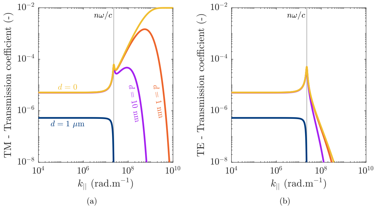
Figure 6.7: Transmission coefficient between two layers separated by a distance d obtained for \hbar\omega = 1.42 eV, in an infinite medium with dielectric function \varepsilon = 10 + i .
