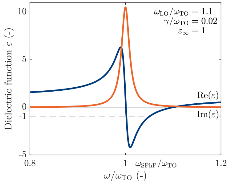
Figure 1.11: Typical dielectric function obtained with a Lorentz oscillator for the optical phonon contribution.
