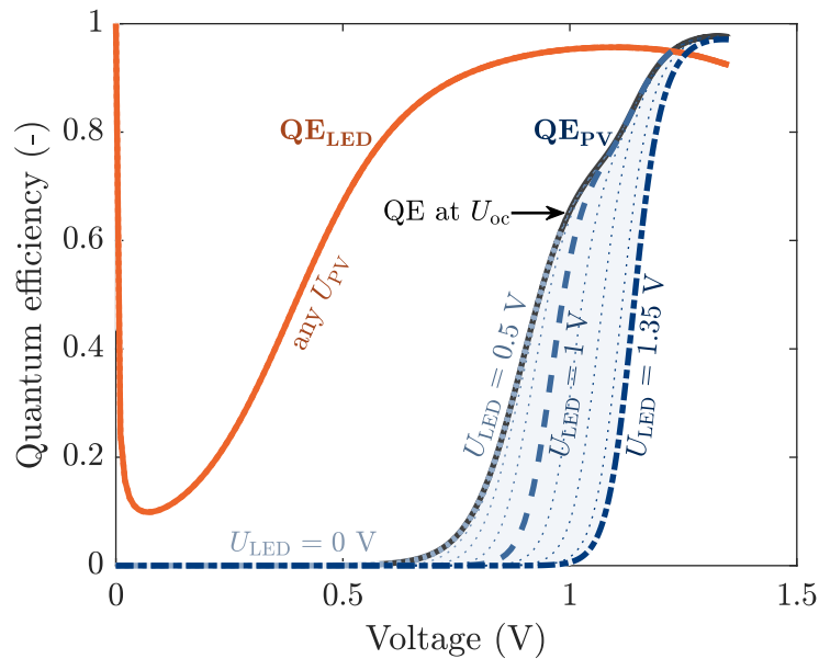
Figure 5.19: Variation of a component quantum efficiency as a function of its applied voltage, given in the voltage range in which the component behaves as expected (i.e. below U_{oc} for the PV cell and above U_{oc} for the LED). In the case of the PV cell, the QE profile varies with LED voltage and is therefore plotted every 0.1 V of U_{LED} . The value of the PV cell QE at U_{oc} is also represented in dark grey.
