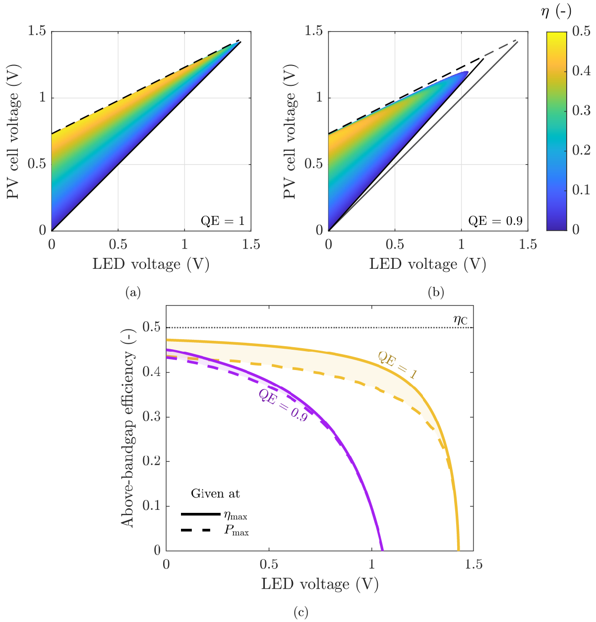
Figure 3.11: \eta -VV characteristic of an AlGaAs-GaAs NF-TPX device, for a 10 nm gap distance ( T_{LED} = 600 K, T_{PV} = 300 K), respectively for (a) QE = 1 , (b) QE = 0.9 . The full line corresponds to Eq. (3.9), the dashed line to Eq. (3.10a). (c) \eta -V characteristics of AlGaAs-GaAs NF-TPX devices. In all these figures, only above-bandgap photons are considered.
