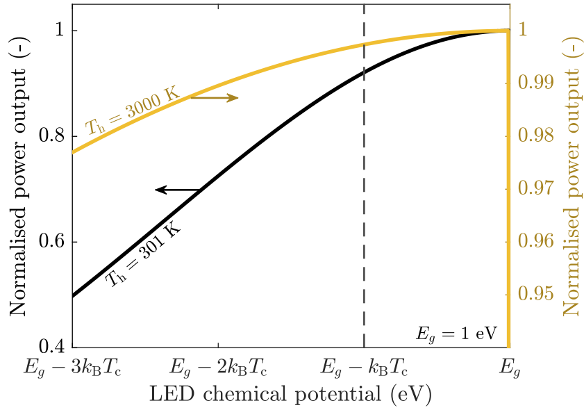
Figure 2.6: Variation of power output with LED chemical potential, for an LED temperature of 301 and 3000 K. Different scales are used for the two temperatures considered to improve readability.
