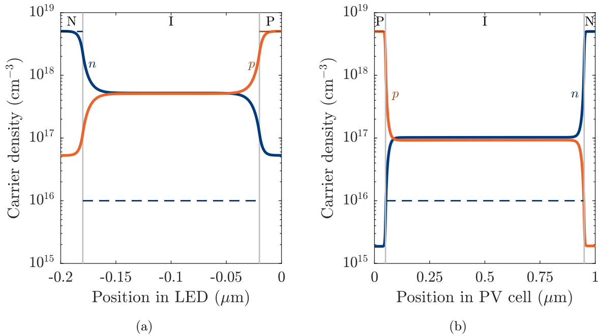
Figure 5.11: Charge carrier density at MPP (a) in the LED, (b) in the PV cell.
