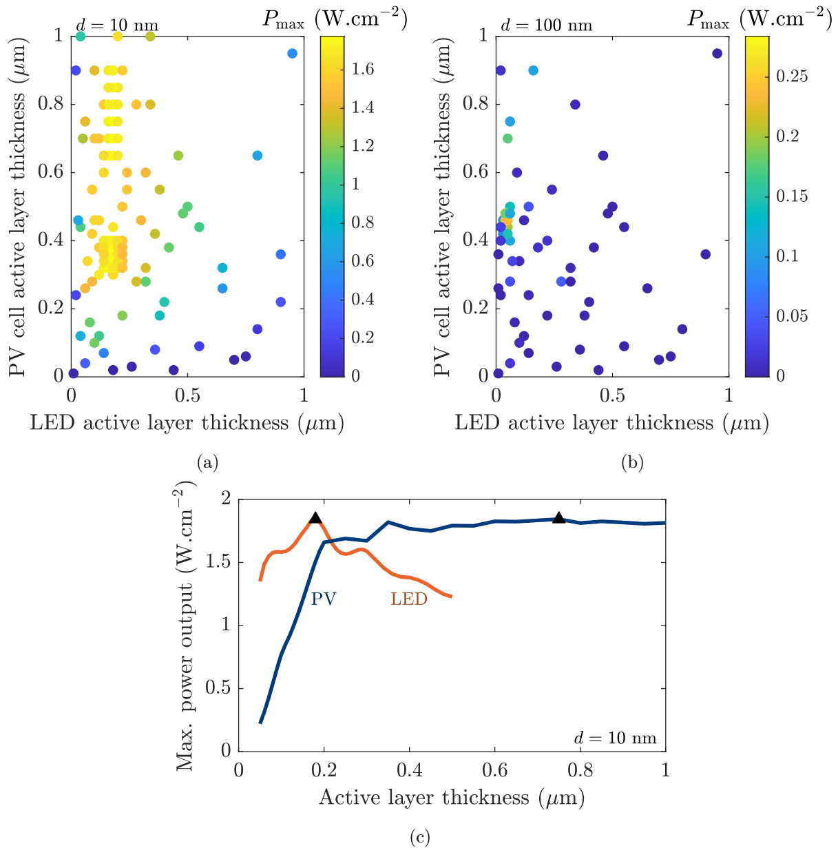
Figure 6.11: Power output estimate for different couples of active layer thicknesses, given by the optimisation process (a) at 10 nm, (b) at 100 nm. In (c) is given the variations of power output with active layer thicknesses at a 10 nm gap distance, around the optimum denoted by the markers.
