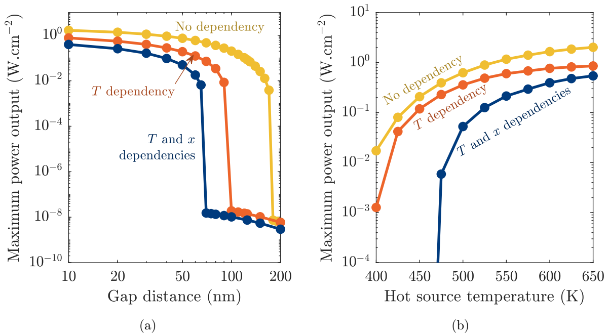
Figure 6.21: Influence of (a) the gap distance, (b) the heat source temperature on the maximum power output of the InGaAs/InGaP device. In the figures, x represent the indium fraction.
