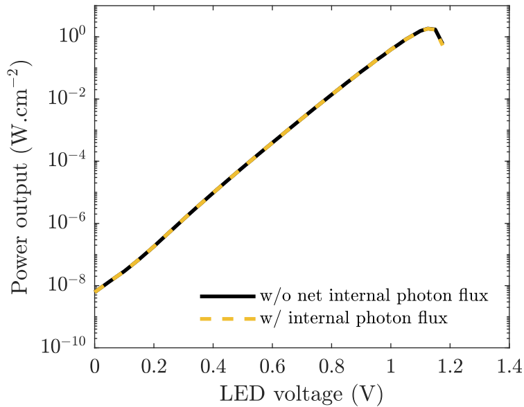
Figure F.2: P- V_{\text{LED}} characteristic of the AlGaAs/InGaP device represented in Figure 6.10a, either with or without the contribution of the photon flux internal to a component.
