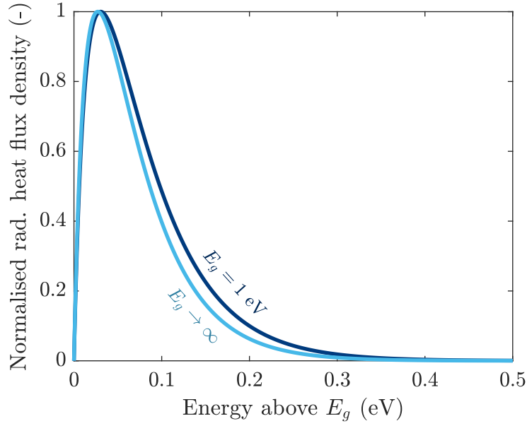
Figure 2.10: Spectrum of the radiative heat flux exchanged between the LED and the PV cell for (E_g - \mu)/k_B T = \ln(2) and for T_h = 600 K.
