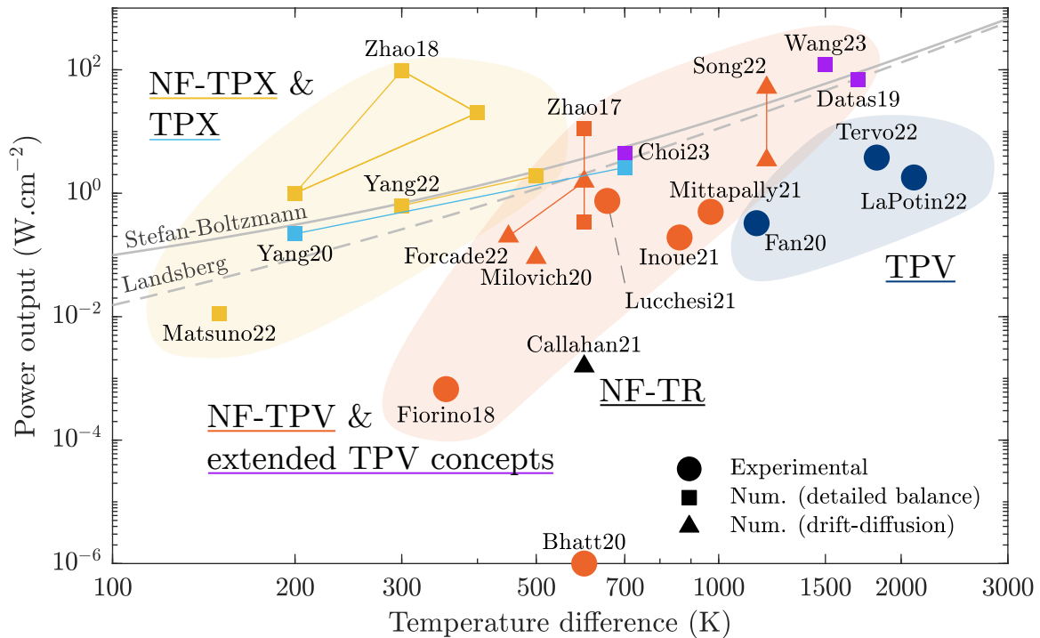
Figure 1.16: State-of-the-art of the performance of radiative heat engines. Connected points come from the same source. Stefan-Boltzmann law is expressed as \sigma(T_h^4 - T_c^4) , while Landsberg's limit corresponds to the power output P = \eta_L \sigma T_h^4 of a radiative engine receiving radiation from a blackbody and operating with Landsberg's efficiency (assuming a heat sink at ambient temperature).
