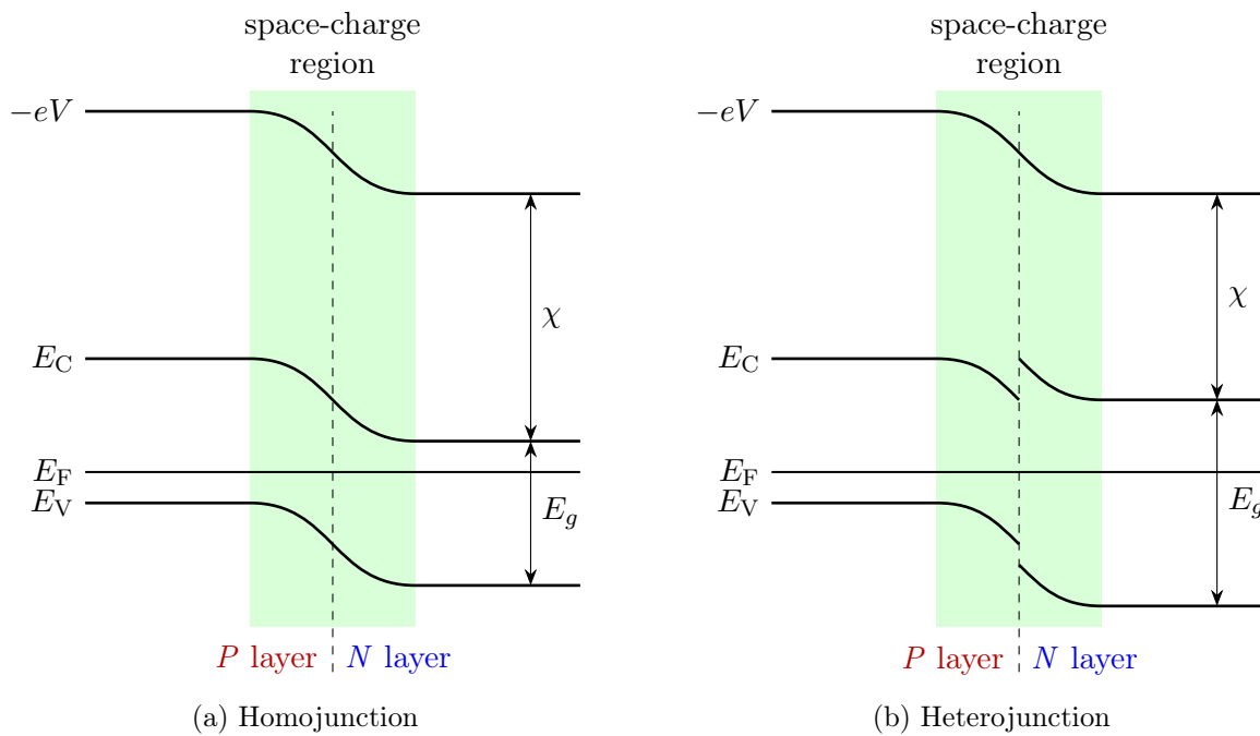
Figure 4.5: Band diagram for different abrupt junctions at equilibrium.
