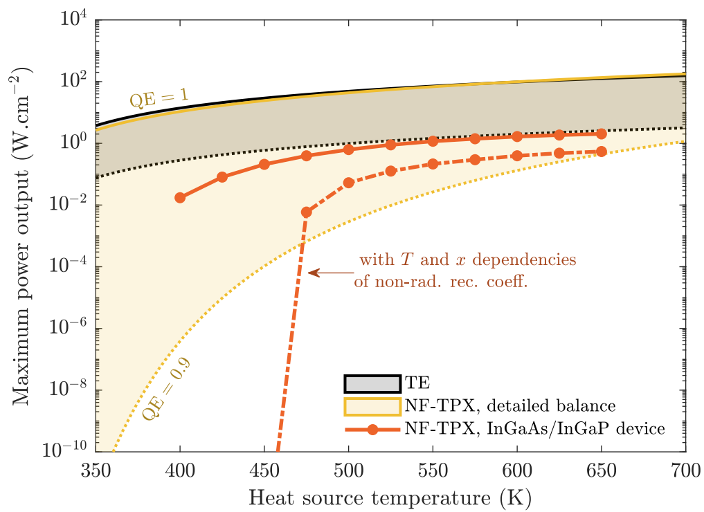
Figure 6.22: Performance of NF-TPX devices obtained from detailed balance (Chapter 3) and from the drift-diffusion modelling of charge transport in the InGaAs/InGaP device (Chapter 6), compared to thermoelectrics.
