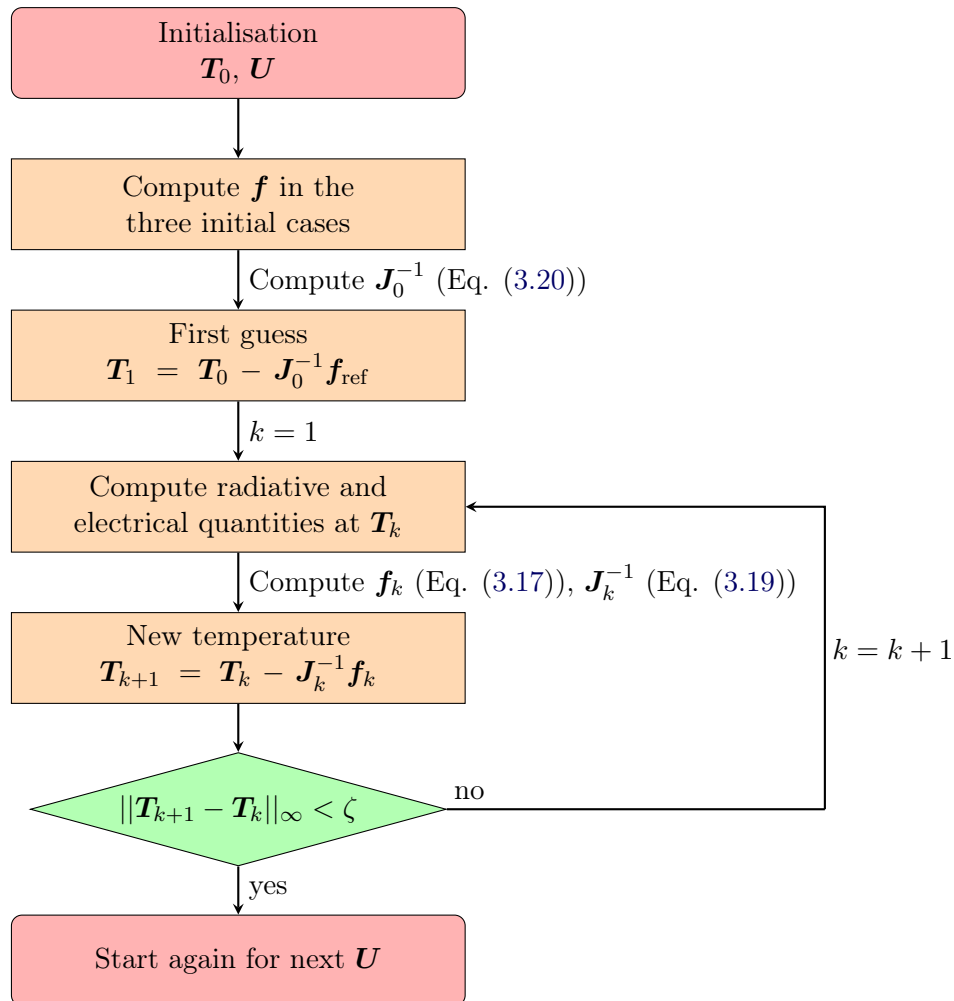
Figure 3.15: Flowchart of the Broyden's method based algorithm used to obtain the temperatures of both components at thermal equilibrium.
