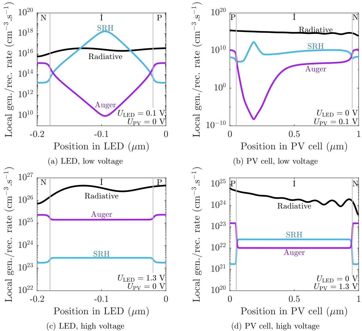
Figure 5.17: Local generation-recombination rates obtained at different voltages (a) in the LED, (b) in the PV cell. In all four panels, the rates are given in absolute value. Only for radiative events in the weakly biased PV cell is the generation rate greater than the recombination rate.
