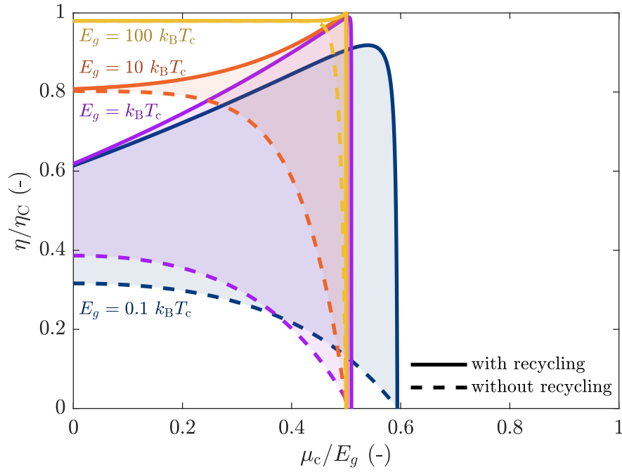
Figure 2.4: Variation of efficiency with chemical potential of radiation emitted by the cold absorber, obtained for T_h = 600 K and T_c = 300 K and for monochromatic radiation.
