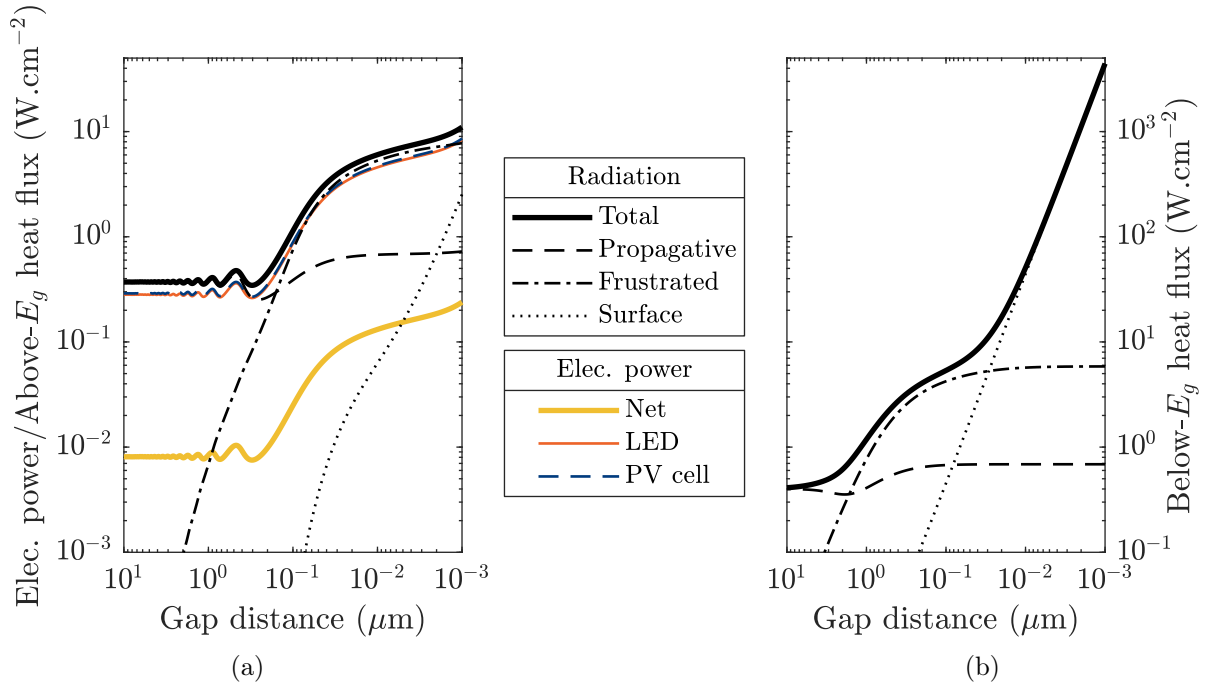
Figure 3.9: Influence of the gap distance on the different energy flows circulating through the device, at maximum power point and for a QE of 0.9. The different electrical powers and the above-bandgap heat transfer are provided in (a), while below-bandgap heat transfer is provided in (b).
