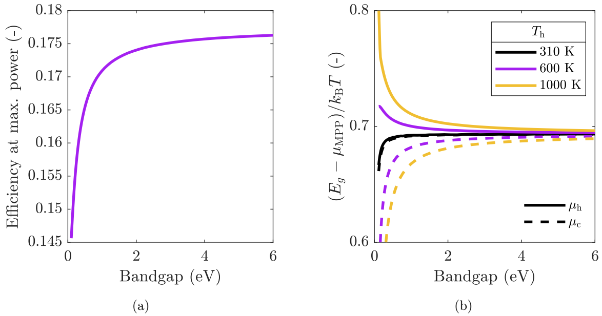
Figure 2.8: (a) Variation of efficiency at maximum power with bandgap for T_h = 600 K. (b) LED and PV cell chemical potentials at maximum power point given relatively to the bandgap and the energy k_B T (resp. k_B T_h and k_B T_c ) for various heat source temperatures.
