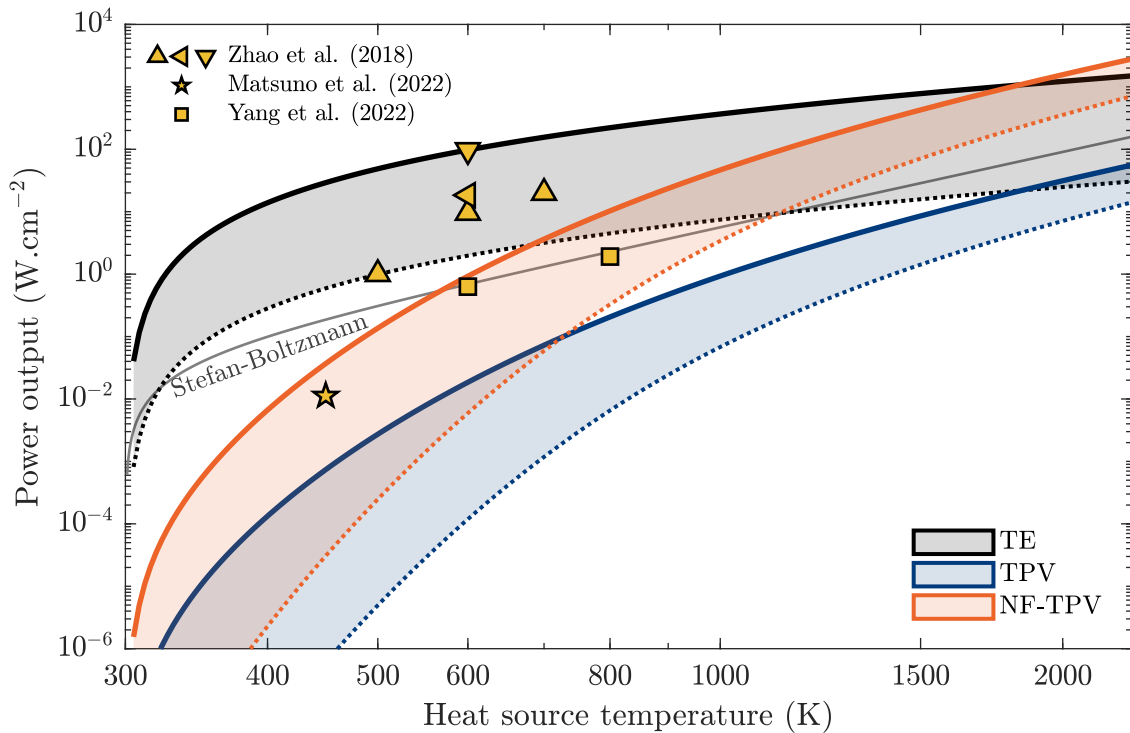
Figure 1.17: Basic models for the variation of power generated with heat source temperature, obtained for different radiative heat engines. Full and dashed line represent ideal and more realistic scenarios. For the data from [Zhao et al. 2018], several markers are used to denote the difference of hypothesis considered ( \nabla : ideal case, \triangleleft : with non-radiative recombinations, \triangle : with non-radiative recombinations and imperfect back mirrors).
