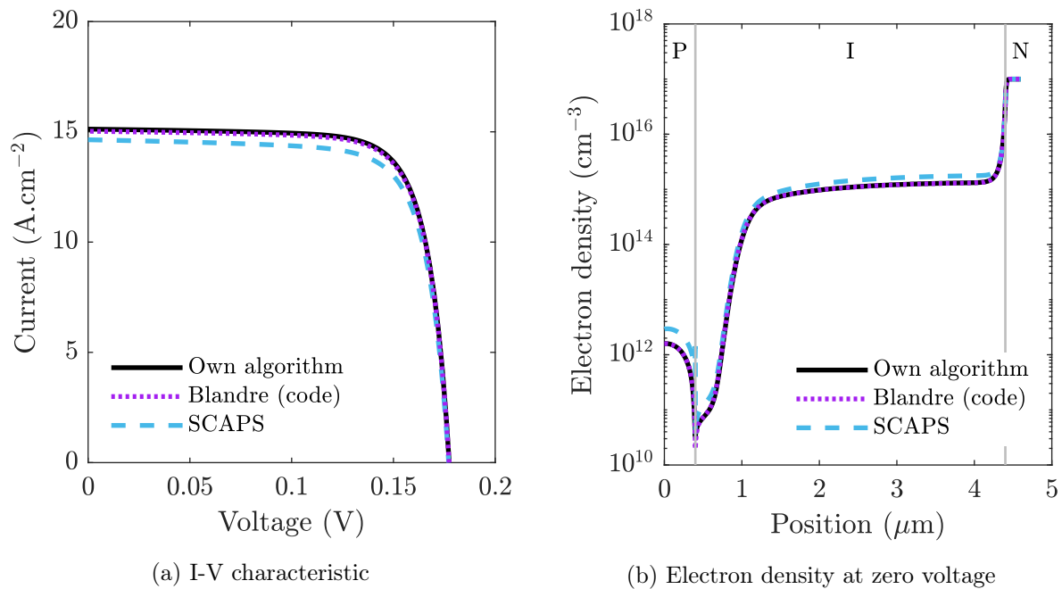
Figure 5.3: Comparison of the results obtained by different 1D drift-diffusion solvers for the reference device shown in Figure 5.2.
