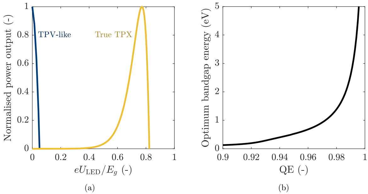
Figure 3.2: (a) Variation of the power output with respect to the LED voltage, for TPV-like (QE = 0.1, E_g = 0.2 eV) and true TPX (QE = 0.95, E_g = 1 eV) behaviour. For each LED voltage, the power output shown corresponds to the maximum obtained by varying the PV cell voltage. In both cases, power output is normalised by the maximum power. (b) Bandgap energy leading to maximum power output, computed for high quantum efficiencies.
