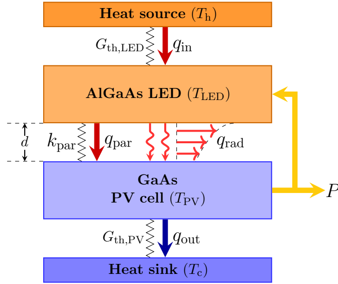
Figure 3.14: Schematic of the AlGaAs-GaAs device considered, with exo-irreversibilities taken into account.
