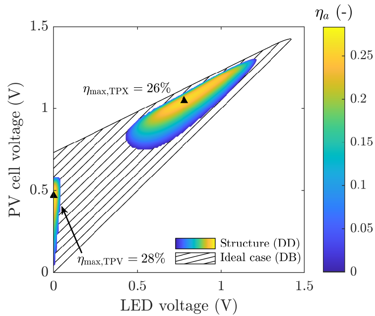
Figure 5.8: \eta -VV characteristic of the AlGaAs-GaAs homostructure.
