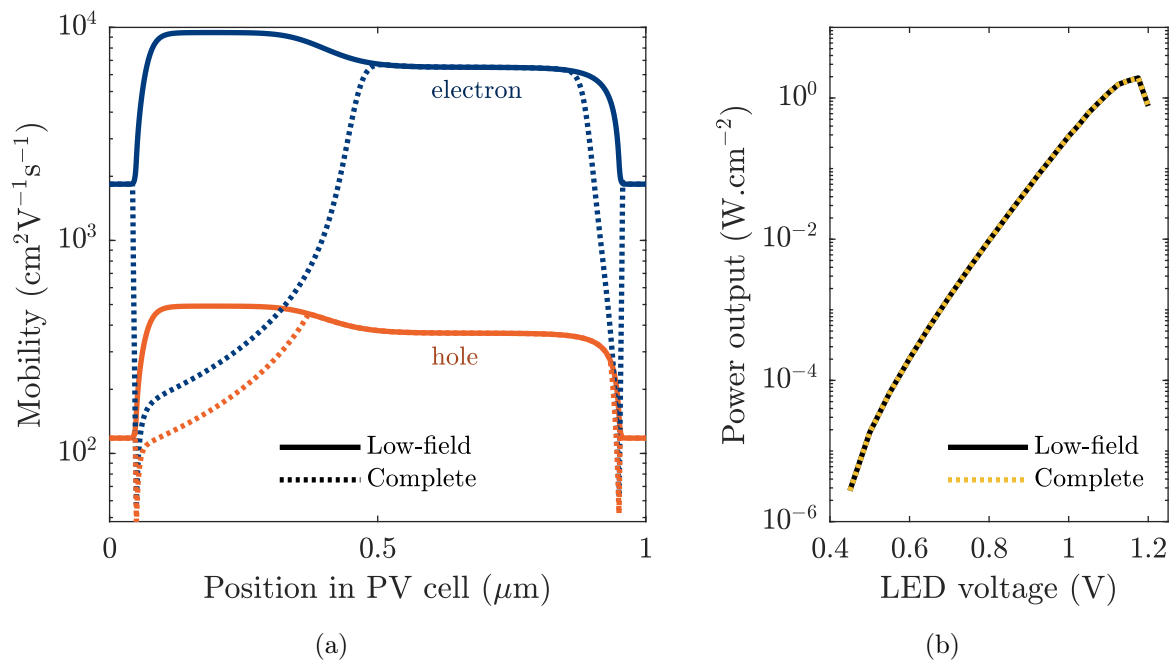
Figure F.1: Impact of using low-field or field-dependent mobility (a) on the value of mobility in the PV cell at equilibrium, (b) on the overall TPX performance. The device considered is provided in Figure 5.4.
