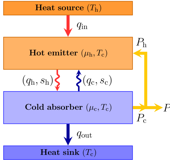
Figure 2.1: Representation of the luminescent heat engine.
