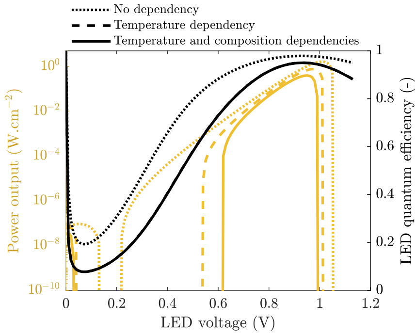
Figure 6.20: P - V_{LED} characteristic of the structure illustrated in Figure 6.19 for different scenarios, along with the LED QE at zero PV cell voltage.
