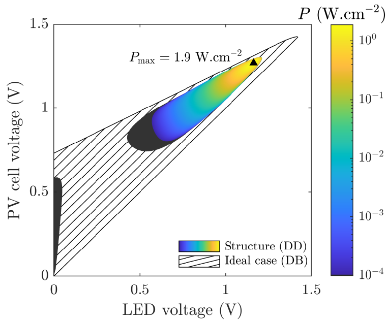
Figure 5.6: P-VV characteristic of the AlGaAs-GaAs homostructure.
