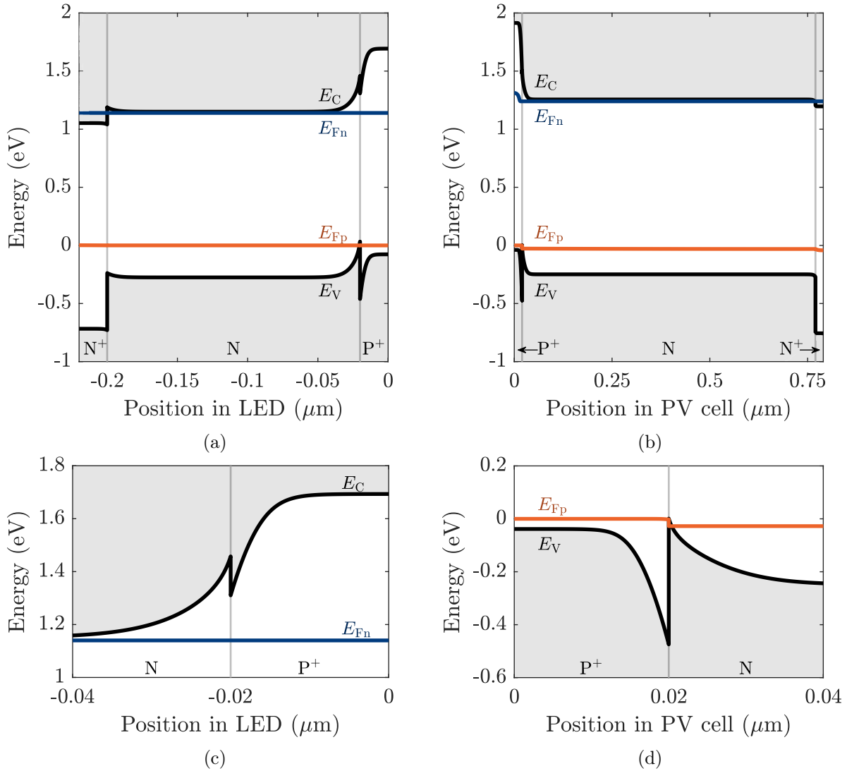
Figure 6.15: Band diagrams at maximum power point (a) in the LED, (b) in the PV cell. Panels (c) and (d) display a zoom of the band diagrams around the P^+ - N interface, respectively in the LED (for electrons) and the PV cell (for holes).
