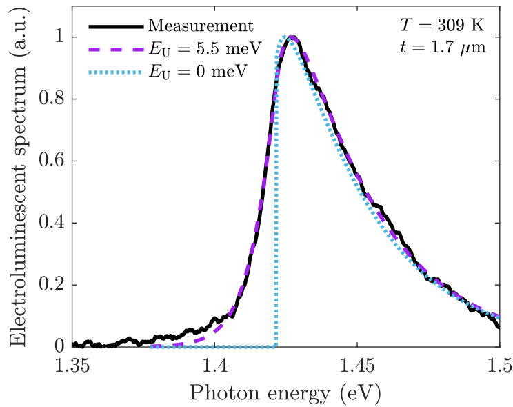
Figure 5.24: Comparison of the electroluminescent emission spectrum of an LED obtained from measurements and from Eq. (5.17).
