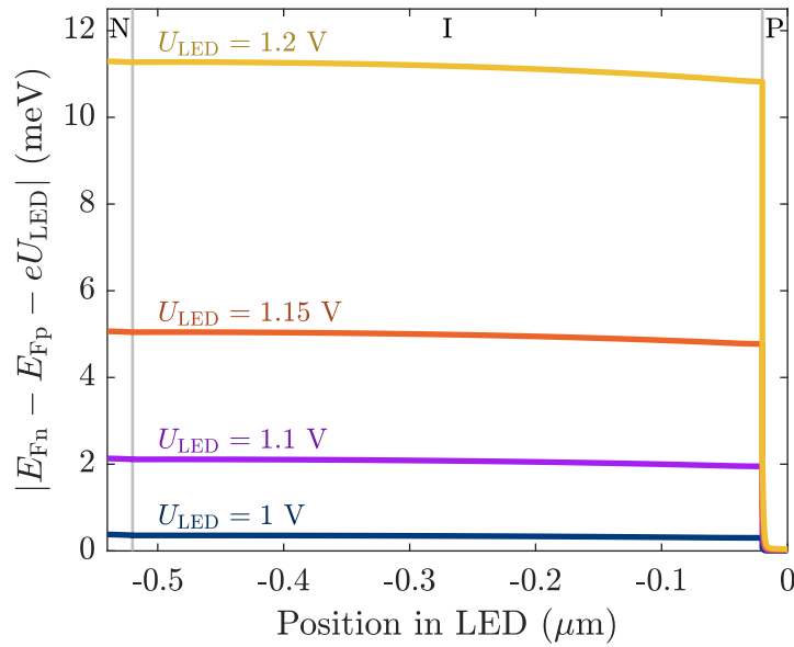
Figure 6.6: Typical deviation of the quasi Fermi level difference with respect to eU in a 600 K LED. It is obtained considering the TPX device shown in Figure 6.8 with an unbiased PV cell.
