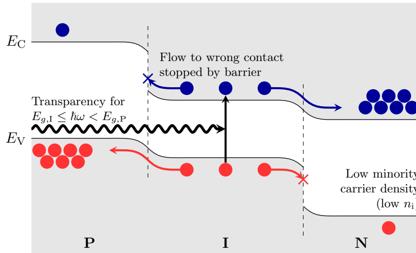
Figure 6.1: Advantages of heterostructures over homostructures.
