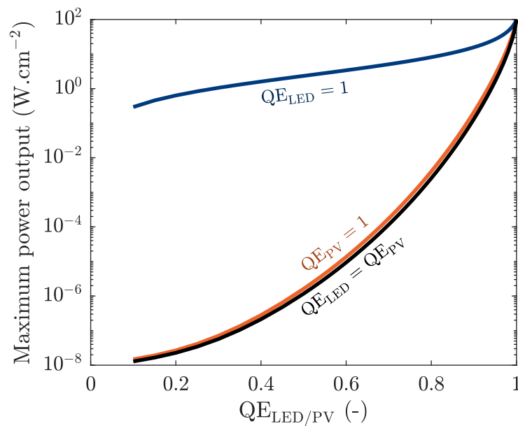
Figure 5.16: Variation of power output with quantum efficiency obtained with the detailed-balance model.
