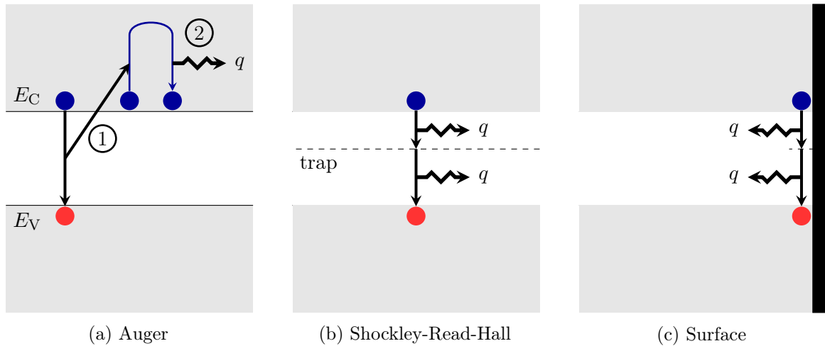
Figure 4.2: Schematics of the main types of non-radiative recombinations.
