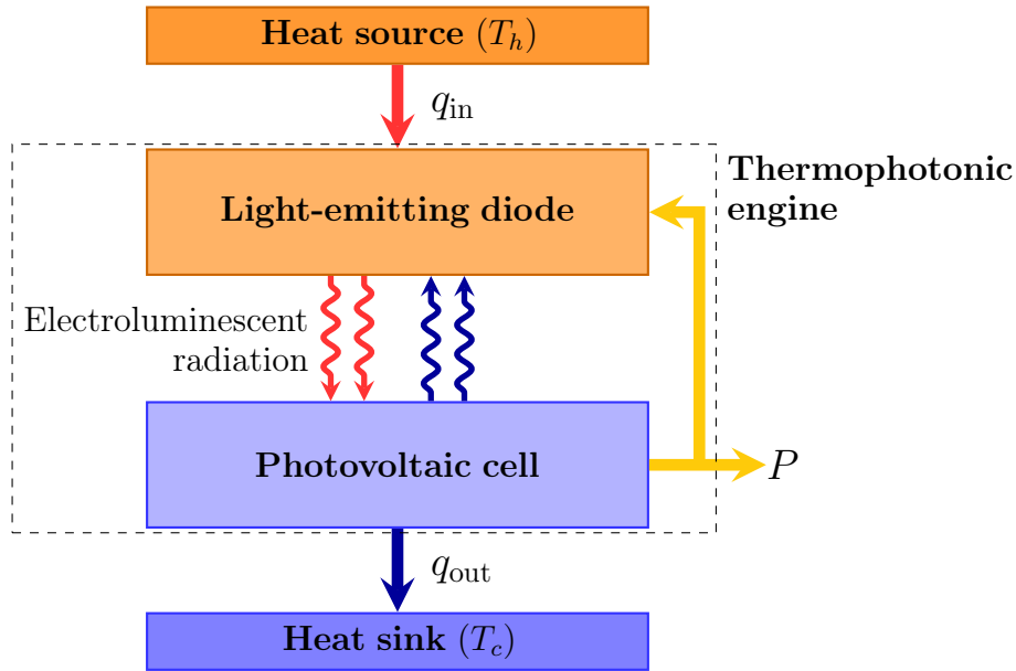
Figure 1.6: Representation of the thermophotonic heat engine.
