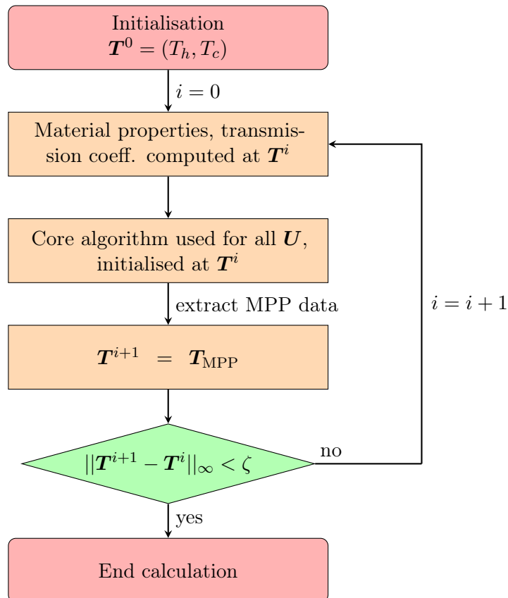
Figure 3.16: Flowchart of the secondary iterative process for self-consistent calculation of temperature and performance at maximum power point.
