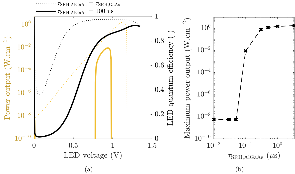
Figure 6.17: Influence of the SRH lifetime in AlGaAs (a) on the P-V LED TPX characteristic, (b) on the maximum power output.
