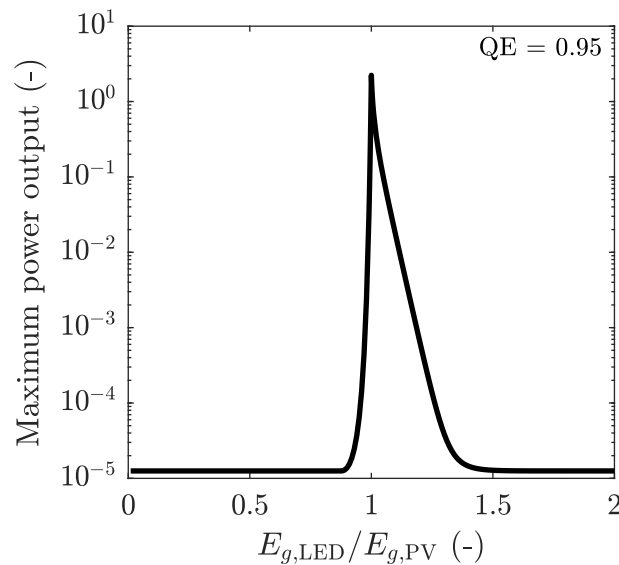
Figure 3.3: Variation of maximum power with the bandgap mismatch, for materials with dielectric function \varepsilon = 10 + 1i and for a PV cell bandgap of E_g = 1 eV.
