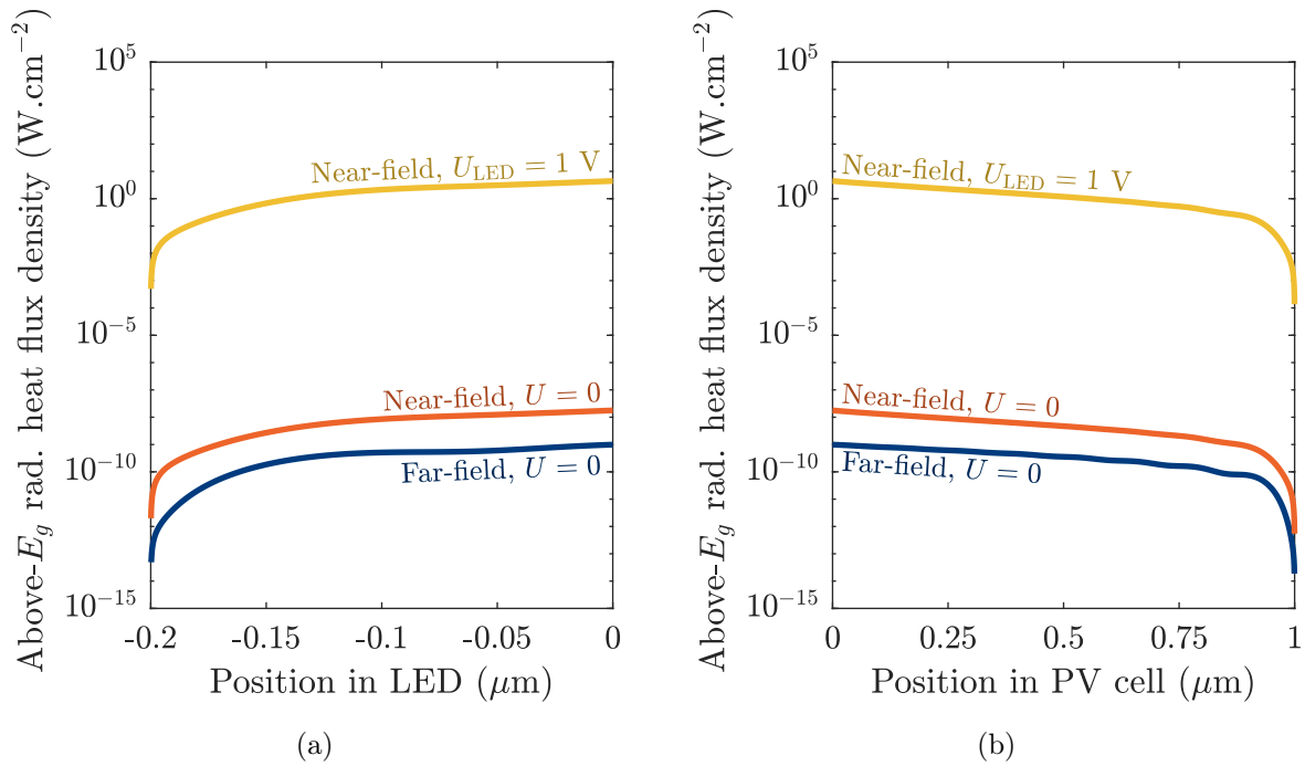
Figure 5.5: Local heat flux density (a) in the LED, (b) the PV cell obtained in the near field ( d = 10 \text{ nm} ) or in the far field. In all cases, the PV cell voltage is zero.
