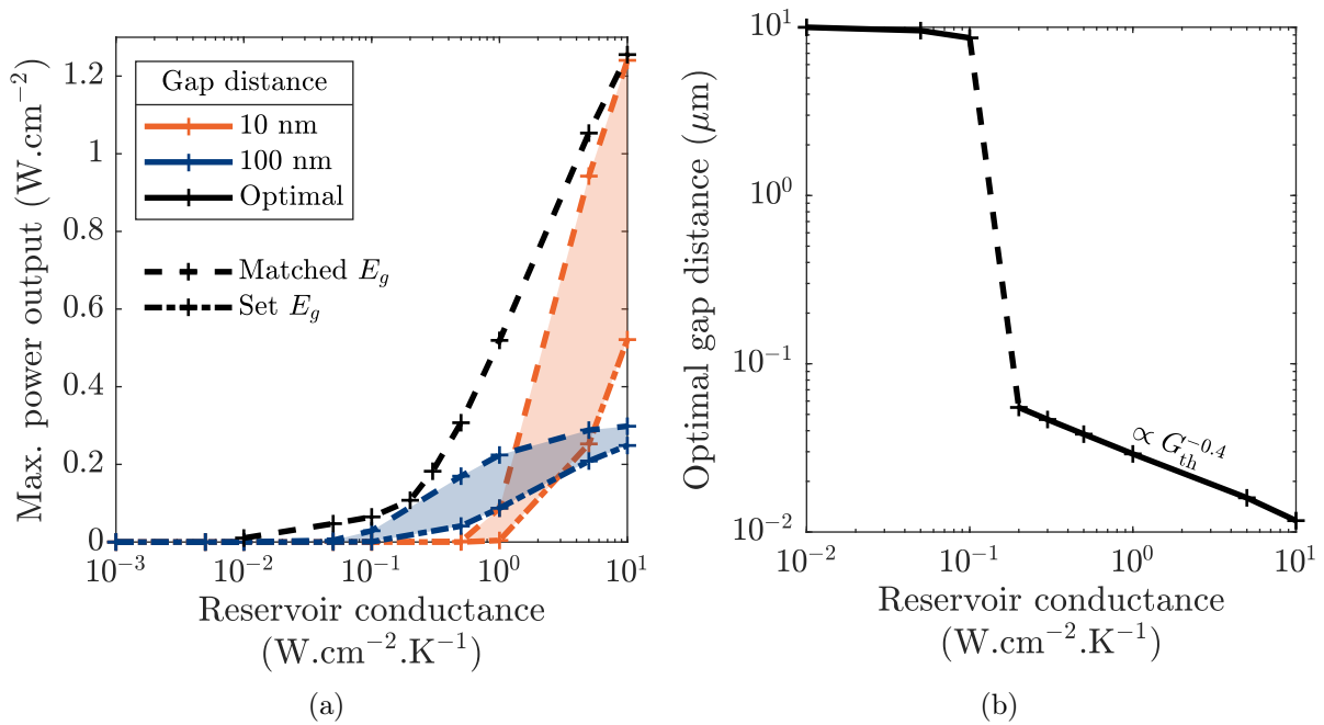
Figure 3.20: (a) Impact of reservoir conductance on the performance of the NF-TPX device, considering the complete spectrum. (b) Gap distance optimising the maximum power output as a function of the reservoir thermal conductance.
