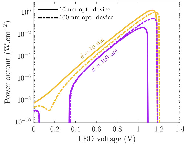
Figure 6.13: P - V_{\text{LED}} characteristic of the two optimised TPX devices, at 10 and 100 nm gap distance.
