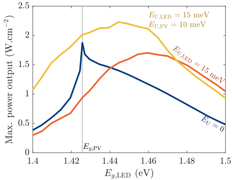
Figure 5.25: Variations of the maximum power output with the LED bandgap, controlled through the aluminium fraction.
