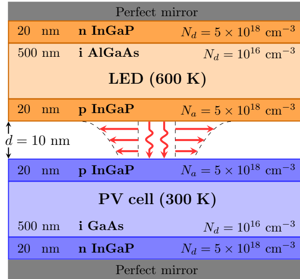
Figure 6.8: Non-optimised heterostructure-based TPX device used to compare the in-house solver with SCAPS.
