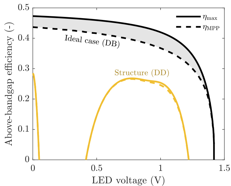
Figure 5.9: \eta - V_{LED} characteristic of the AlGaAs-GaAs homostructure.
