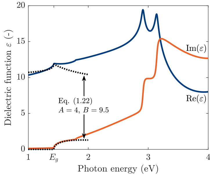
Figure 1.12: Dielectric function obtained for GaAs at room temperature with the model and parameters given in [Gonzalez-Cuevas et al. 2007].
