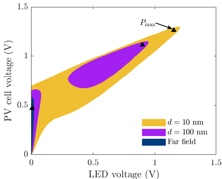
Figure 5.27: Power production region of a modified version of the structure shown in Figure 5.4, in which the doping level of intermediate layers is increased to 10^{18} \text{ W.cm}^{-3} .
