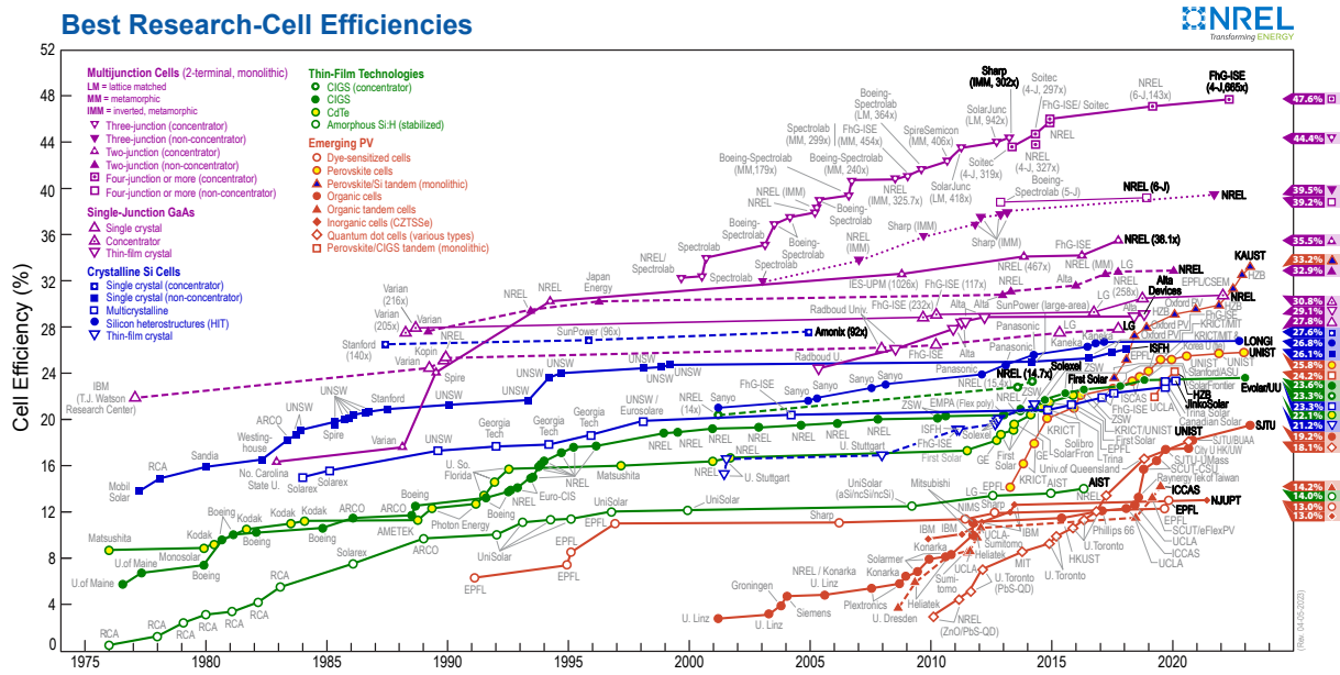
Figure 1.14: Best research-cell efficiency chart [NREL 2023].
