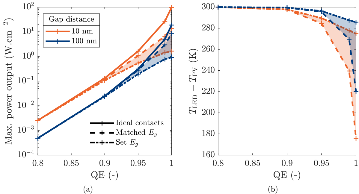
Figure 3.17: Impact of the QE on (a) the device performance, (b) the difference of temperature in the device for various reservoir thermal conductances, considering only above-bandgap photons.
