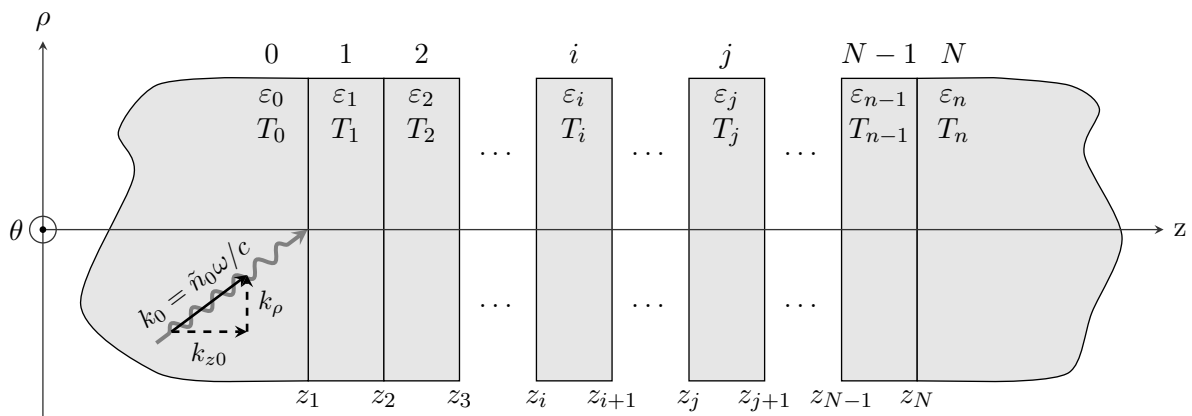
Figure 1.9: 1D multilayered structure considered in the simulation of near-field radiative heat transfer in the z direction. Schematic inspired by [Francoeur et al. 2009].
