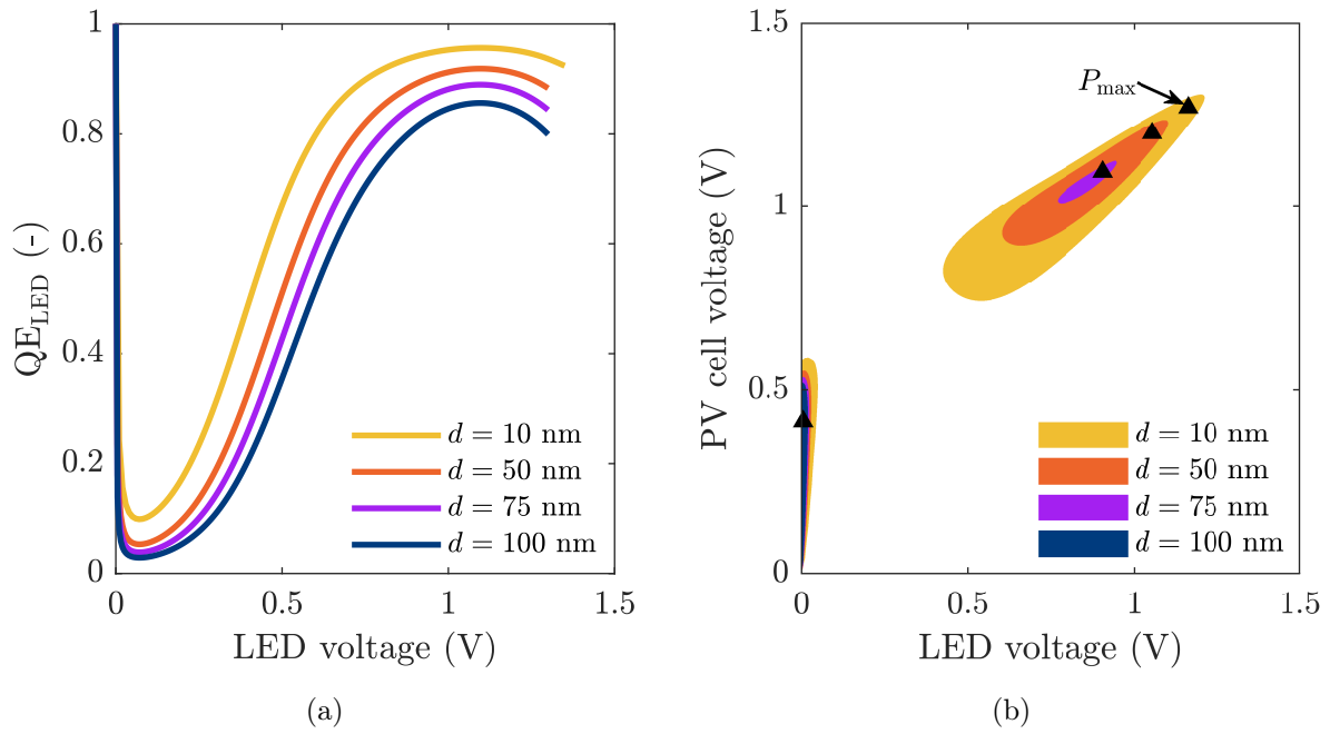
Figure 5.22: Impact of the gap distance (a) on the LED quantum efficiency, (b) on the TPX device power production region.
