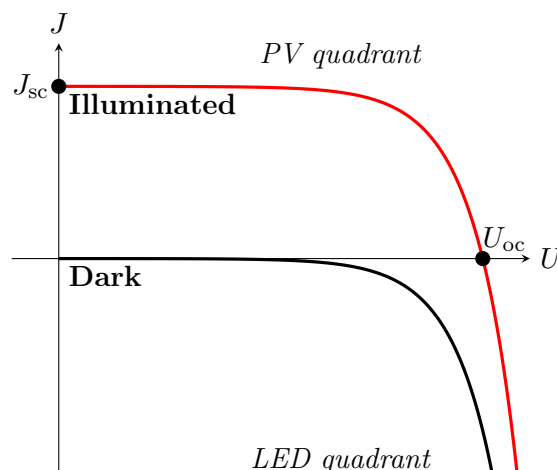
Figure 1.5: Current-voltage (I-V) characteristic of optoelectronic devices. In terms of sign convention, U \cdot J > 0 means that electrical power is produced.
