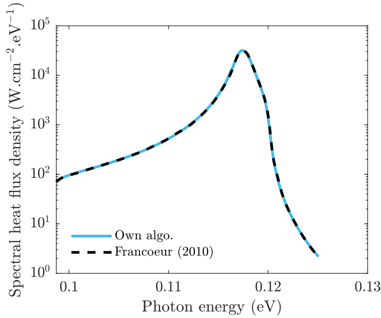
Figure A.1: Reproduction of the results provided in [Francoeur et al. 2010], obtained for slabs of thickness 10 nm and for a 10 nm gap distance.
