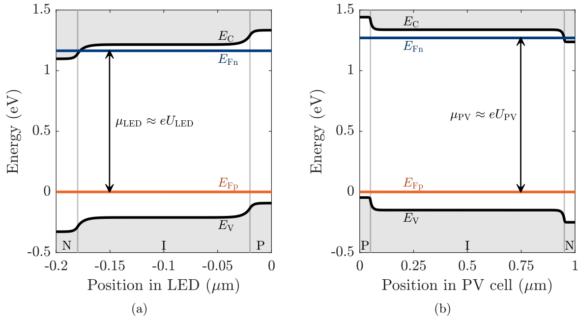
Figure 5.13: Band diagrams at MPP (a) in the LED, (b) in the PV cell.
