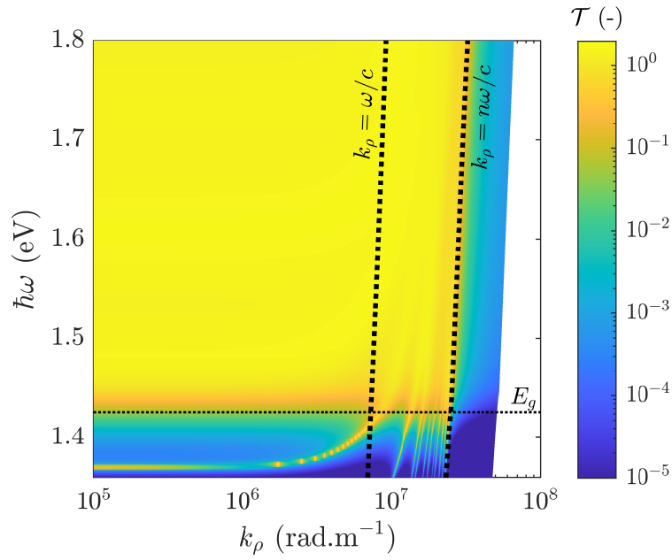
Figure 5.26: Transmission coefficient between the LED and the PV cell as a function of \omega and k_\rho .
