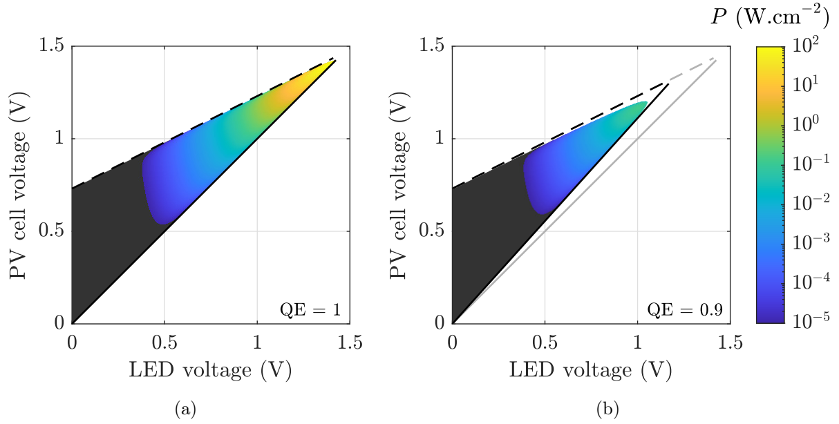
Figure 3.5: P-VV characteristic of an AlGaAs-GaAs NF-TPX device, for a 10 nm gap distance ( T_{\text{LED}} = 600 K, T_{\text{PV}} = 300 K), respectively for (a) \text{QE} = 1 , (b) \text{QE} = 0.9 . The full line corresponds to Eq. (3.9), the dashed line to Eq. (3.10a).
