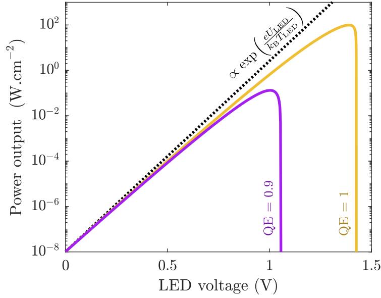
Figure 3.6: P- V_{LED} characteristic of an AlGaAs NF-TPX device.
