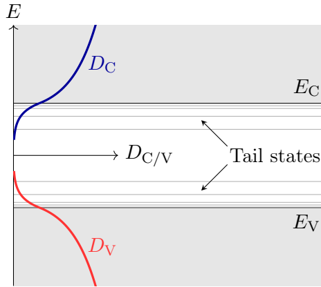
Figure 5.23: Schematic of the tail states inside the bandgap and the subsequent densities of states.
