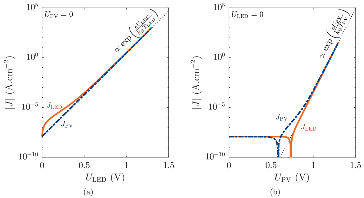
Figure 5.15: I-V characteristics of the LED and the PV cell, obtained by varying (a) U_{\text{LED}} , (b) U_{\text{PV}} .
