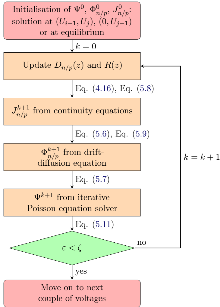
Figure 5.1: Flowchart of the drift-diffusion solver for homostructures at (U_{\text{LED}}, U_{\text{PV}}) = (U_i, U_j) .
