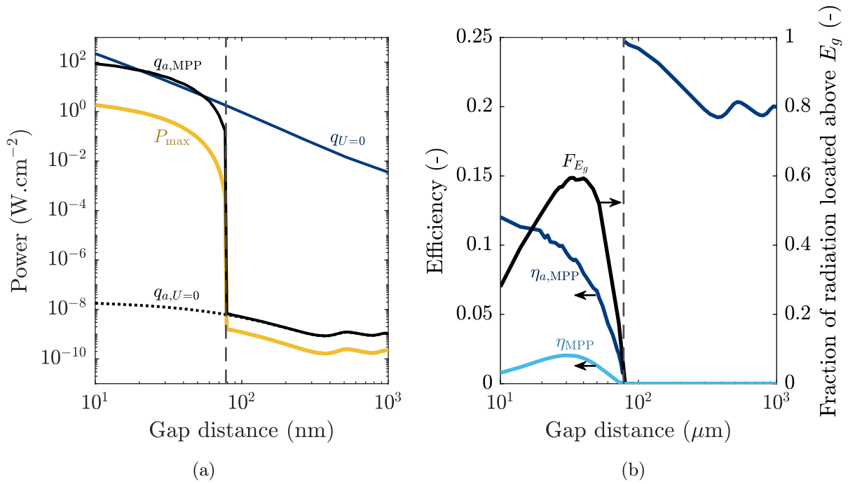
Figure 5.10: Impact of the gap distance on (a) the maximum power output and the transmitted radiative heat flux, (b) the efficiency of the AlGaAs-GaAs homostructure.
