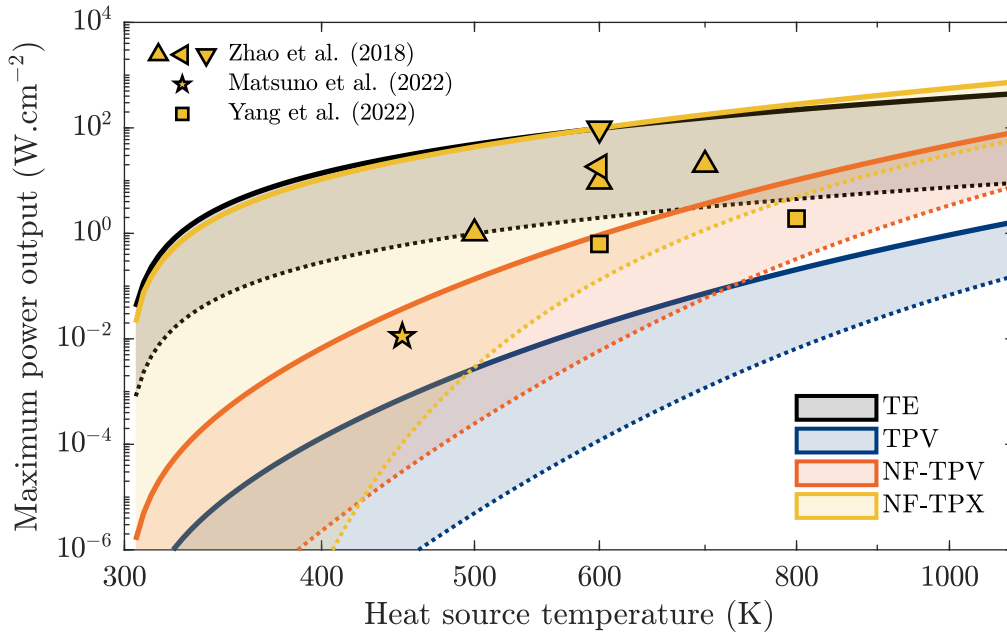
Figure 3.8: Variation of power output for different solid-state heat engines, as a function of the heat source temperature. Full and dashed lines represent ideal and more realistic scenarios (for NF-TPX, corresponding to the QE = 1 and QE = 0.9 cases).
