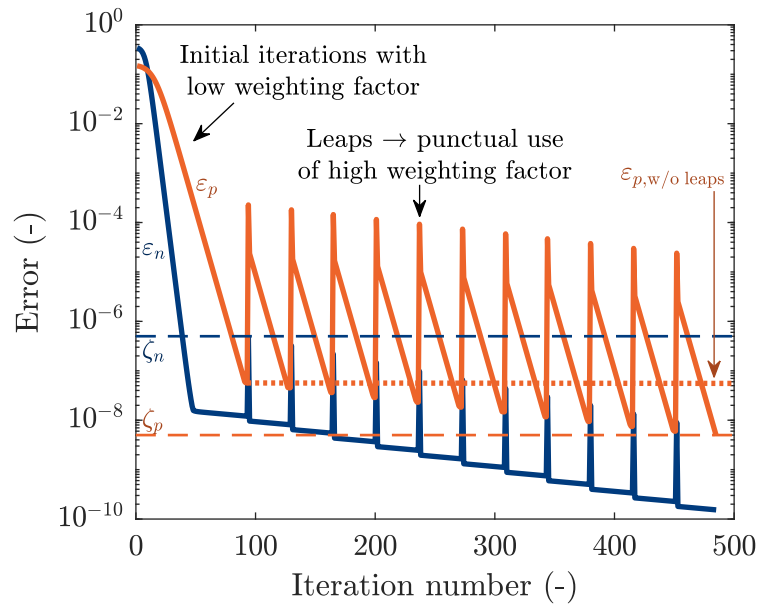
Figure 6.4: Typical variation of the error \varepsilon obtained at each iteration, defined as the relative variation of the Slotboom variables. \zeta denotes the tolerance.
