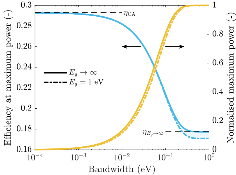
Figure 2.11: Variation of the maximum power output and the related efficiency with radiation bandwidth.
