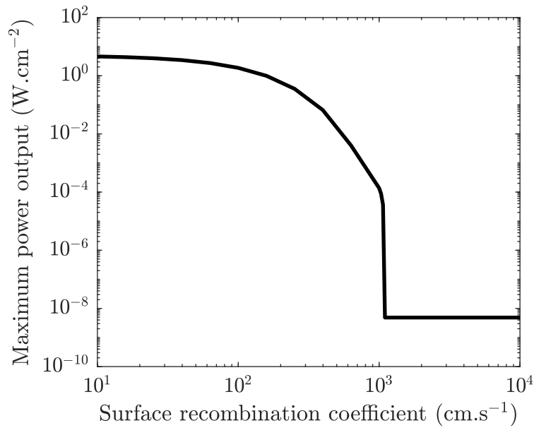
Figure 5.21: Impact of the surface recombination velocity on the maximum power output of the AlGaAs-GaAs homostructure.
