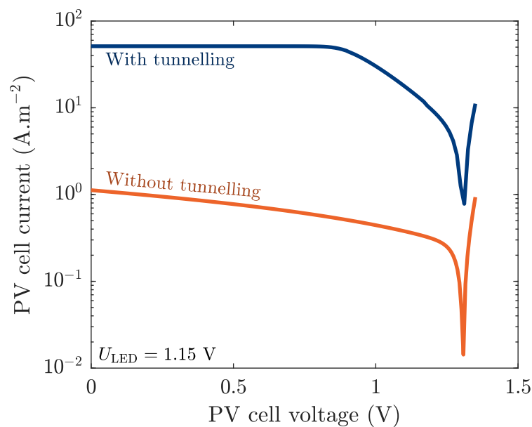
Figure F.3: I-V characteristic of the PV cell from Figure 5.2 with an LED voltage of 1.15 V.
