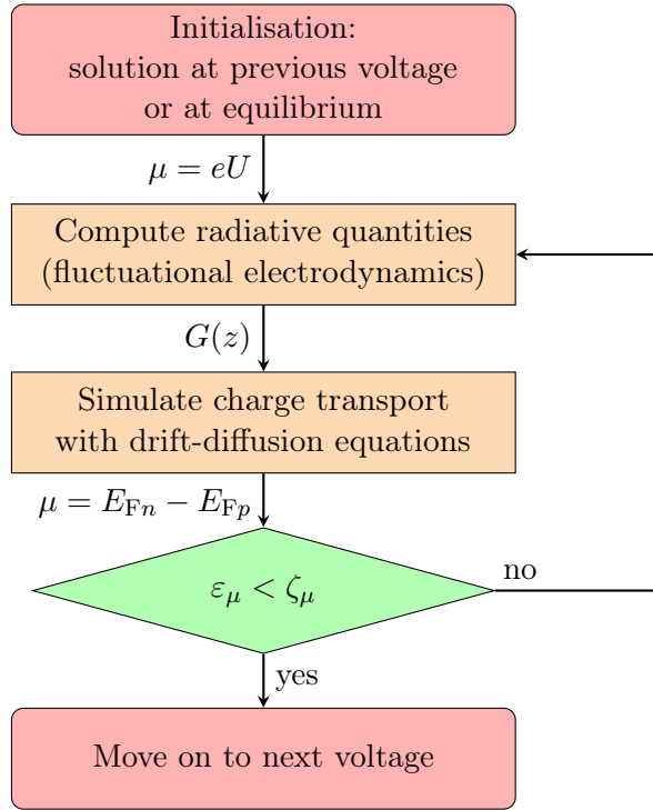
Figure 4.3: Flowchart of the coupled radiative-electrical iterative solver proposed in [Callahan et al. 2021].
