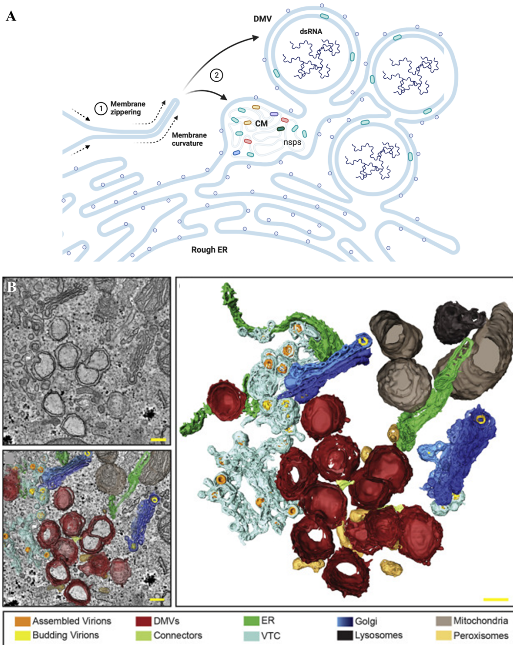
Fig. 16. Formation of DMVs during SARS-CoV-2 replication. A , Schematic of DMV or CM development during viral replication. Membrane zippering (1) is initiated by viral nsp causing membrane curvature. Subsequently, viral replication occurs in DMVs or CMs hiding the viral products from sensors in cell cytoplasm and concentrating components needed for replication. Panel A adapted from [259] and modified with biorender.com. B , Electron tomography and 3D reconstruction of viral replication sites in SARS-CoV-2-infected Calu-3 cells (MOI = 0.5) harvested 24 hours post infection (hpi). Panel B from [261]
