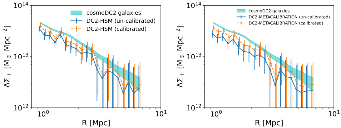
Figure 4.7: Left: stacked excess surface density profile around mass and redshift selected dark matter halos, first by using cosmoDC2 background galaxies (cyan), HSM un-calibrated (blue) and calibrated (orange) shapes. Right: stacked excess surface density profile using cosmoDC2 background galaxies (cyan), and using mCal un-calibrated shapes (blue) and by applying the shear self-calibration (orange).
